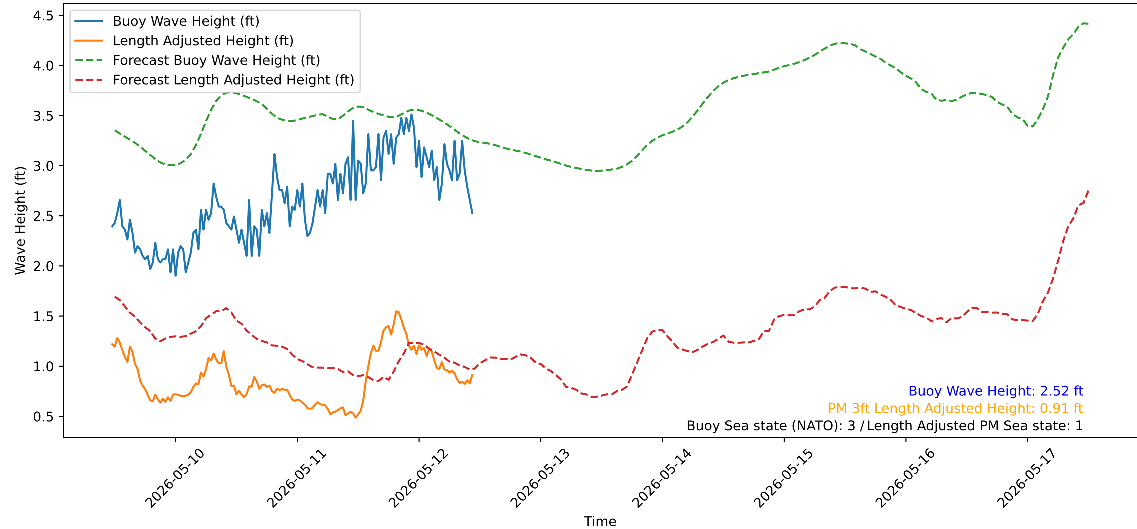
Wave Heights over Time for Green Beach at 2026-05-12 11:31:13
