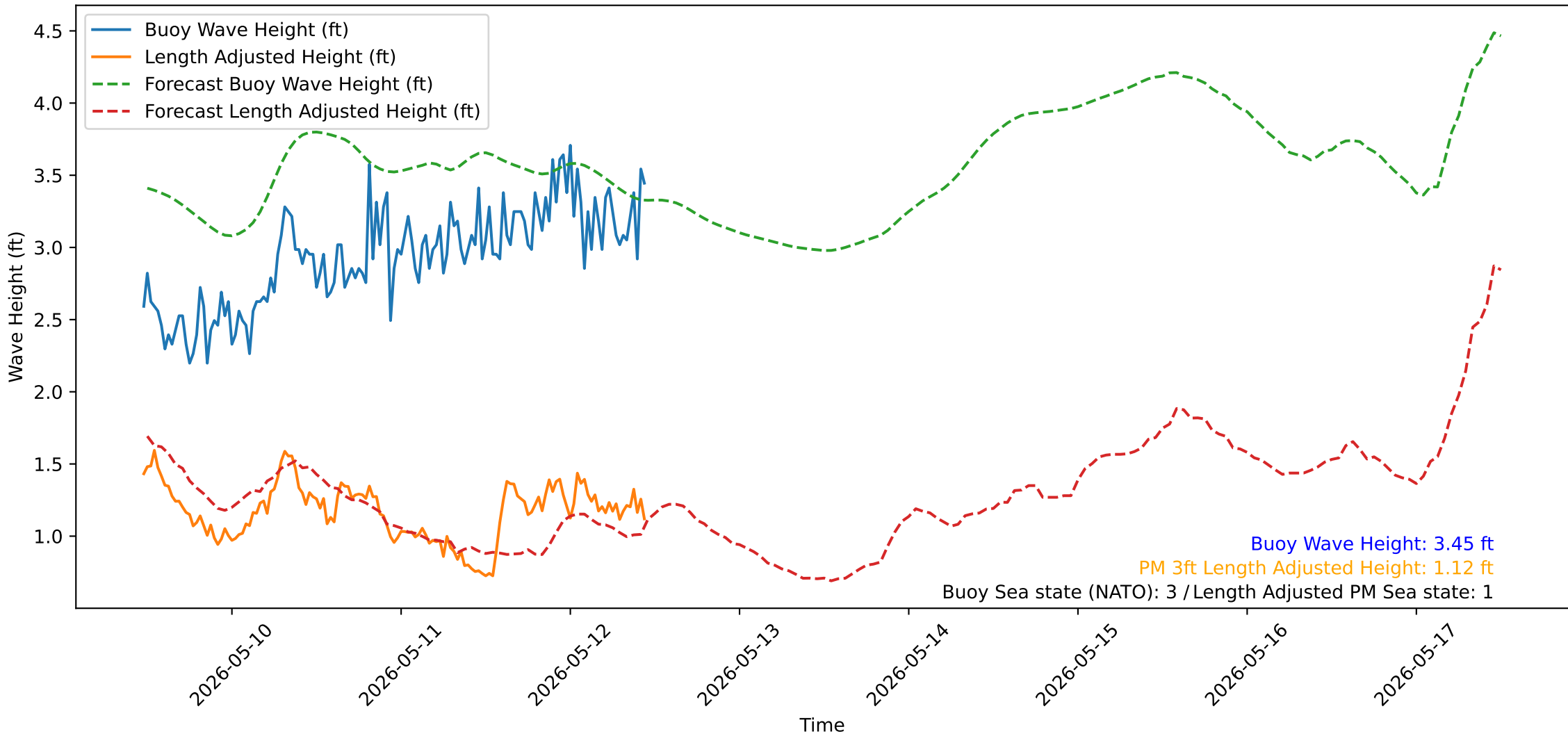
Wave Heights over Time for Oceanside Harbor at 2026-05-12 11:30:32
