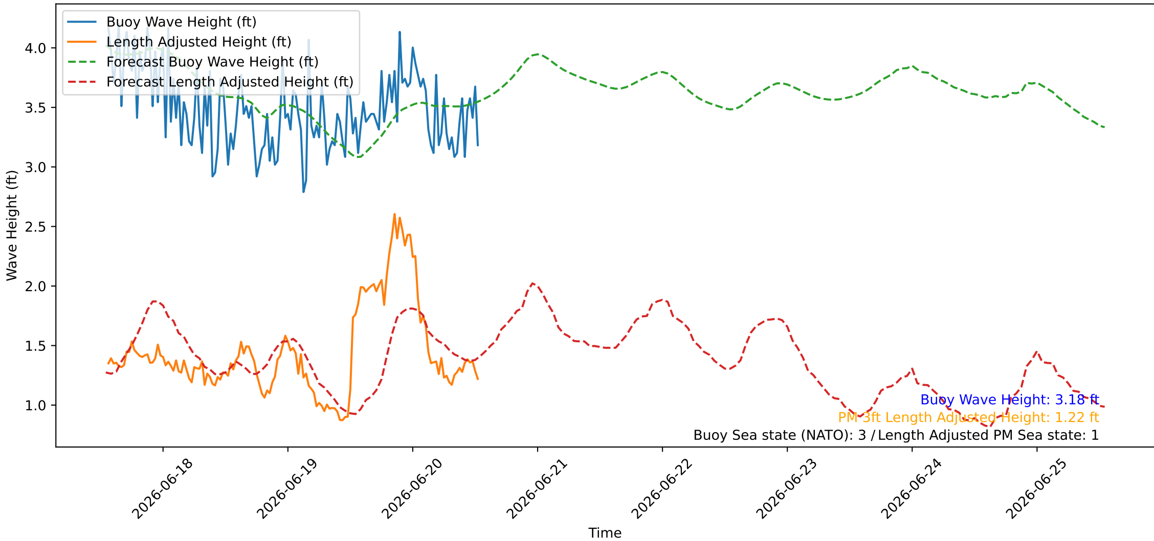
Wave Heights over Time for Oceanside Harbor at 2026-06-20 13:20:27
