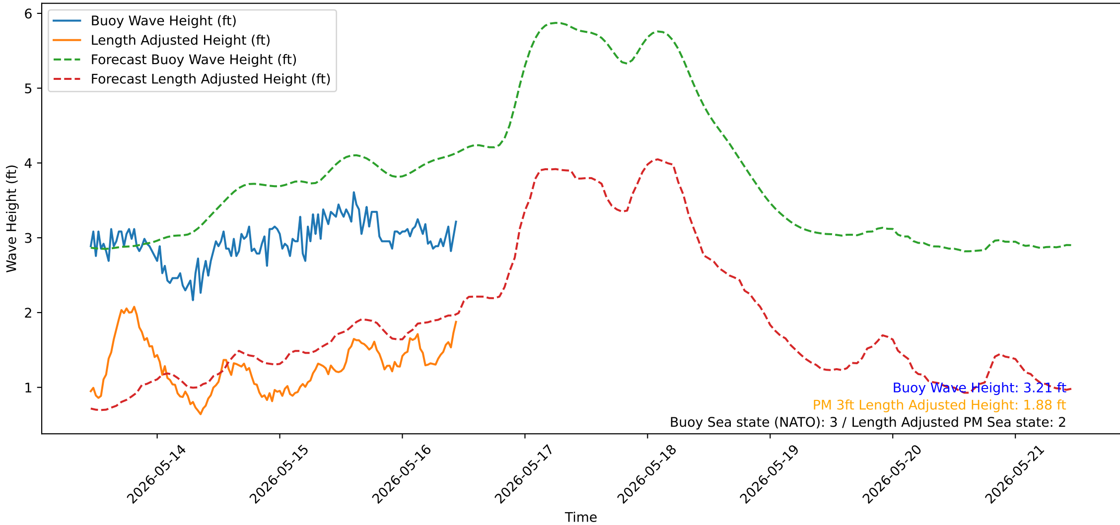
Wave Heights over Time for Oceanside Harbor at 2026-05-16 11:10:32
