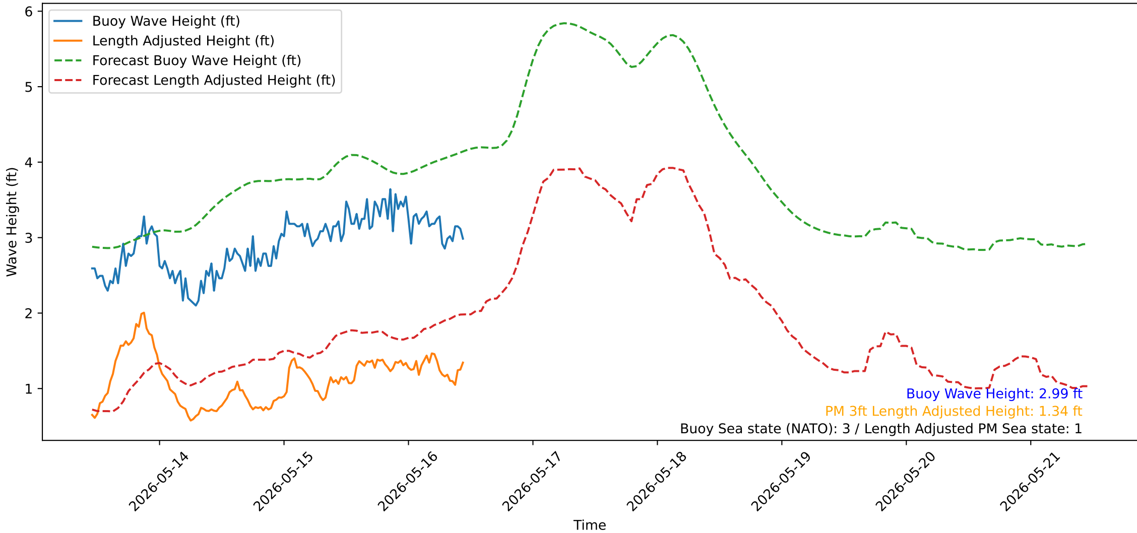
Wave Heights over Time for Green Beach at 2026-05-16 11:11:13
