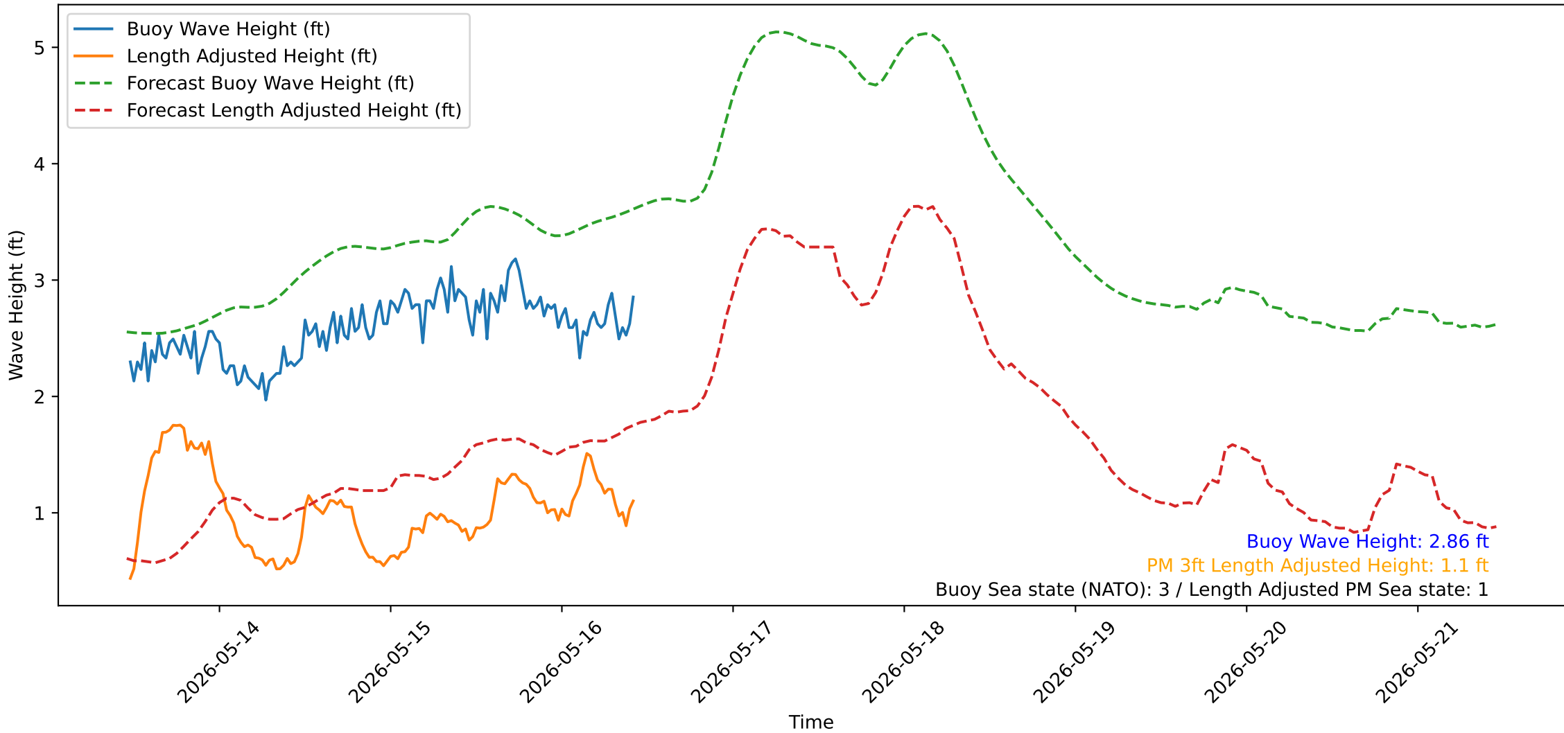
Wave Heights over Time for Red Beach at 2026-05-16 11:10:51
