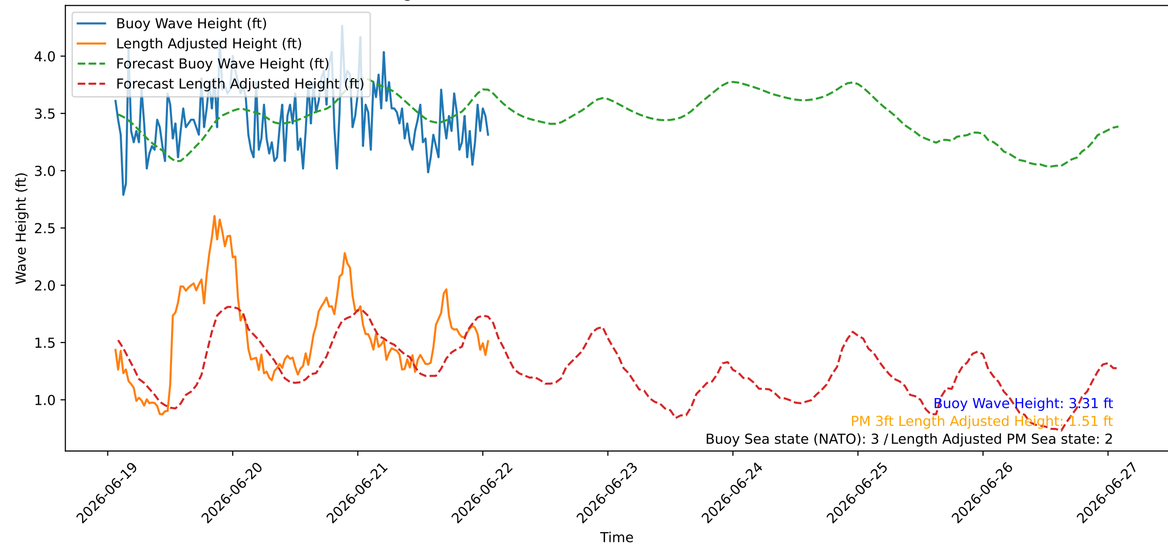
Wave Heights over Time for Oceanside Harbor at 2026-06-22 01:40:26
