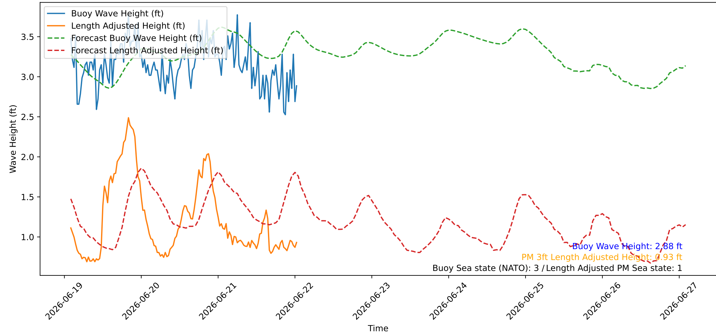
Wave Heights over Time for Red Beach at 2026-06-22 01:40:45
