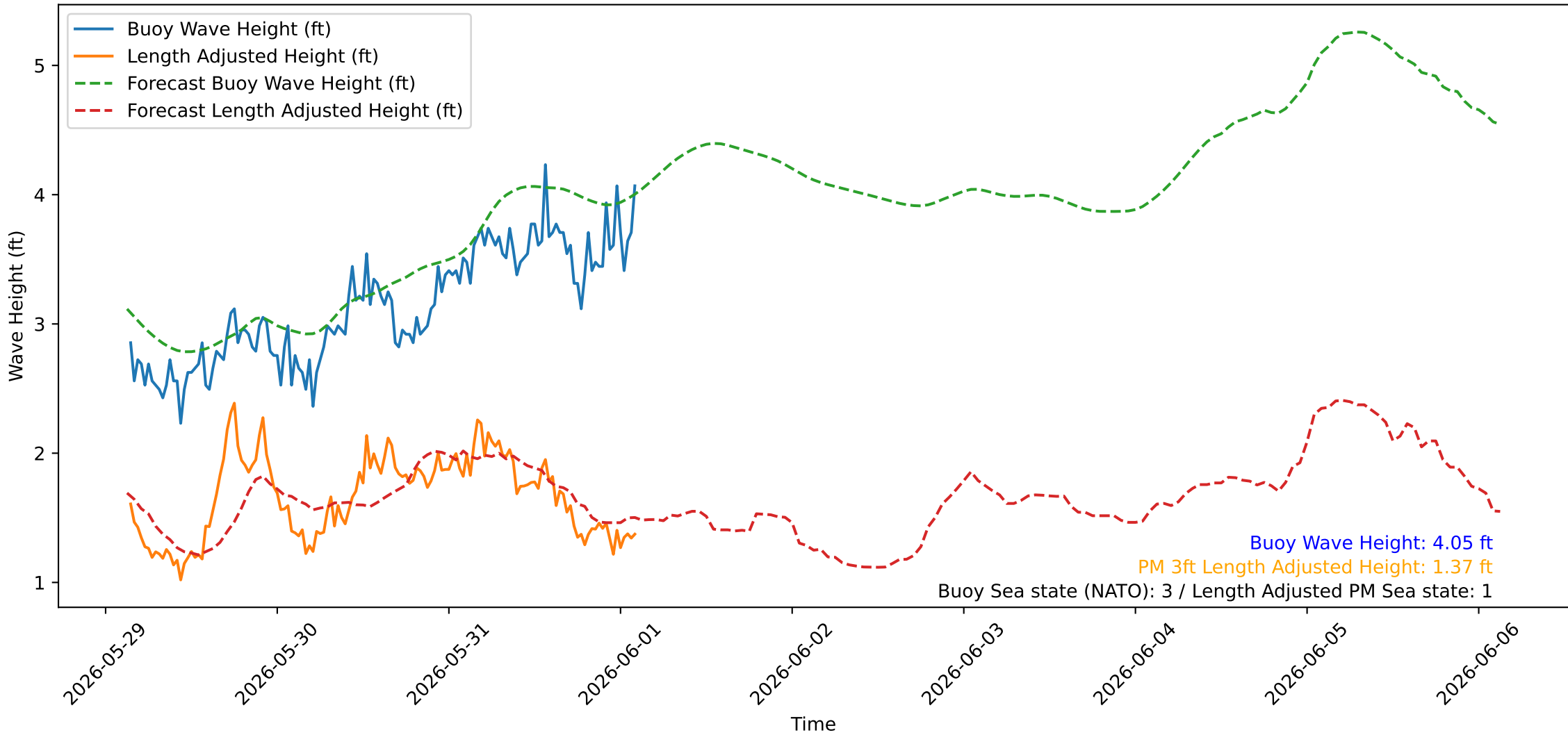
Wave Heights over Time for Oceanside Harbor at 2026-06-01 03:20:25
