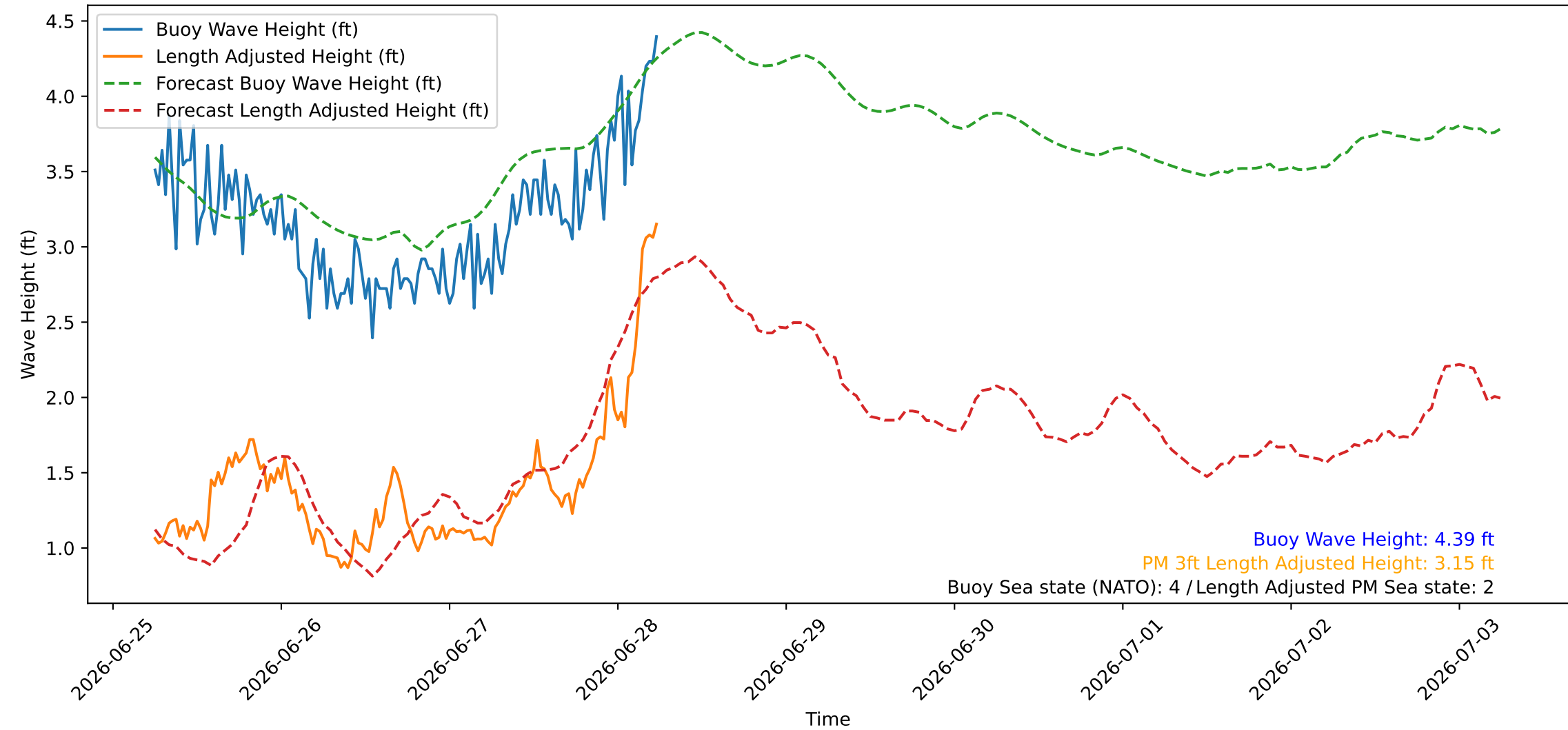
Wave Heights over Time for Oceanside Harbor at 2026-06-28 06:10:25
