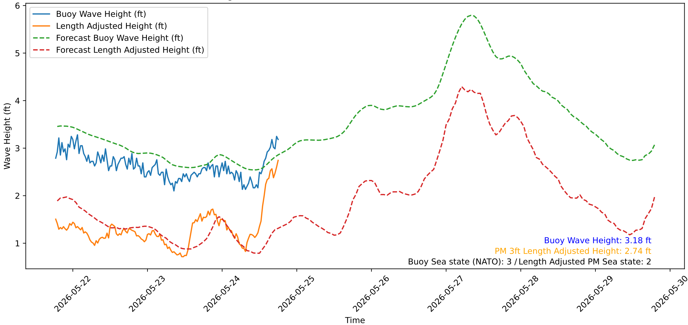
Wave Heights over Time for Oceanside Harbor at 2026-05-24 18:30:32
