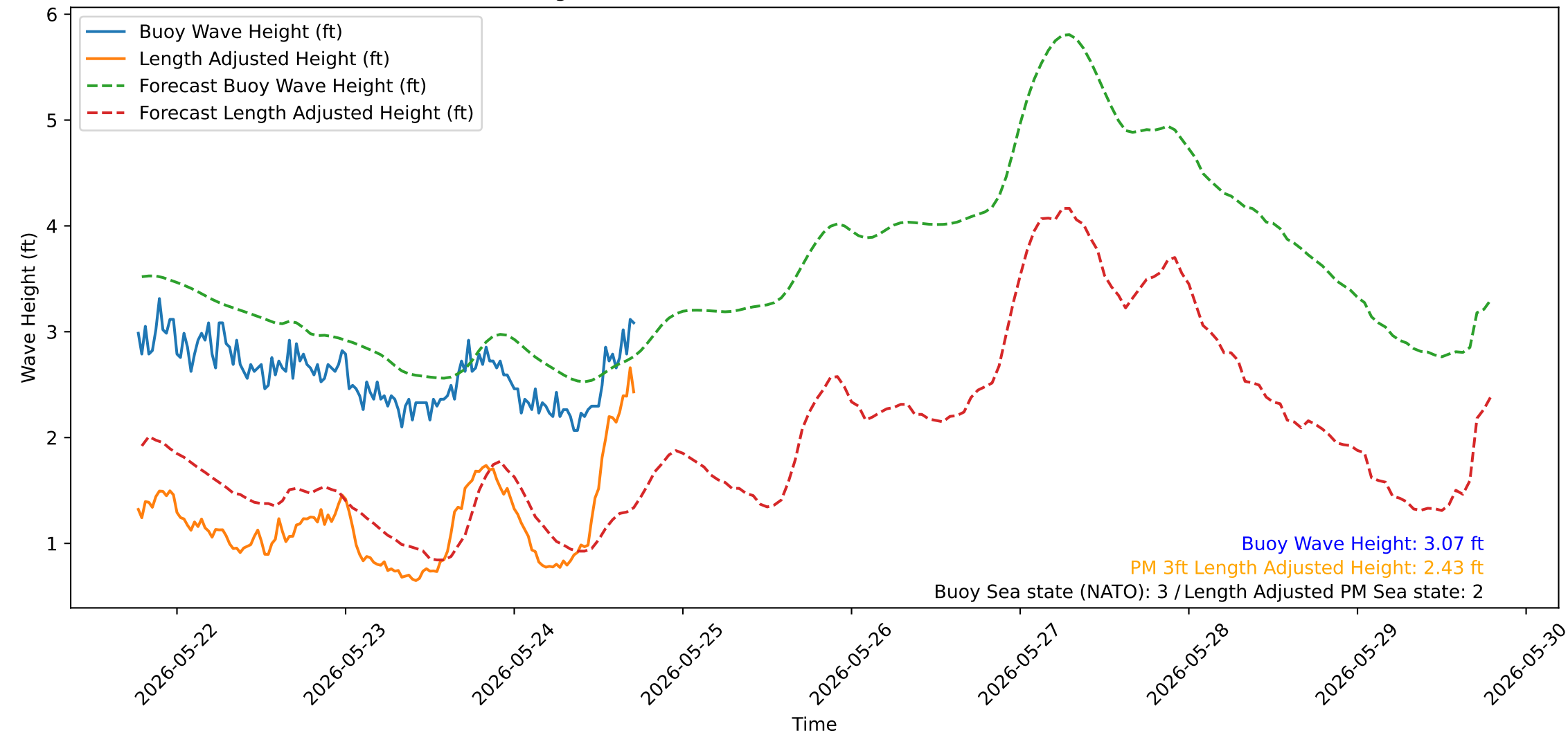
Wave Heights over Time for Green Beach at 2026-05-24 18:31:15
