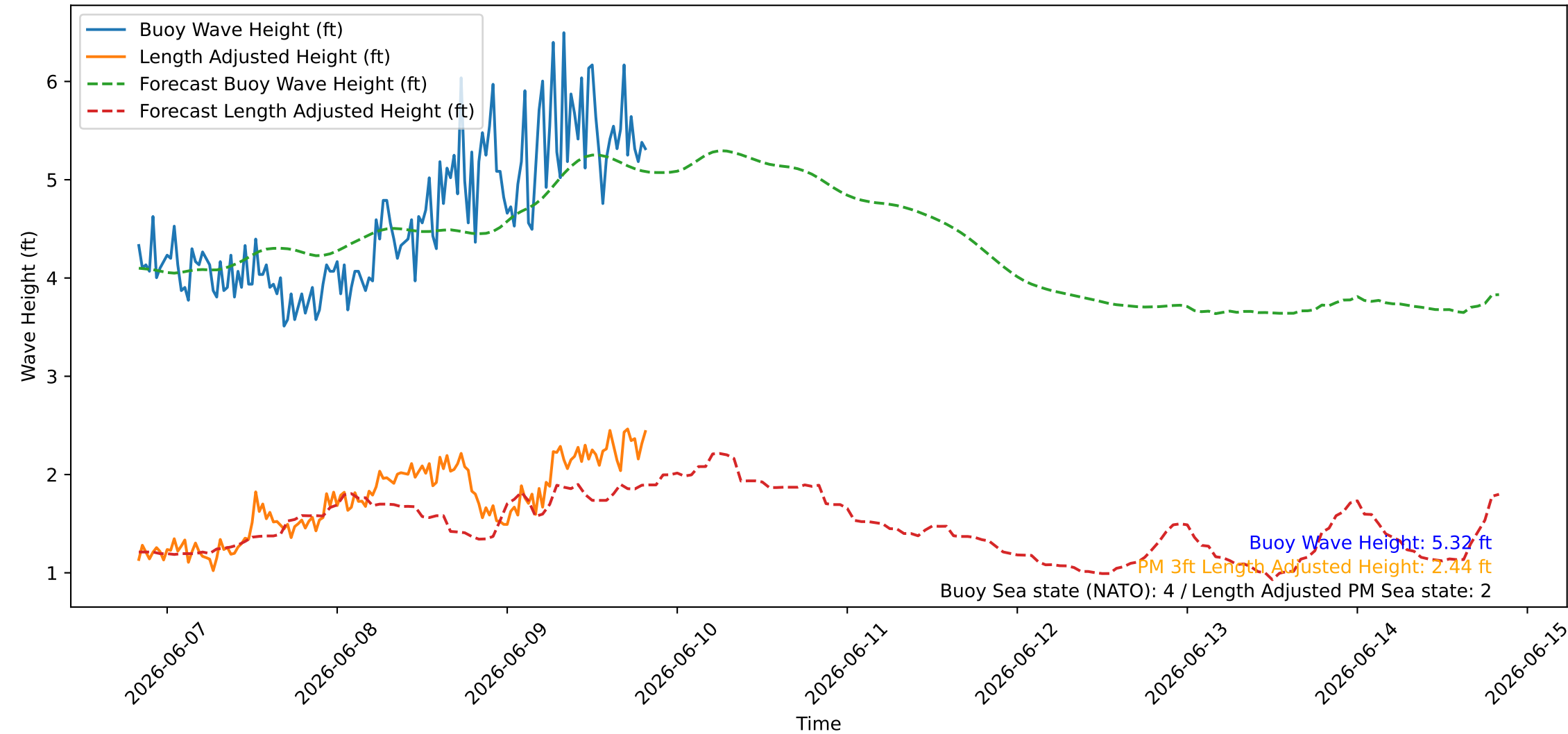
Wave Heights over Time for Oceanside Harbor at 2026-06-09 20:10:27
