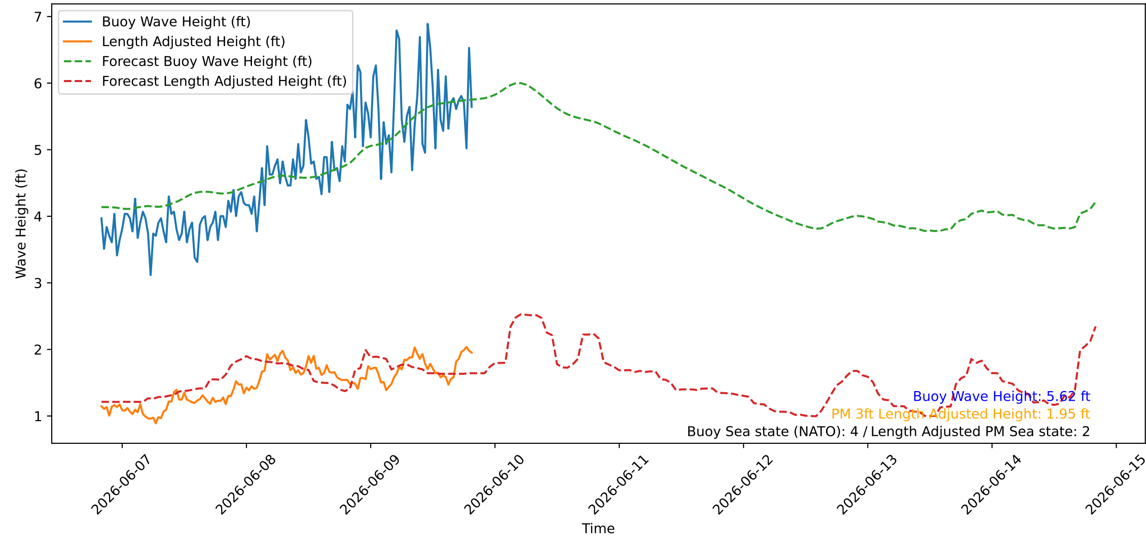
Wave Heights over Time for Green Beach at 2026-06-09 20:11:11
