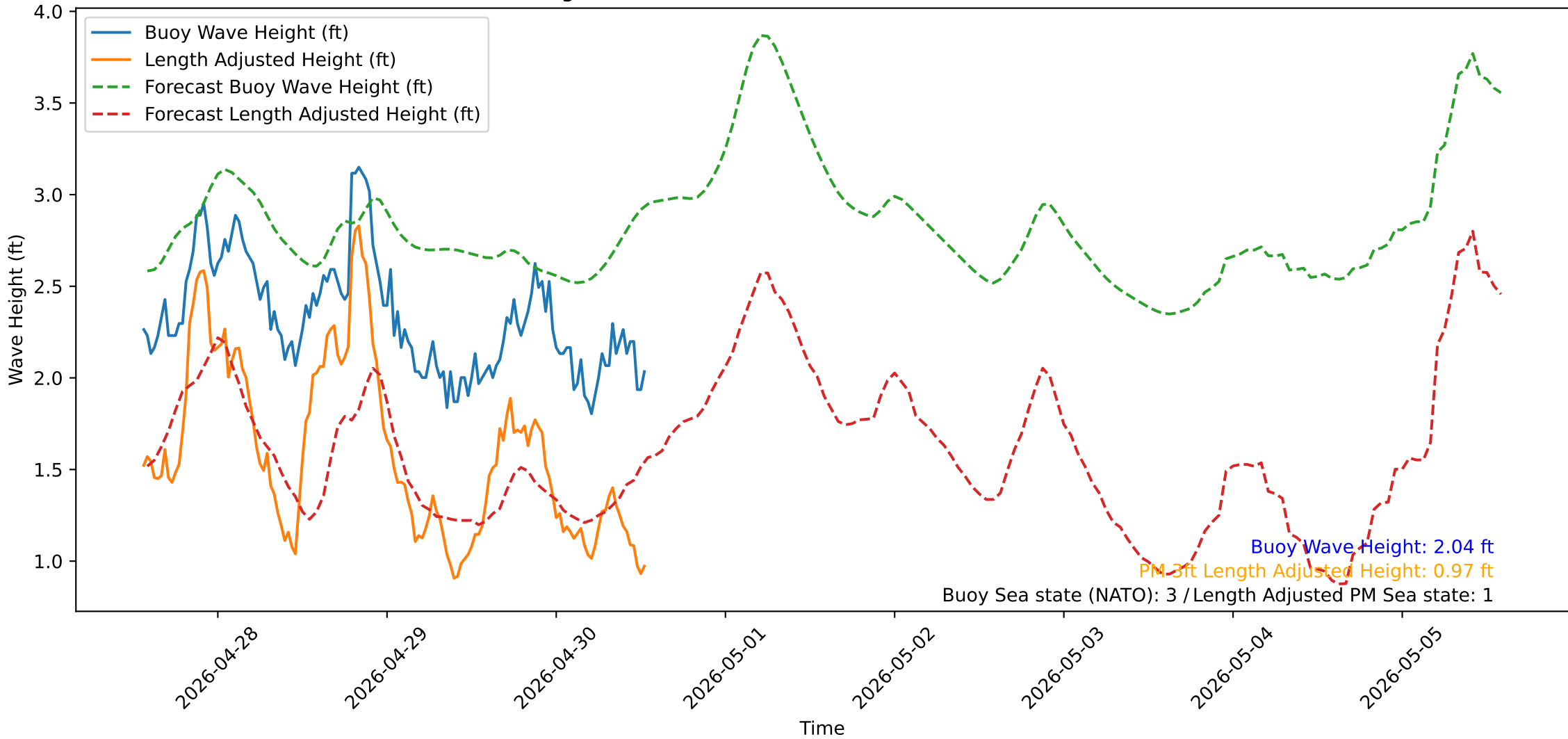
Wave Heights over Time for Green Beach at 2026-04-30 13:31:13
