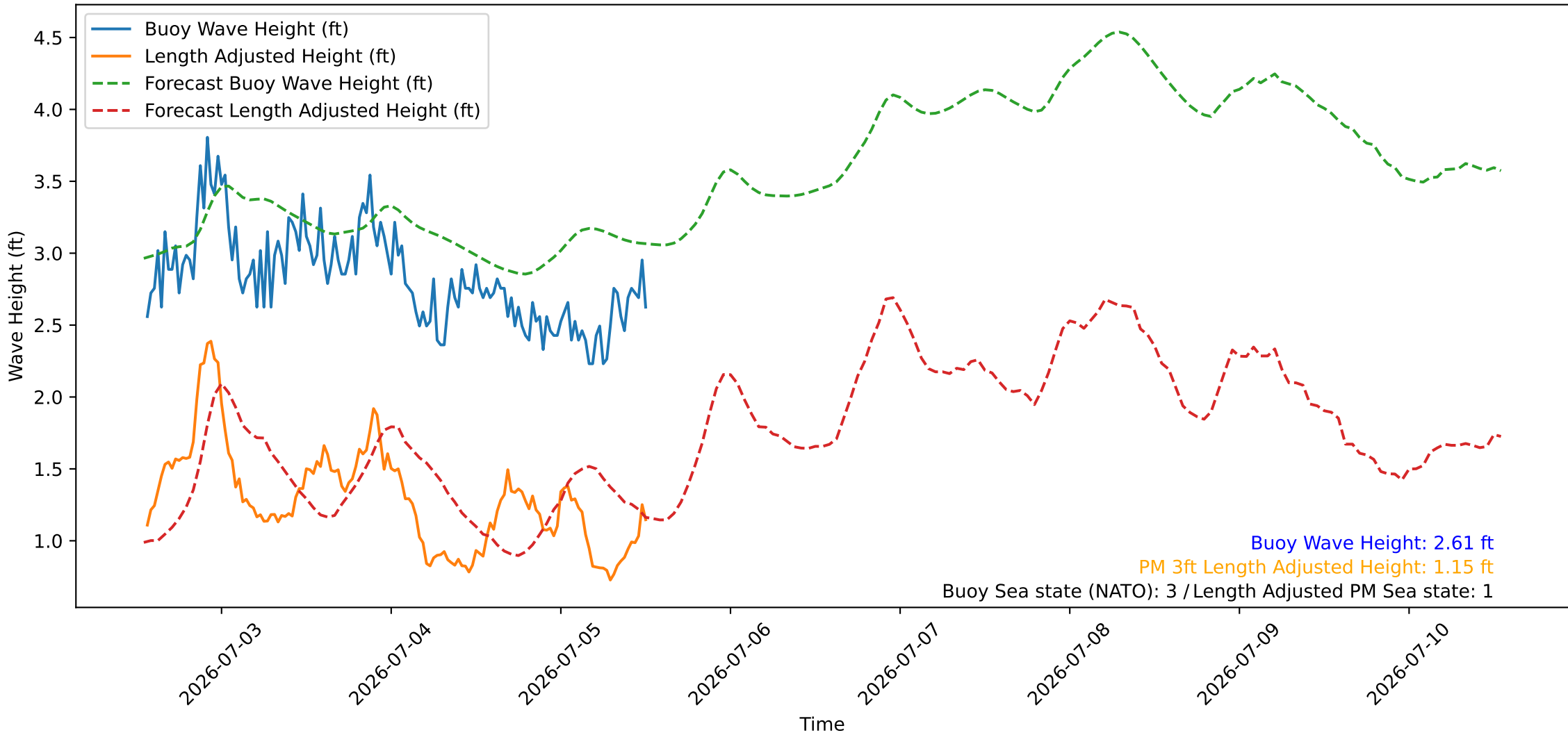
Wave Heights over Time for Red Beach at 2026-07-05 13:00:45
