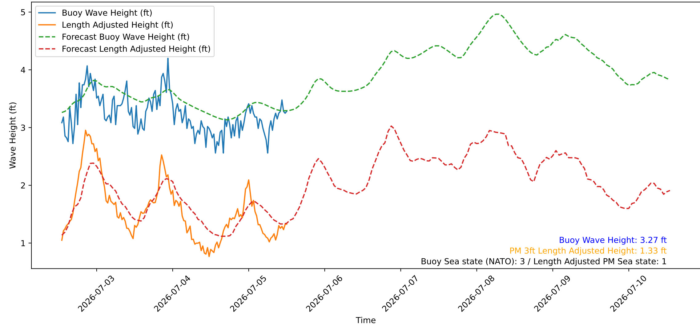
Wave Heights over Time for Green Beach at 2026-07-05 13:01:08
