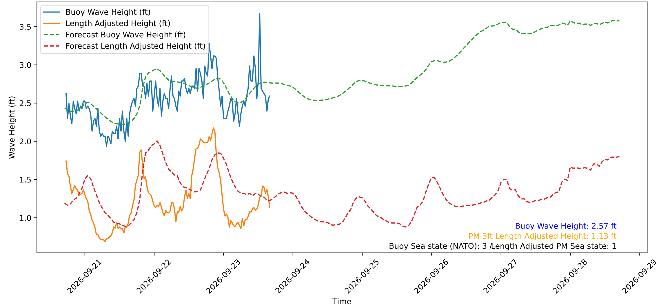
Wave Heights over Time for Red Beach at 2026-09-23 17:00:49
