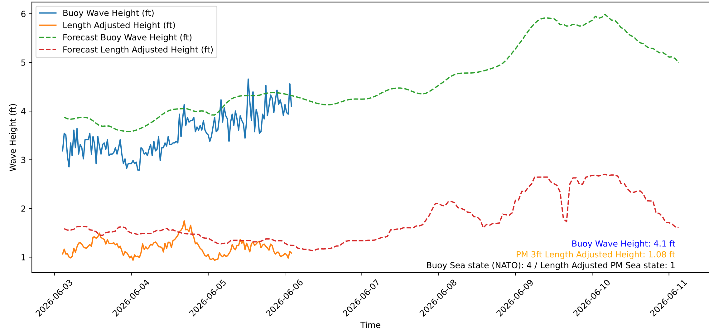
Wave Heights over Time for Green Beach at 2026-06-06 02:41:08
