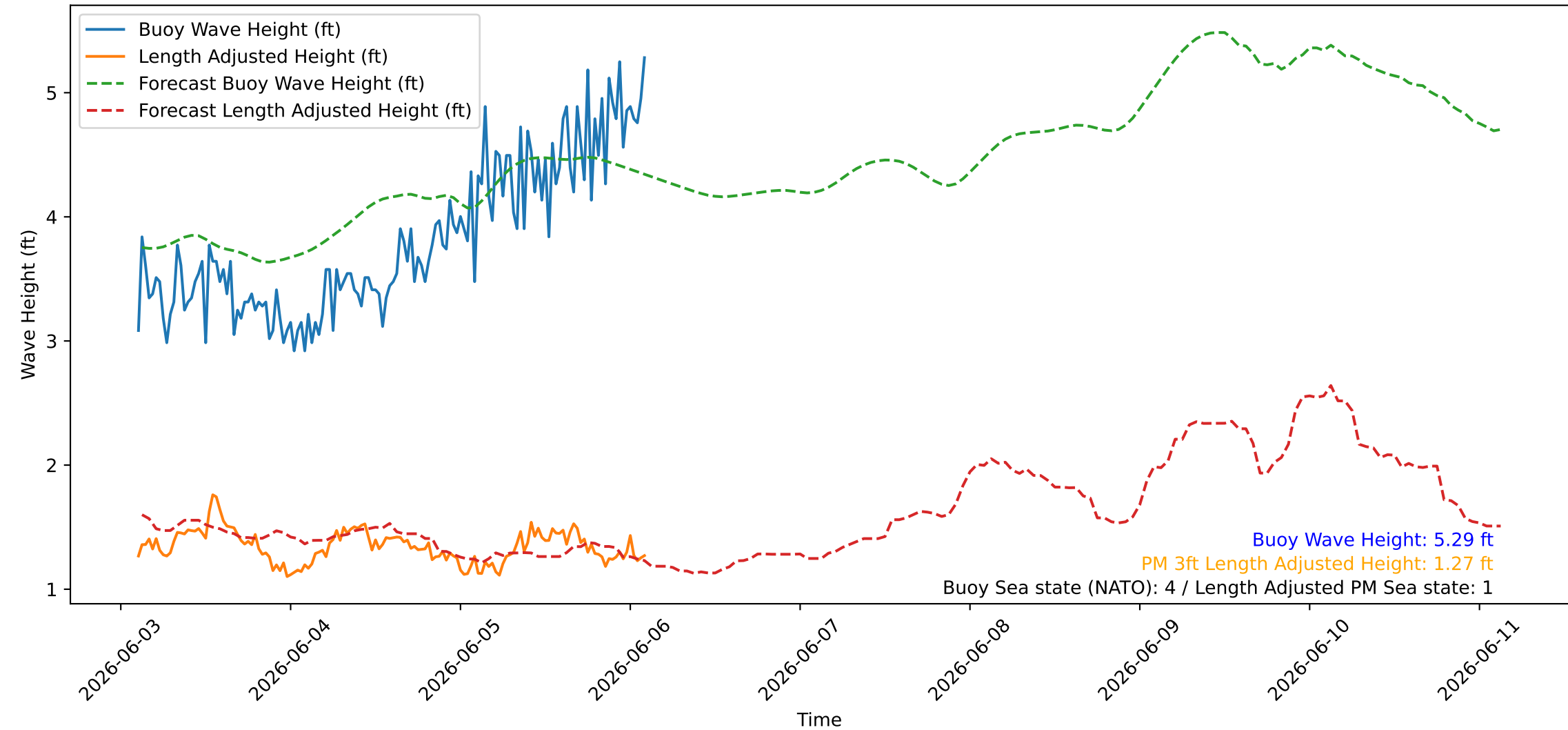
Wave Heights over Time for Oceanside Harbor at 2026-06-06 02:40:26
