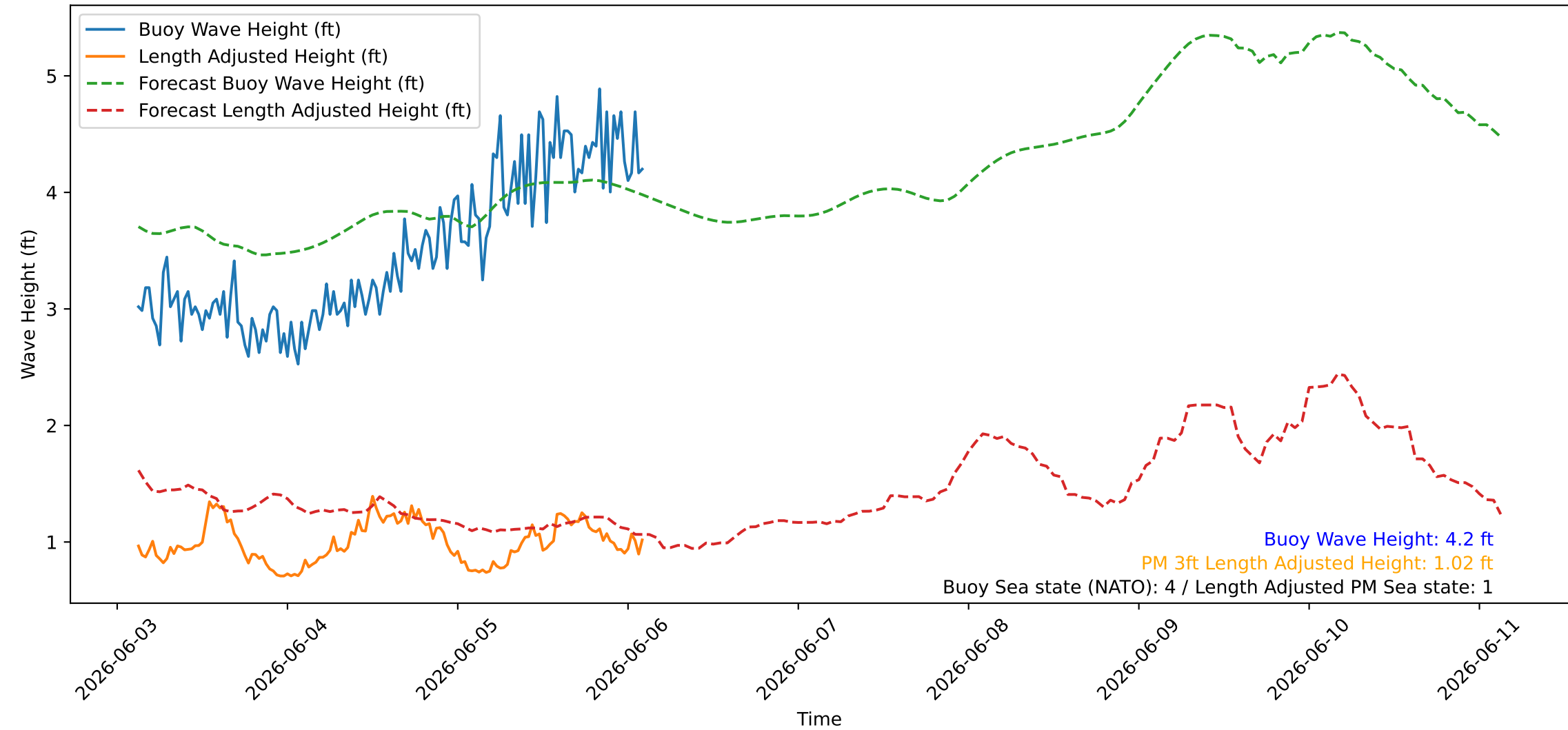
Wave Heights over Time for Red Beach at 2026-06-06 02:40:46
