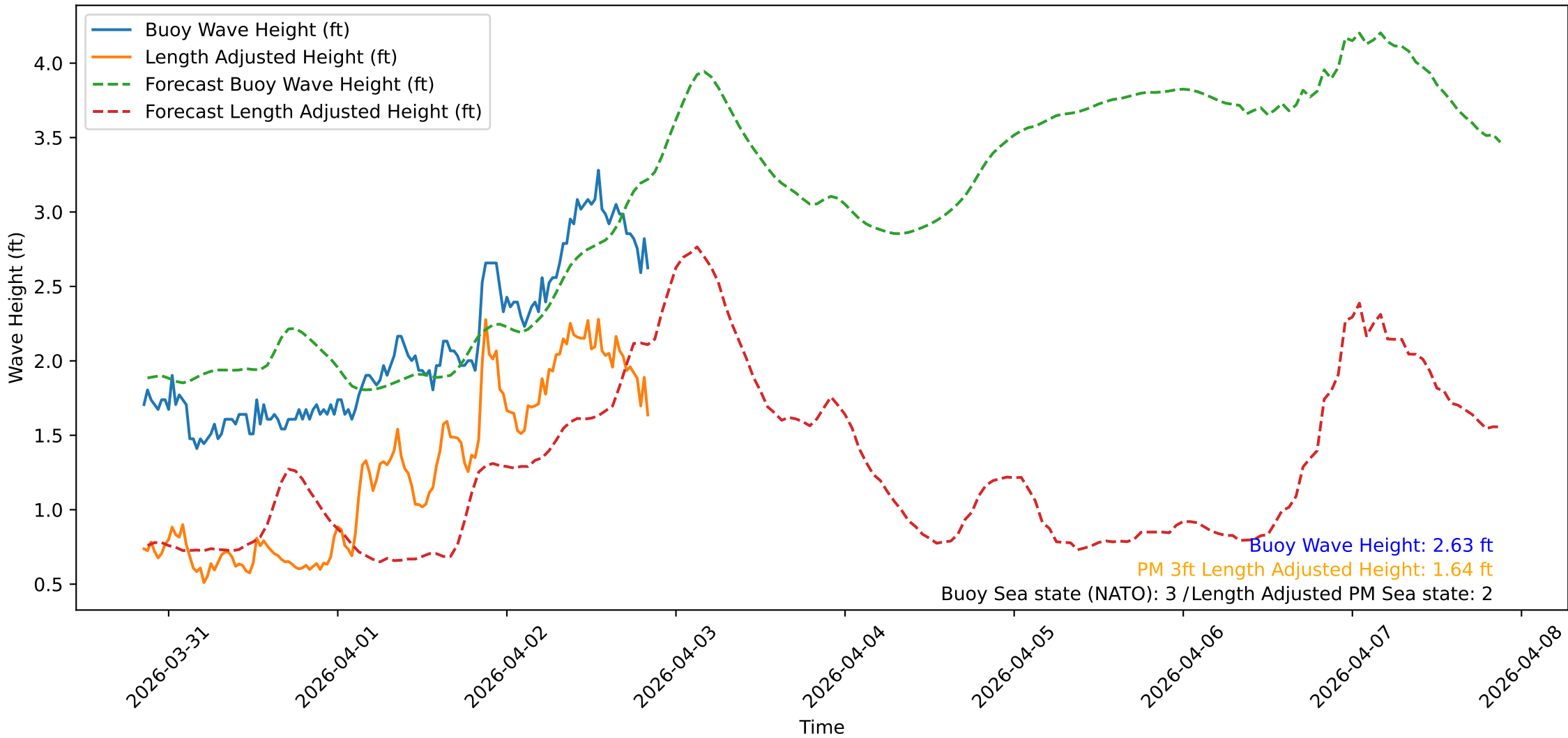
Wave Heights over Time for Green Beach at 2026-04-02 20:41:10
