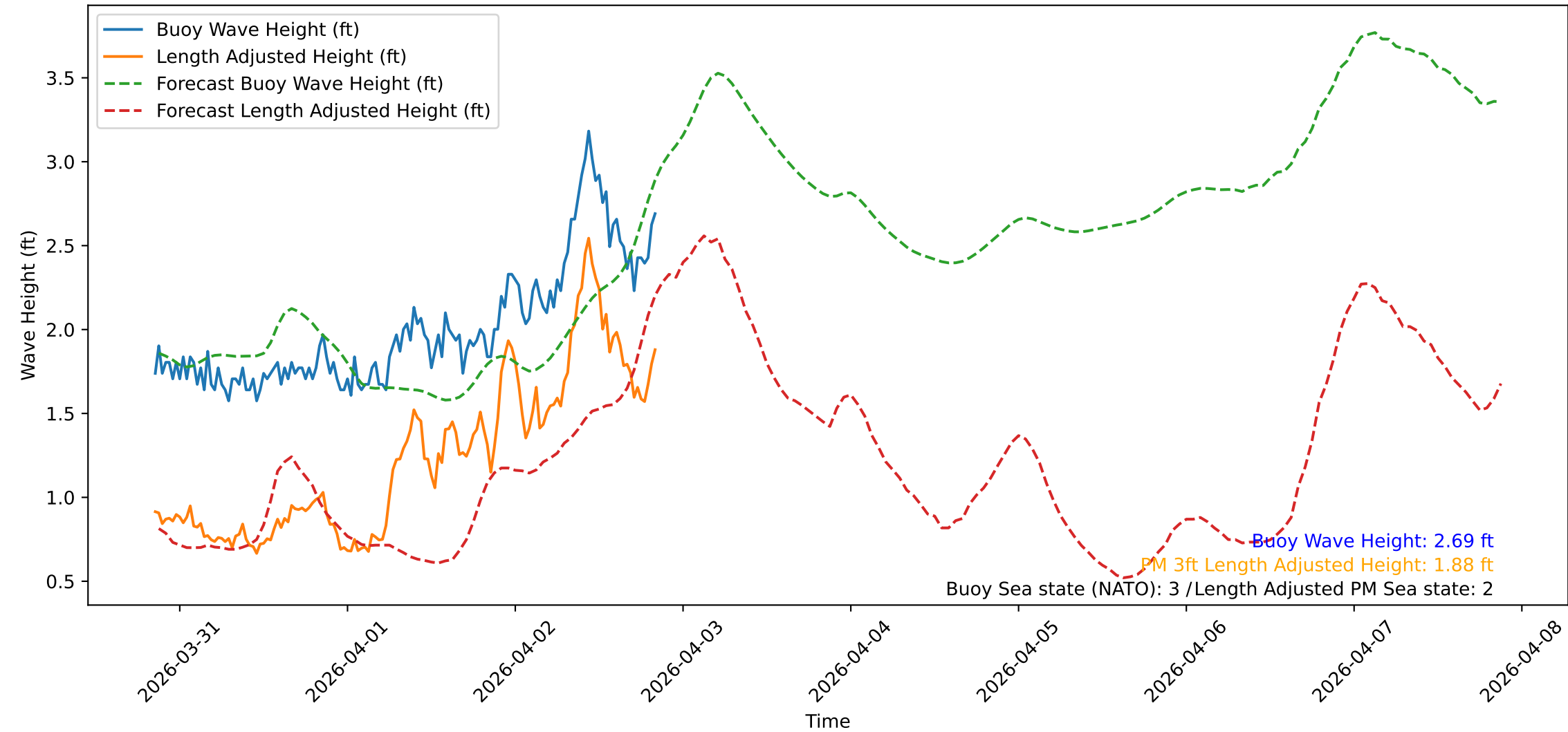
Wave Heights over Time for Oceanside Harbor at 2026-04-02 20:40:31
