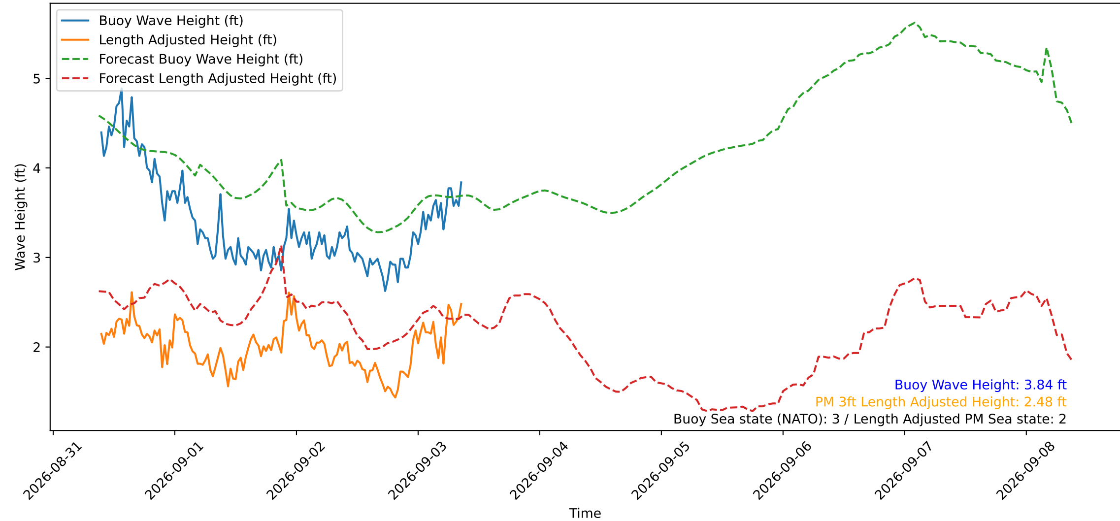
Wave Heights over Time for Oceanside Harbor at 2026-09-03 09:20:30
