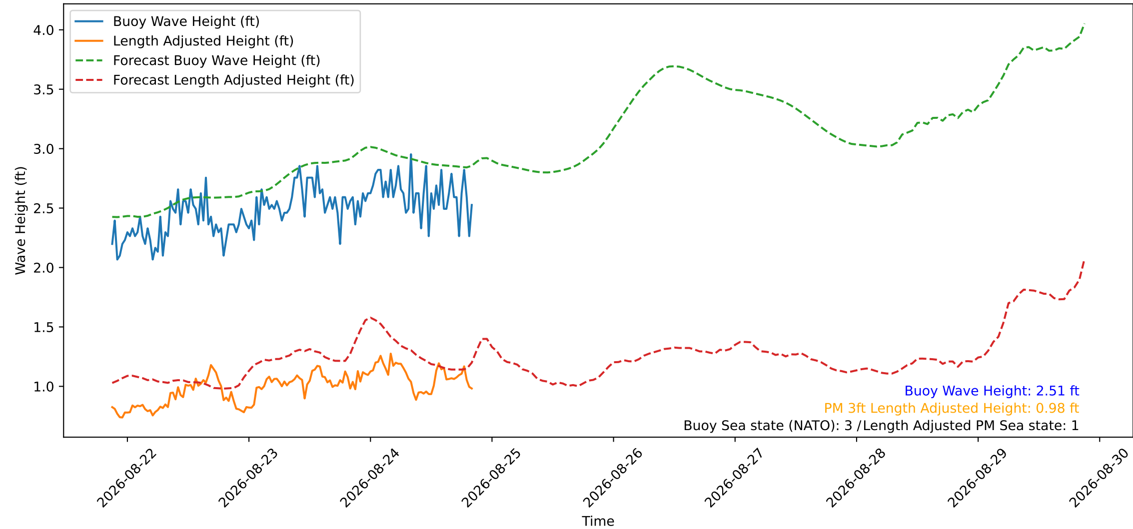
Wave Heights over Time for Red Beach at 2026-08-24 20:50:51
