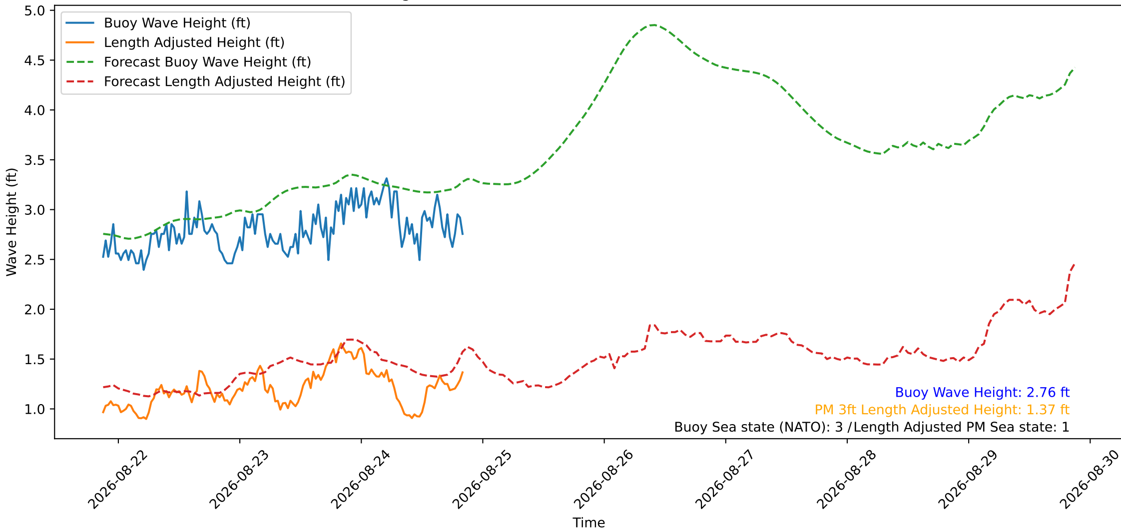
Wave Heights over Time for Green Beach at 2026-08-24 20:51:15
