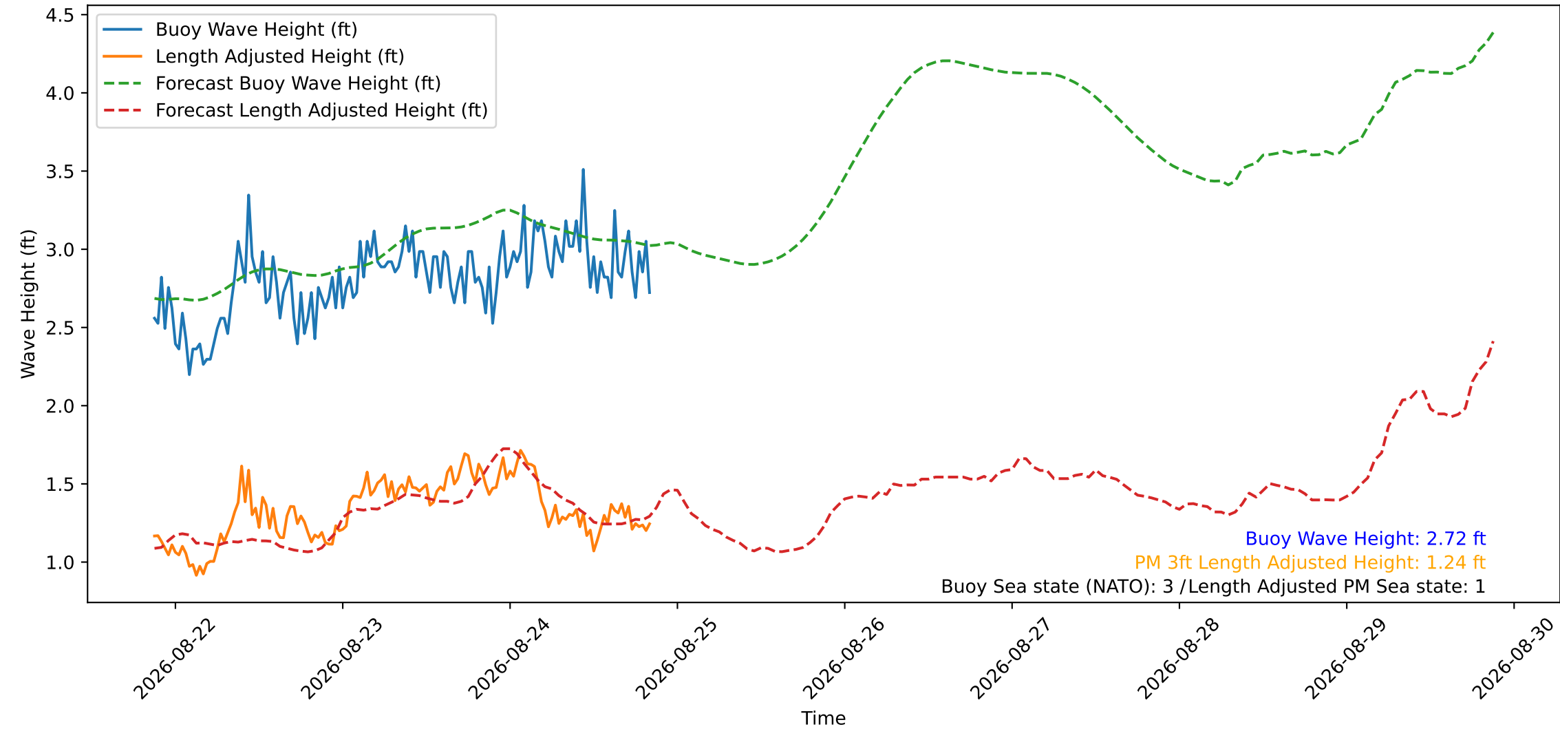
Wave Heights over Time for Oceanside Harbor at 2026-08-24 20:50:29
