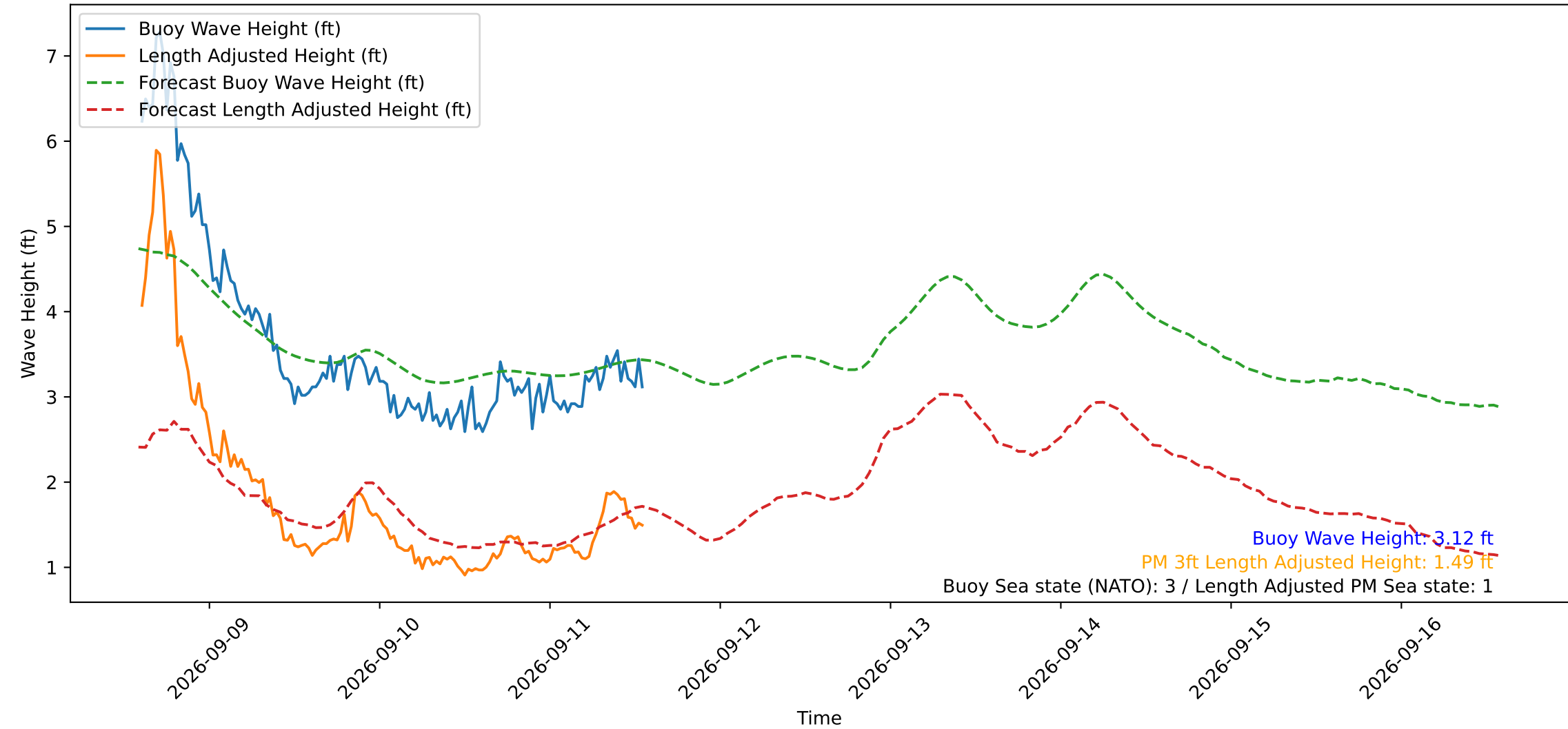
Wave Heights over Time for Green Beach at 2026-09-11 14:01:14
