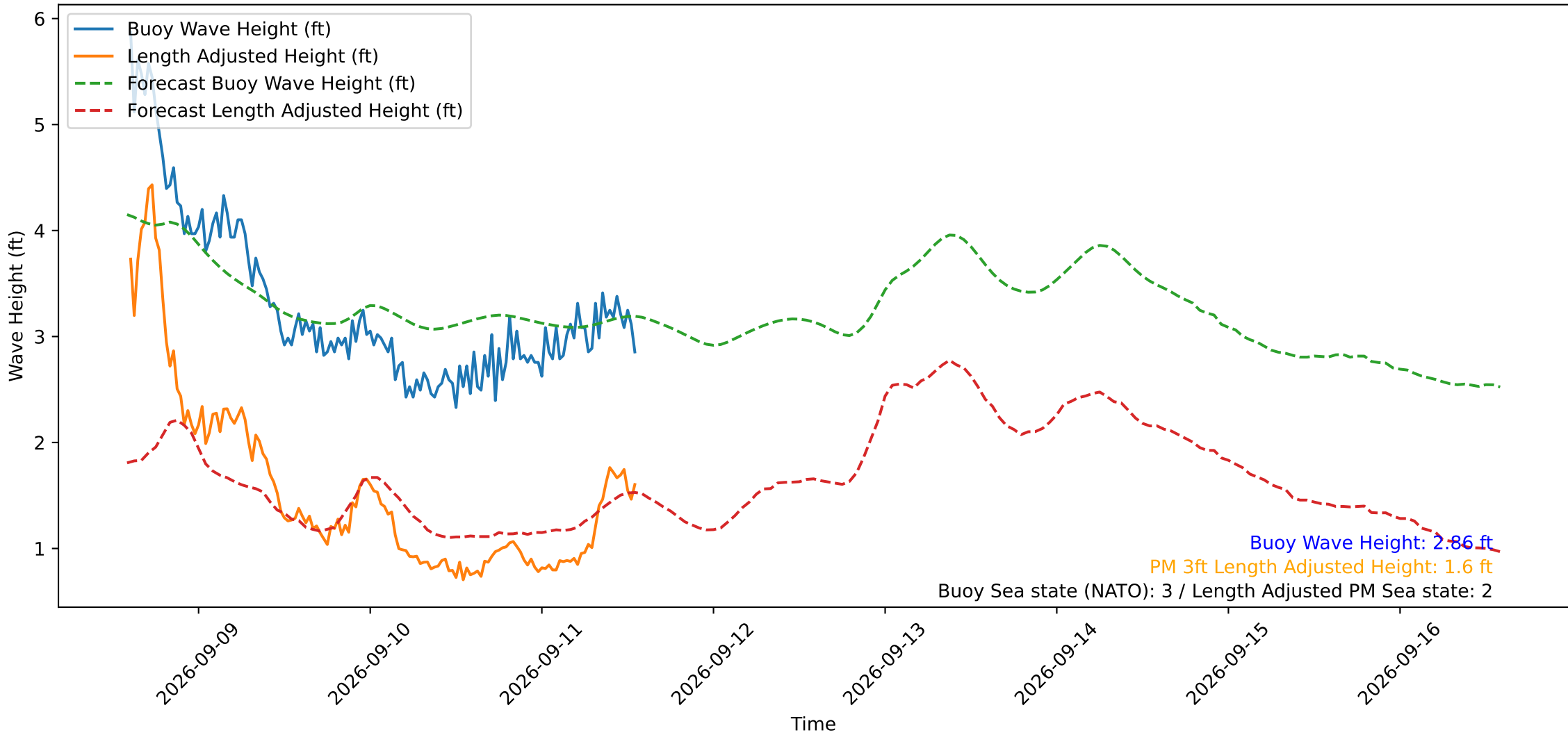
Wave Heights over Time for Red Beach at 2026-09-11 14:00:50
