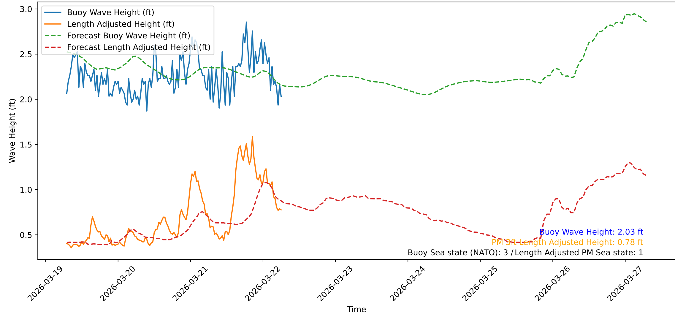
Wave Heights over Time for Red Beach at 2026-03-22 06:50:47
