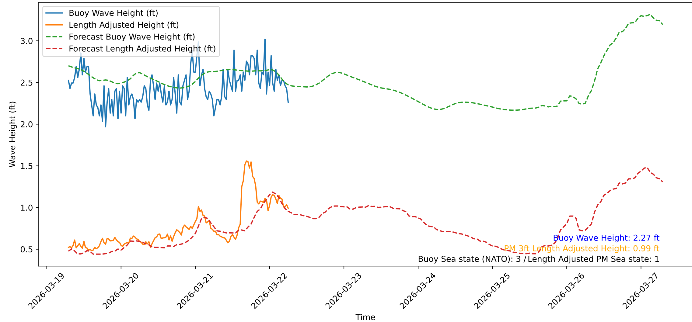
Wave Heights over Time for Oceanside Harbor at 2026-03-22 06:50:32
