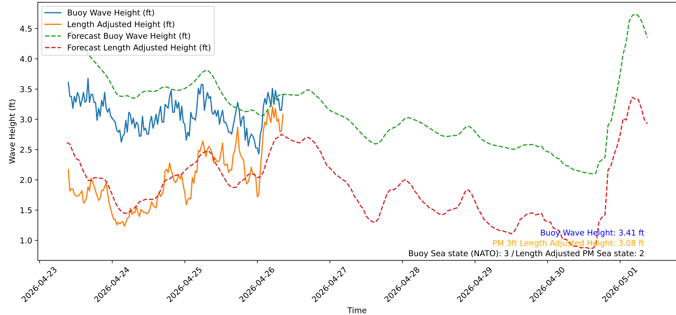
Wave Heights over Time for Green Beach at 2026-04-26 09:21:14
