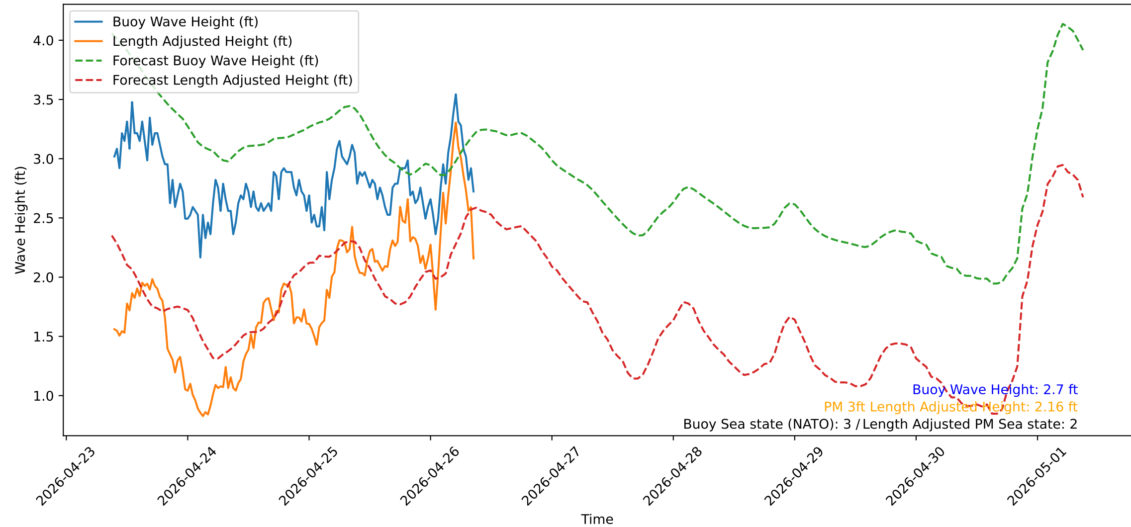
Wave Heights over Time for Red Beach at 2026-04-26 09:20:52
