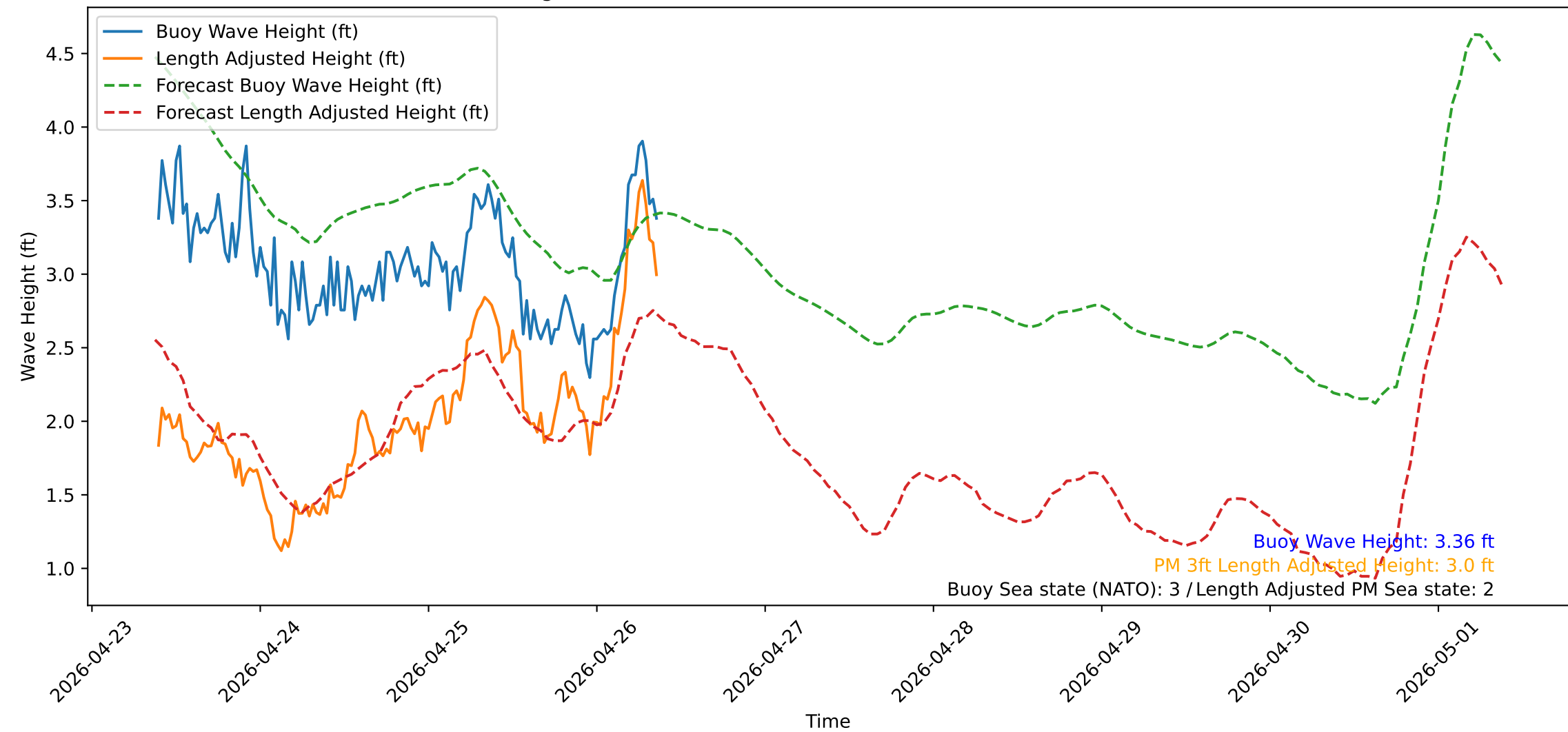
Wave Heights over Time for Oceanside Harbor at 2026-04-26 09:20:31
