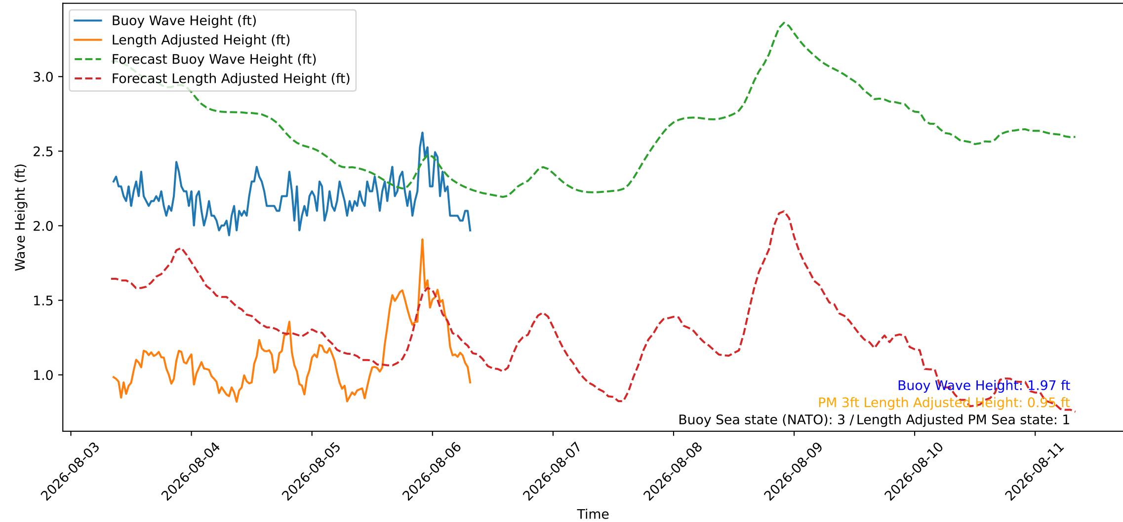
Wave Heights over Time for Green Beach at 2026-08-06 08:21:10
