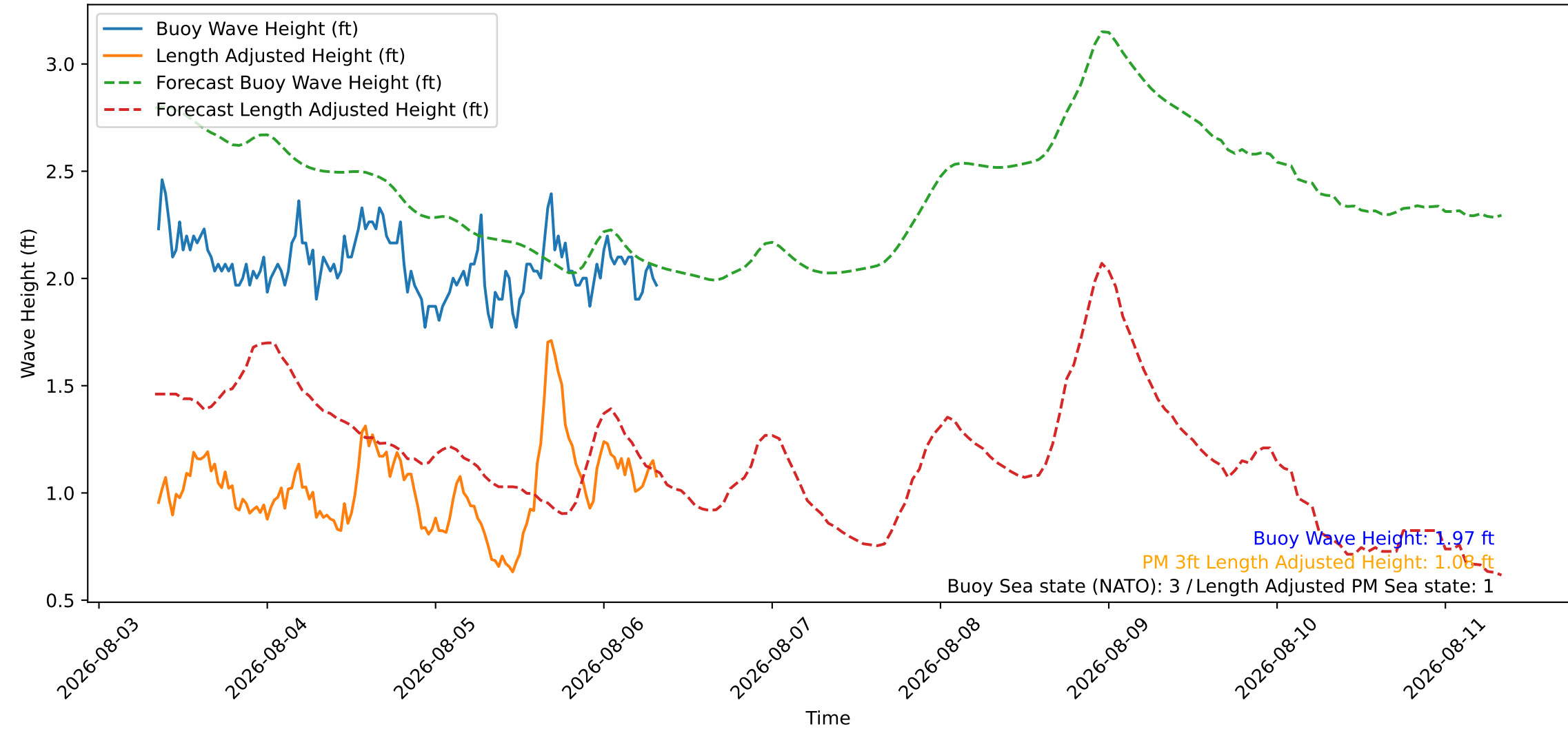
Wave Heights over Time for Red Beach at 2026-08-06 08:20:47
