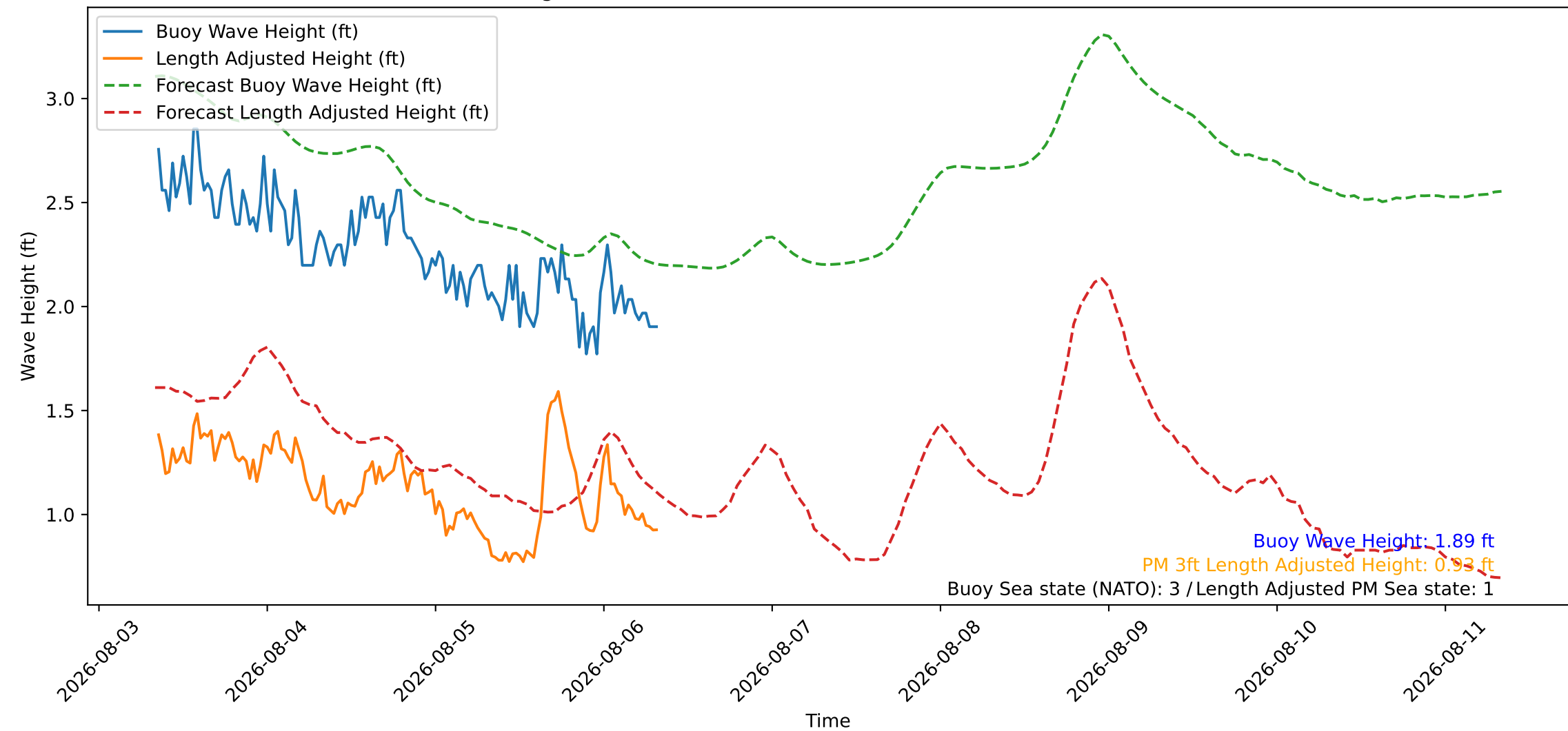
Wave Heights over Time for Oceanside Harbor at 2026-08-06 08:20:26
