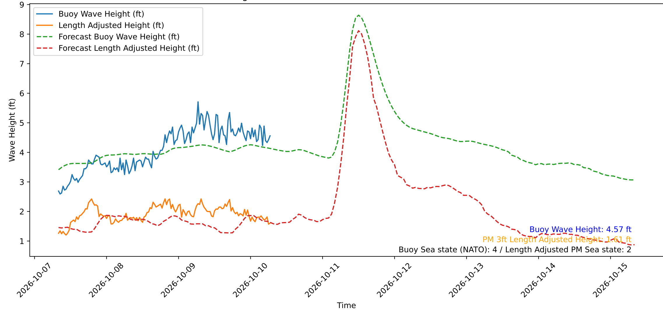
Wave Heights over Time for Red Beach at 2026-10-10 07:30:48
