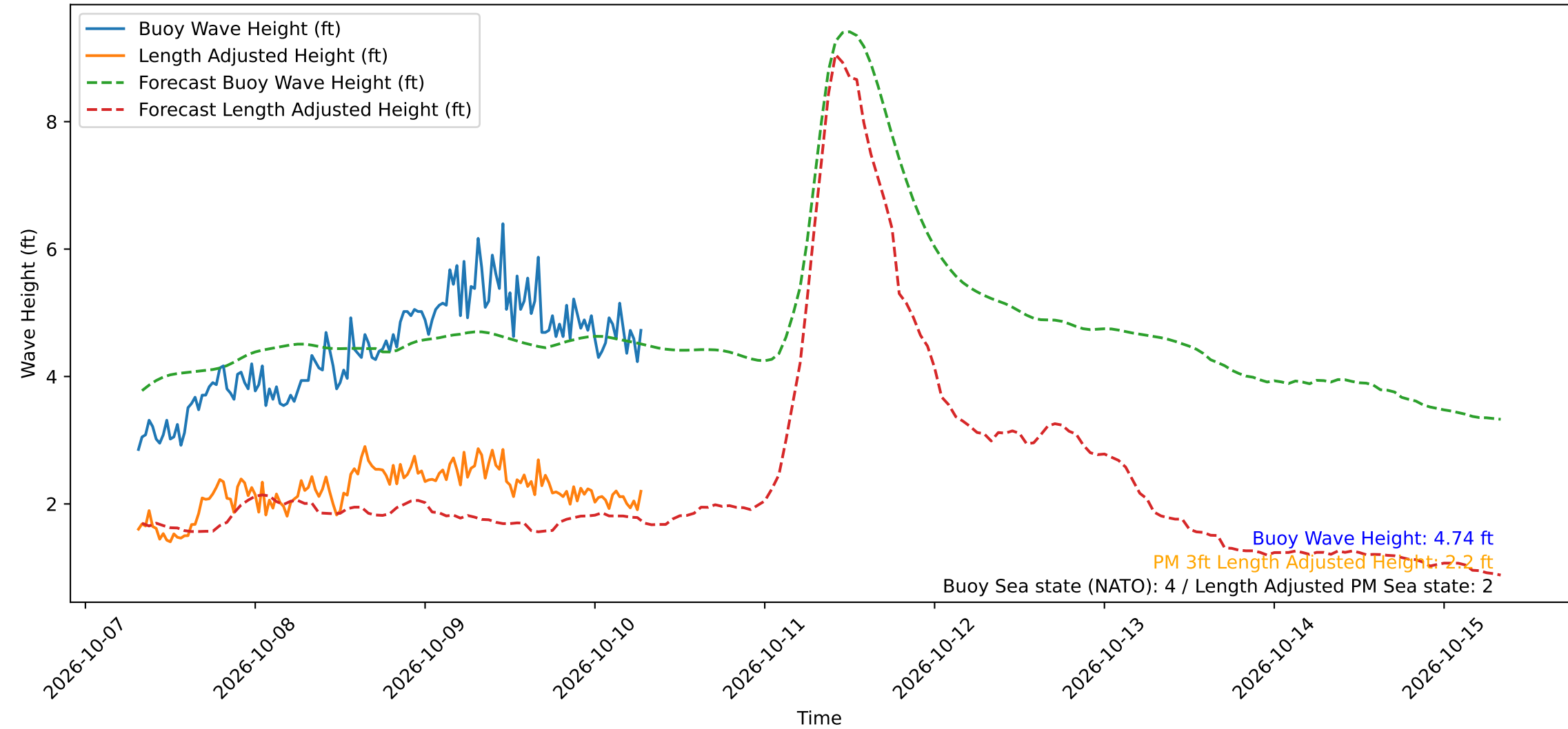
Wave Heights over Time for Oceanside Harbor at 2026-10-10 07:30:29
