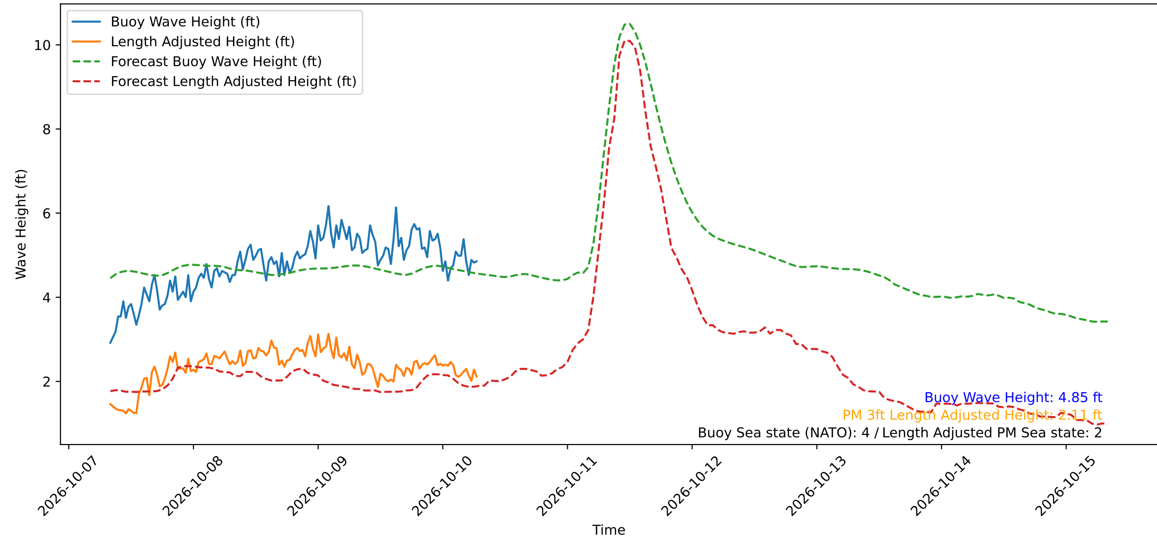
Wave Heights over Time for Green Beach at 2026-10-10 07:31:11
