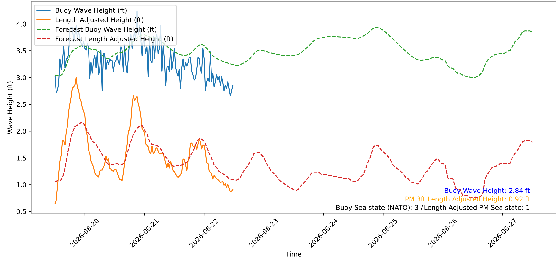
Wave Heights over Time for Green Beach at 2026-06-22 12:11:08
