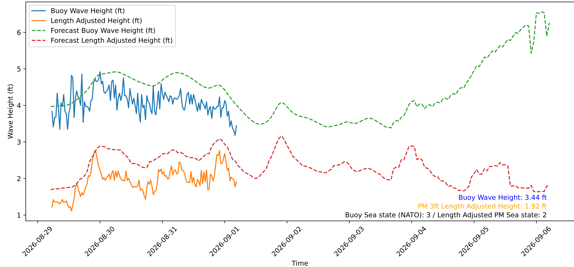
Wave Heights over Time for Green Beach at 2026-09-01 05:21:15
