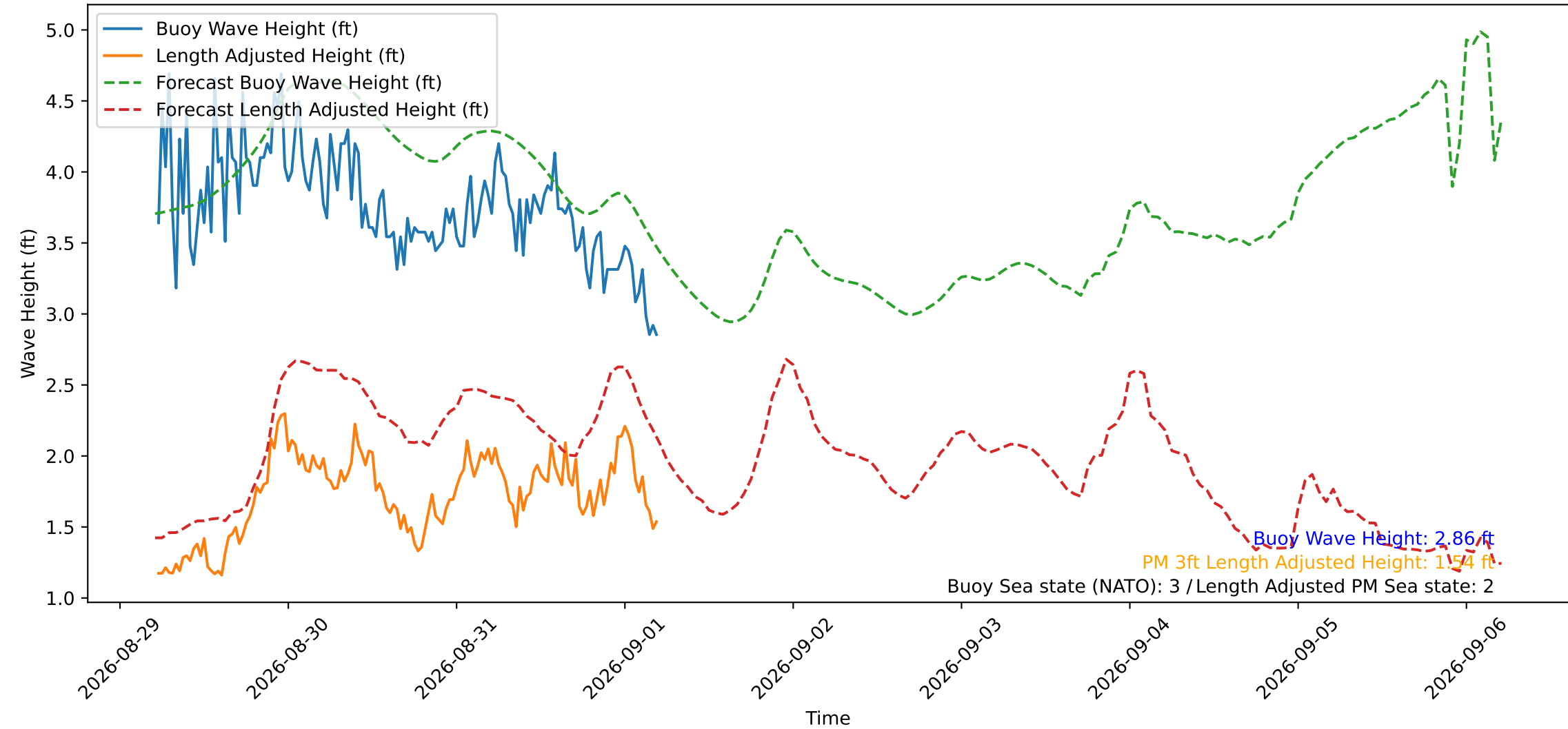
Wave Heights over Time for Red Beach at 2026-09-01 05:20:50
