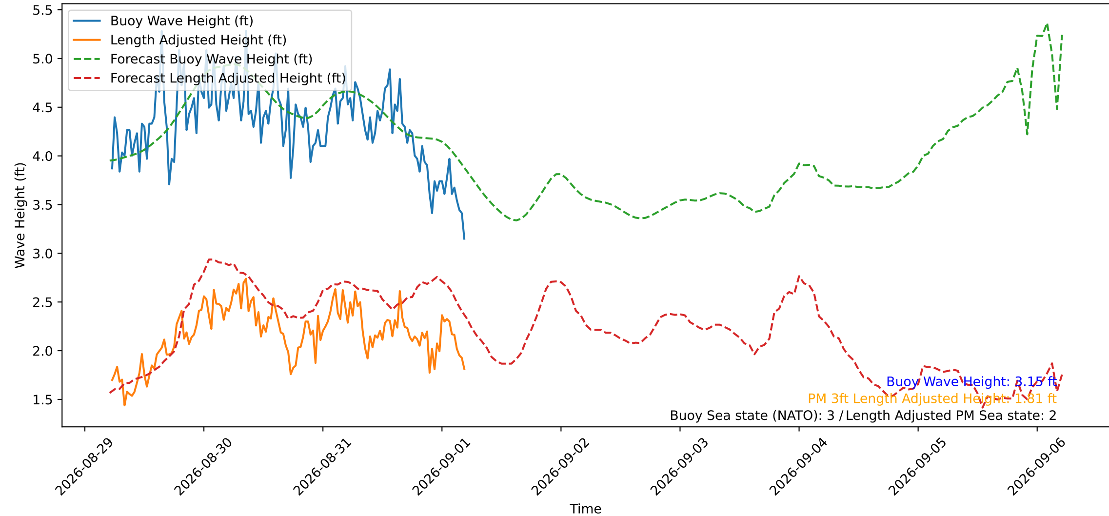
Wave Heights over Time for Oceanside Harbor at 2026-09-01 05:20:29
