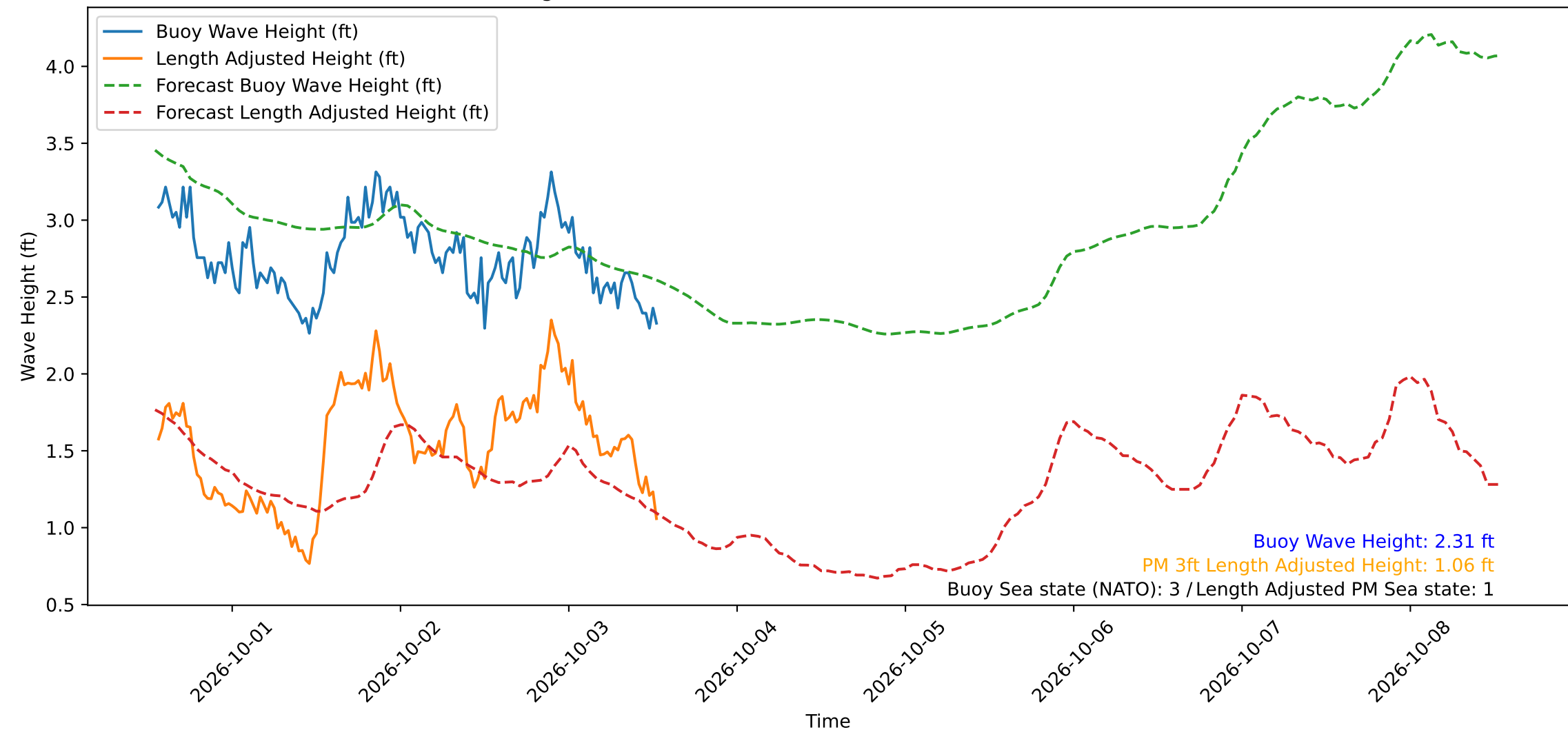
Wave Heights over Time for Oceanside Harbor at 2026-10-03 13:20:30
