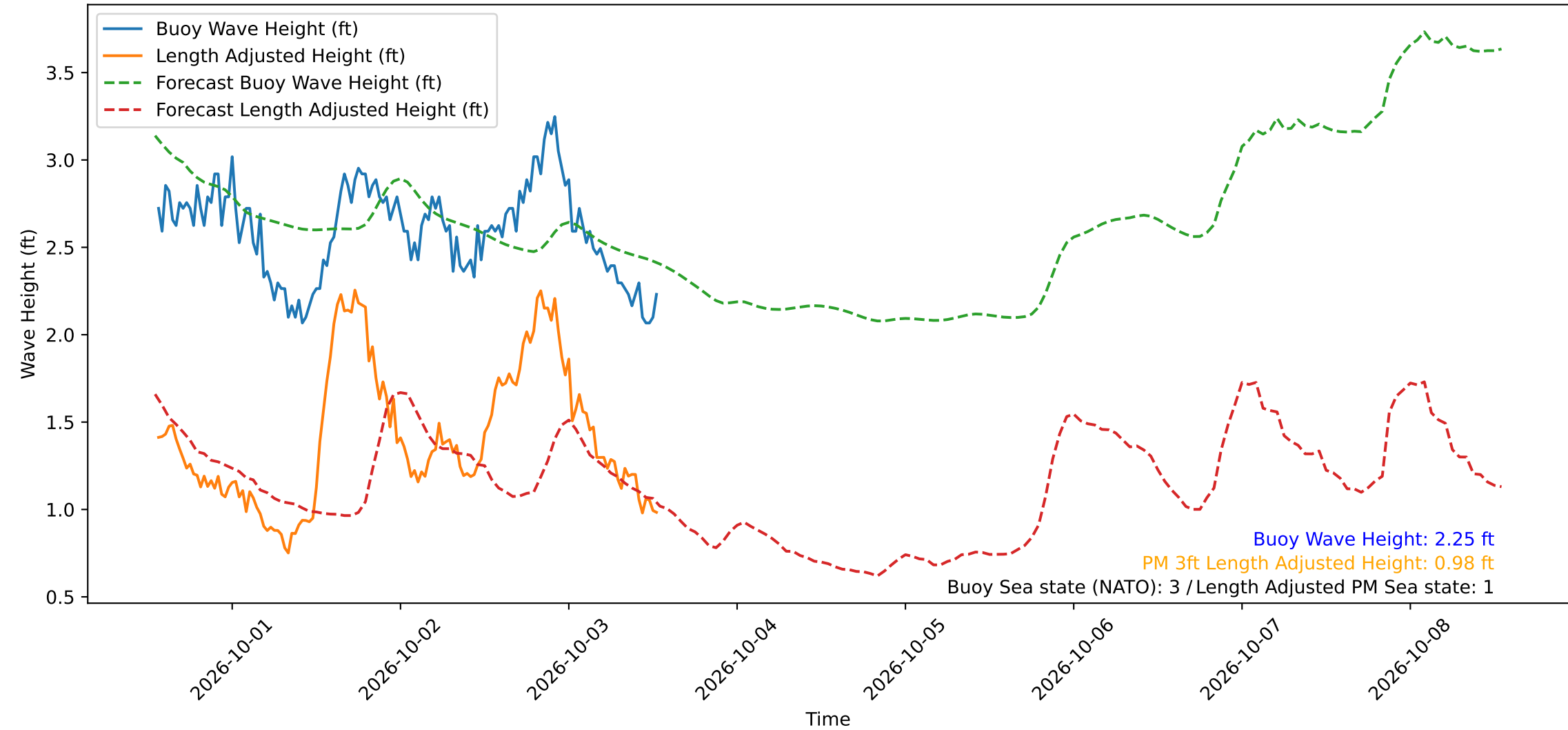
Wave Heights over Time for Red Beach at 2026-10-03 13:20:51
