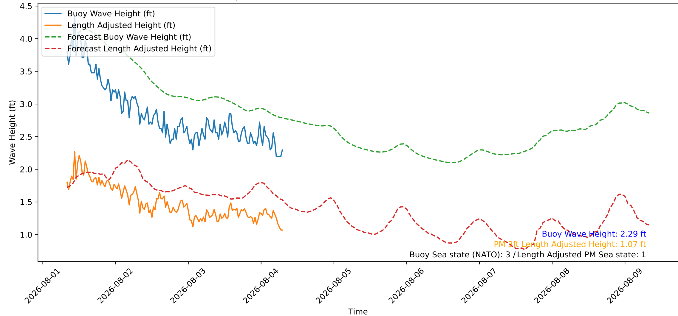
Wave Heights over Time for Oceanside Harbor at 2026-08-04 07:50:27
