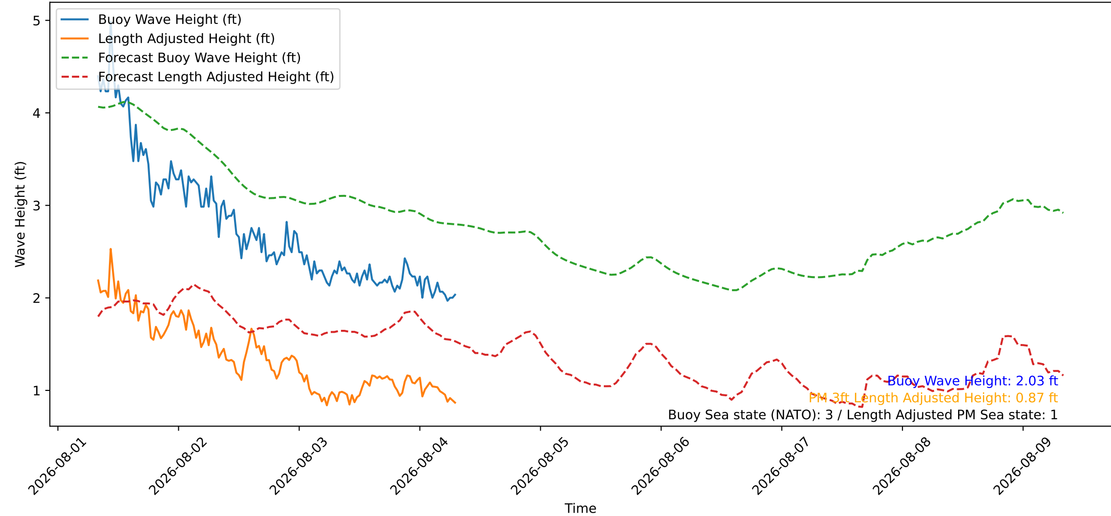
Wave Heights over Time for Green Beach at 2026-08-04 07:51:09
