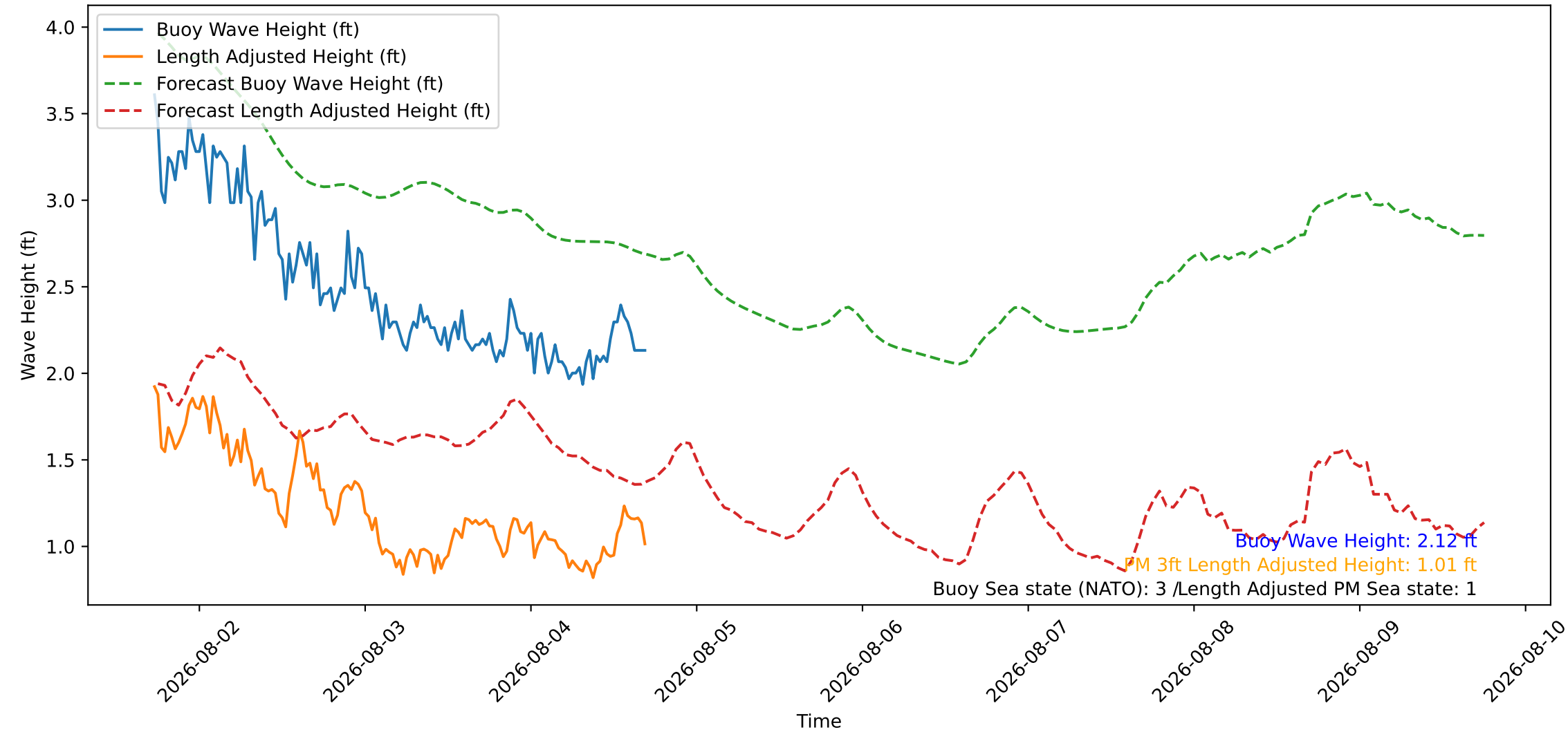
Wave Heights over Time for Green Beach at 2026-08-04 17:31:08
