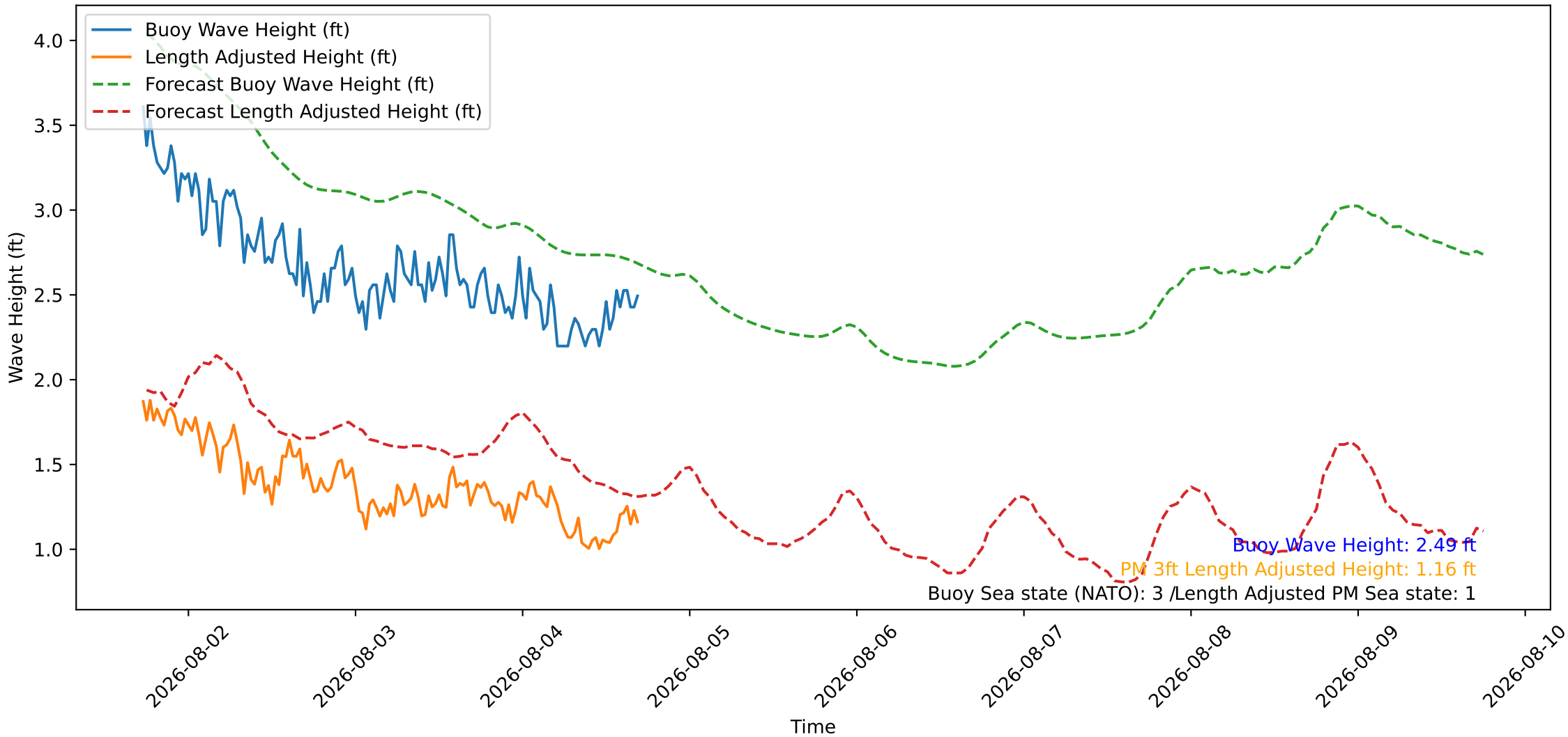
Wave Heights over Time for Oceanside Harbor at 2026-08-04 17:30:27
