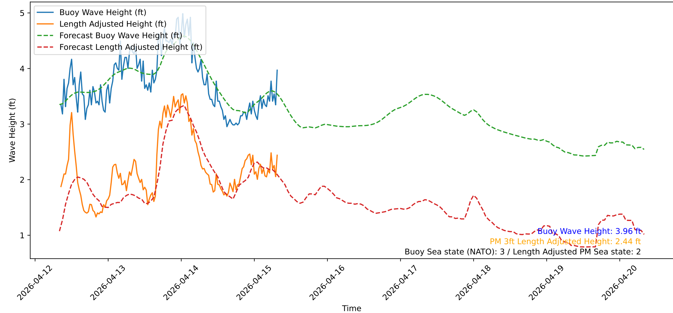
Wave Heights over Time for Green Beach at 2026-04-15 08:21:14
