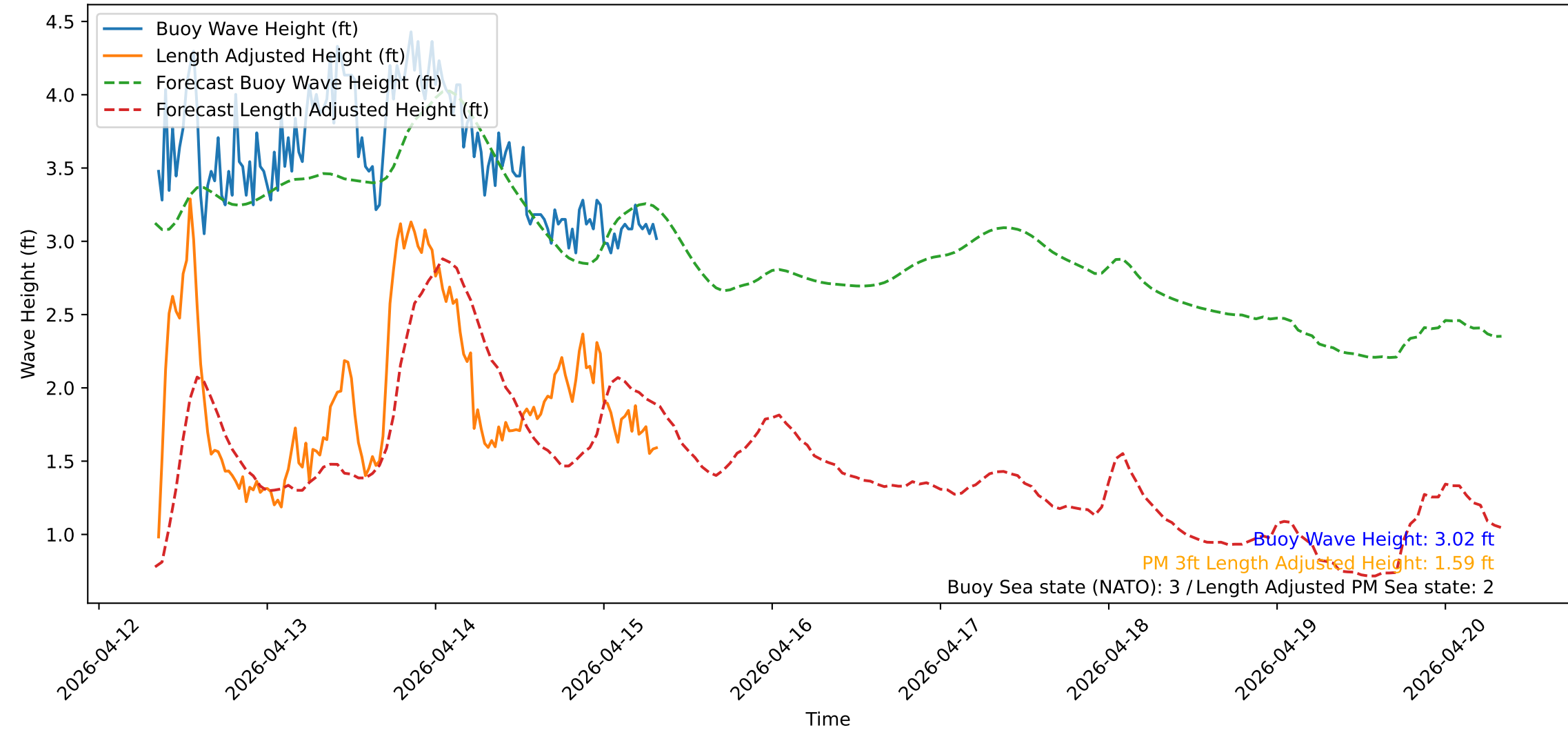
Wave Heights over Time for Red Beach at 2026-04-15 08:20:51
