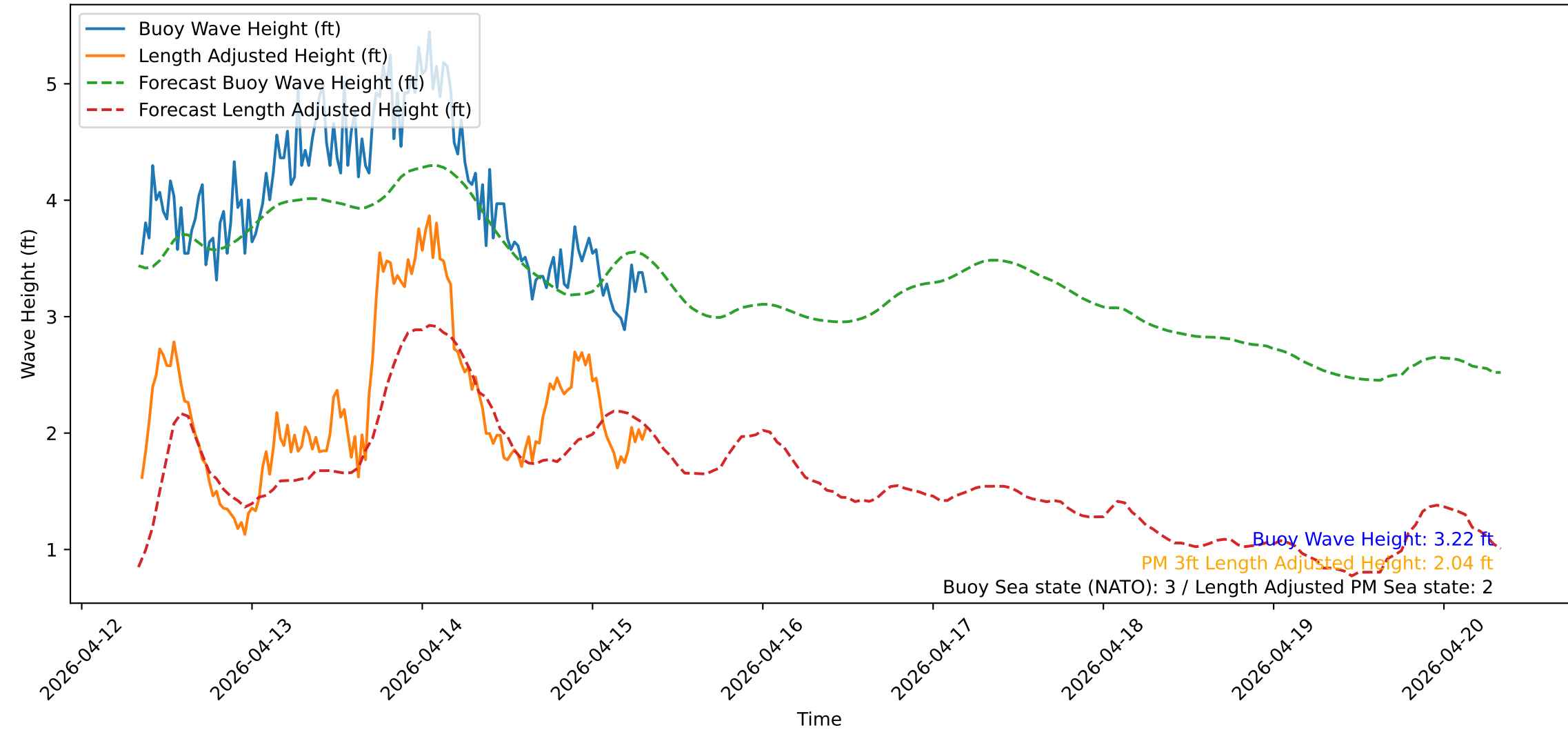
Wave Heights over Time for Oceanside Harbor at 2026-04-15 08:20:31
