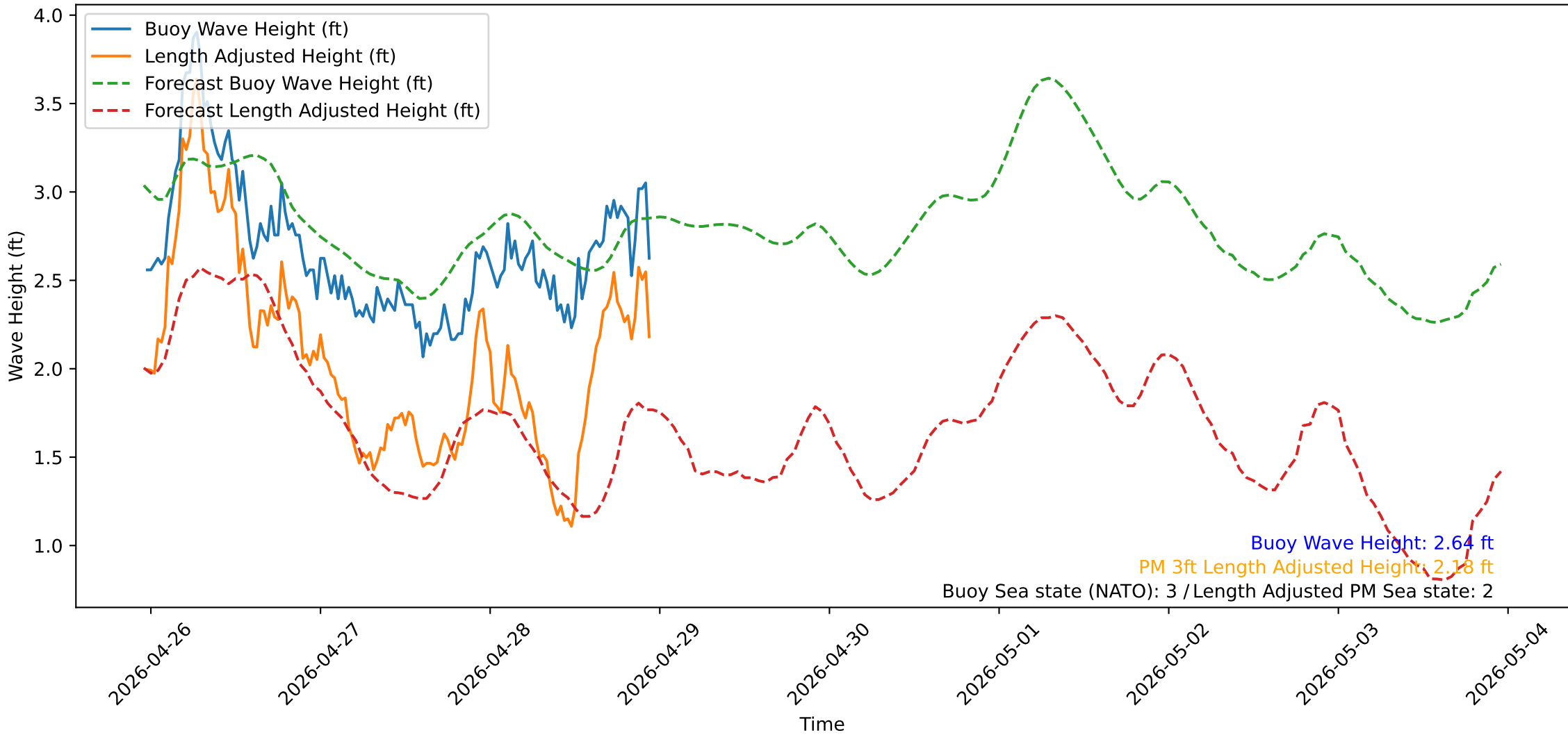
Wave Heights over Time for Oceanside Harbor at 2026-04-28 23:20:32
