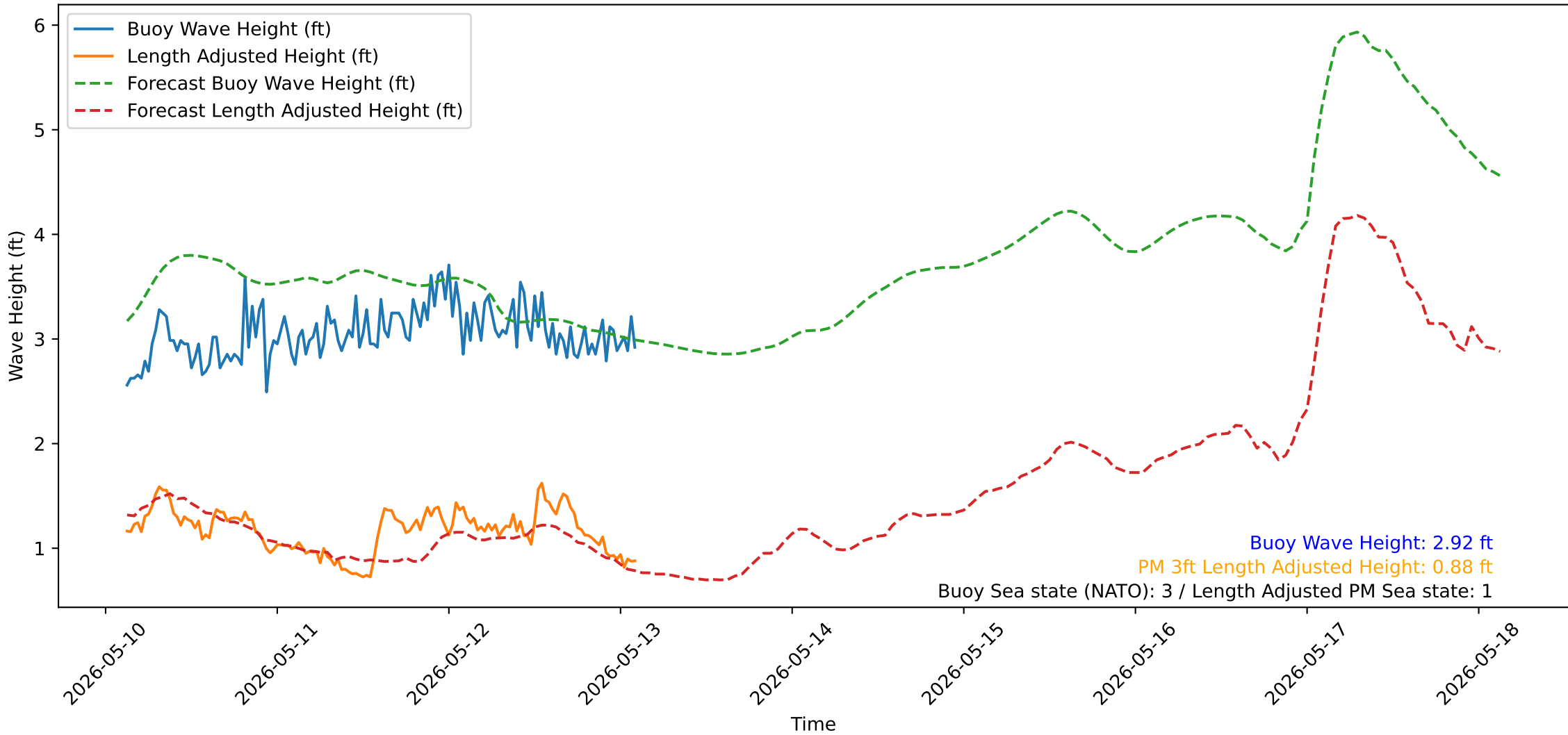
Wave Heights over Time for Oceanside Harbor at 2026-05-13 03:00:31
