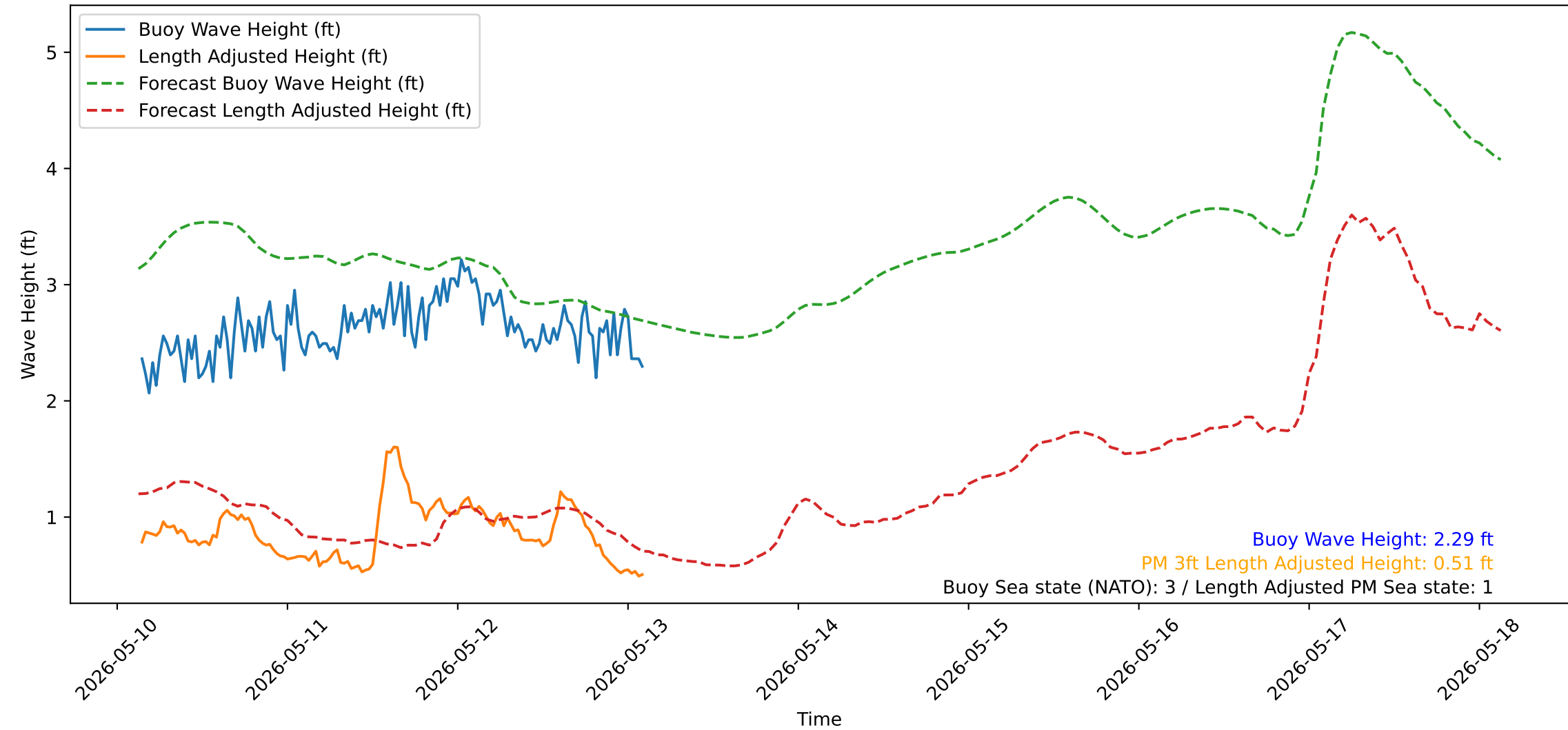
Wave Heights over Time for Red Beach at 2026-05-13 03:00:50
