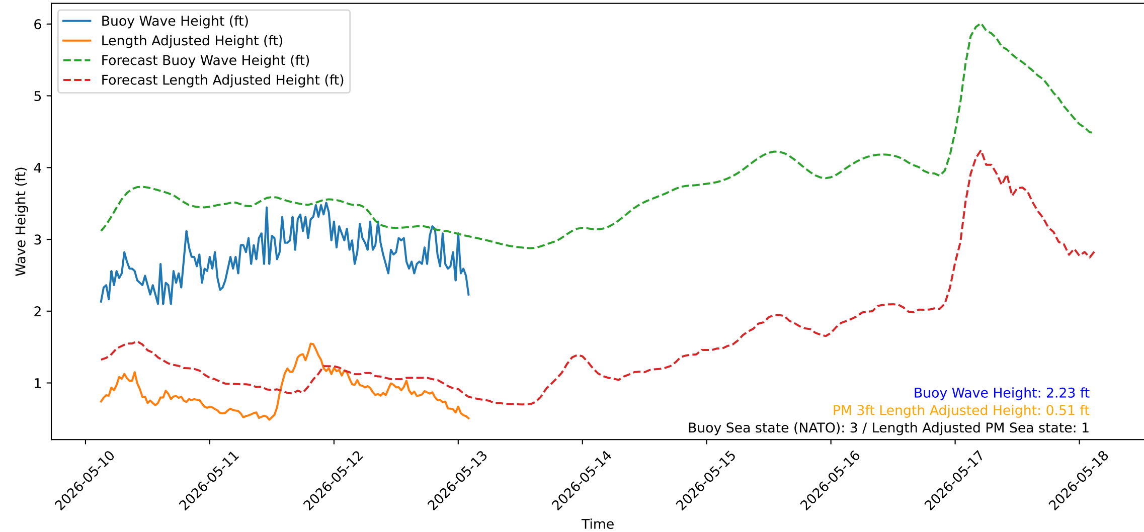
Wave Heights over Time for Green Beach at 2026-05-13 03:01:12
