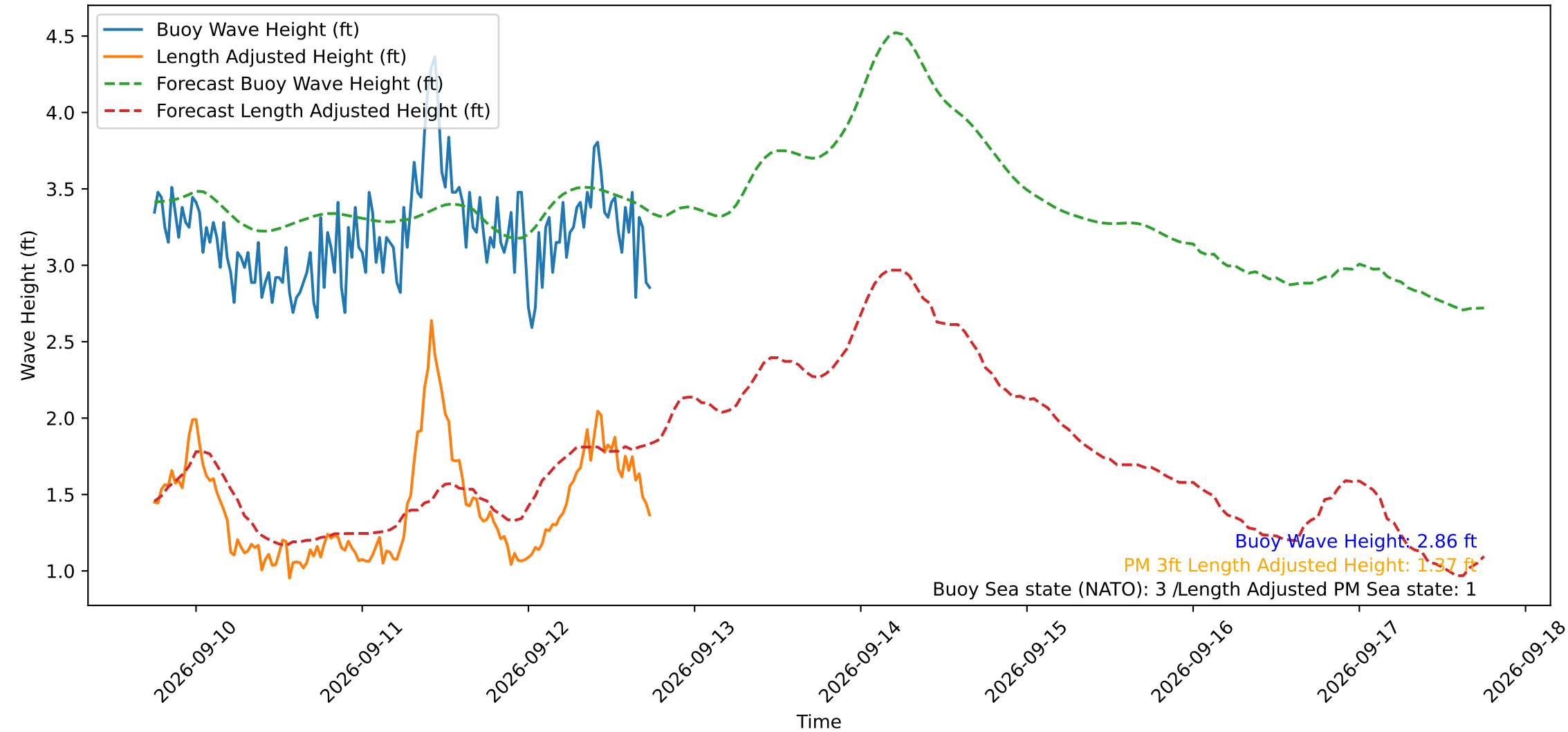
Wave Heights over Time for Oceanside Harbor at 2026-09-12 18:10:29
