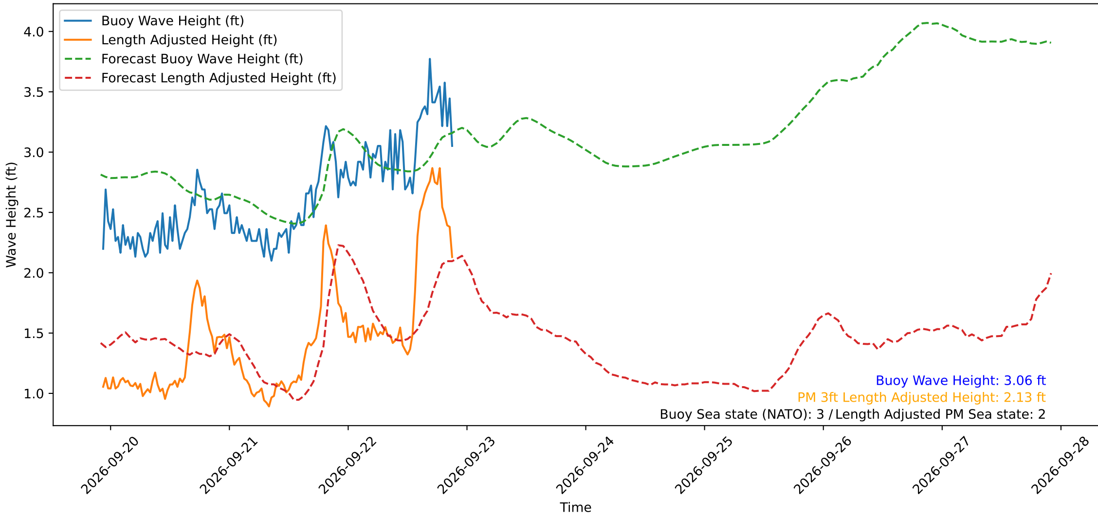
Wave Heights over Time for Oceanside Harbor at 2026-09-22 22:20:29
