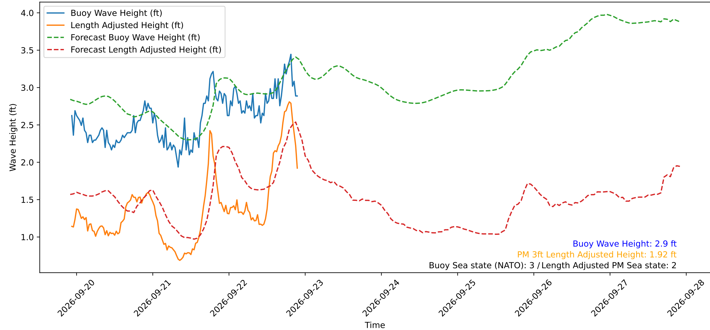
Wave Heights over Time for Green Beach at 2026-09-22 22:21:14
