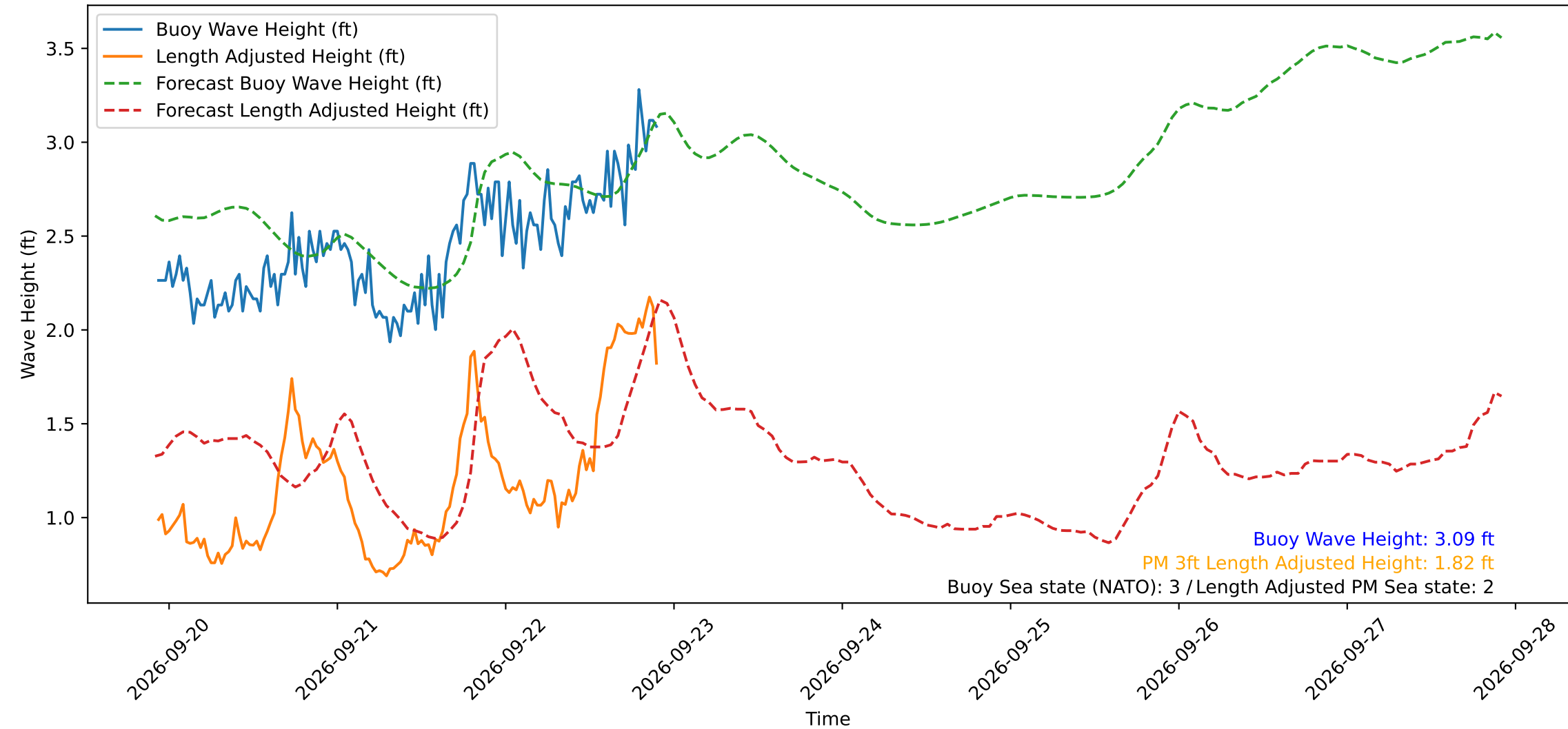
Wave Heights over Time for Red Beach at 2026-09-22 22:20:50
