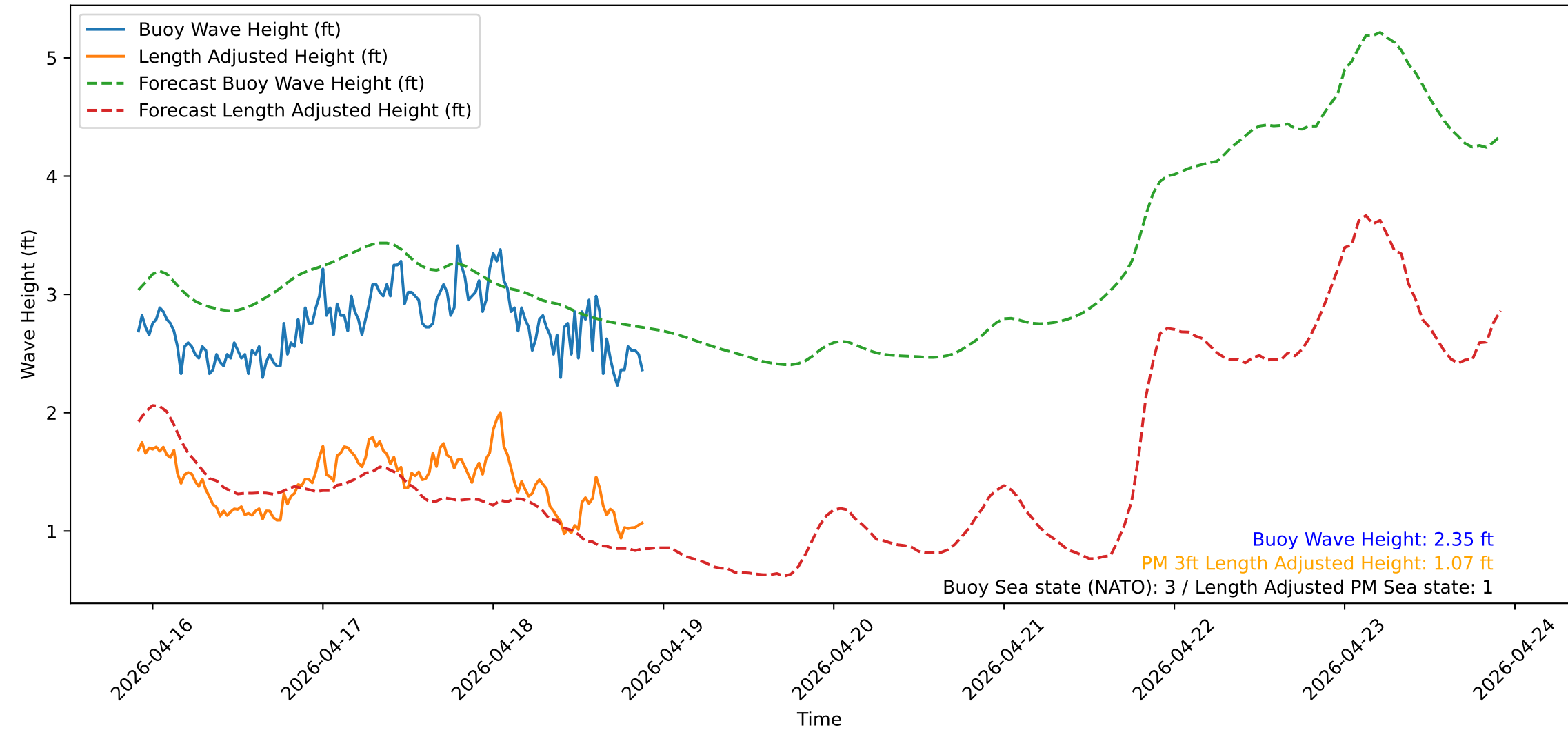
Wave Heights over Time for Oceanside Harbor at 2026-04-18 22:10:31
