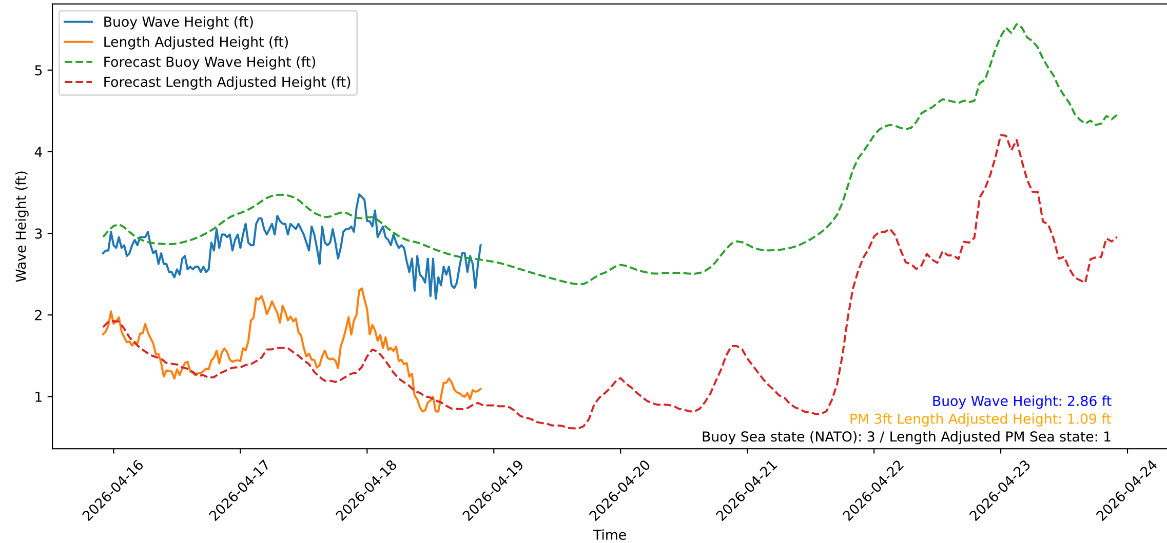
Wave Heights over Time for Green Beach at 2026-04-18 22:11:12
