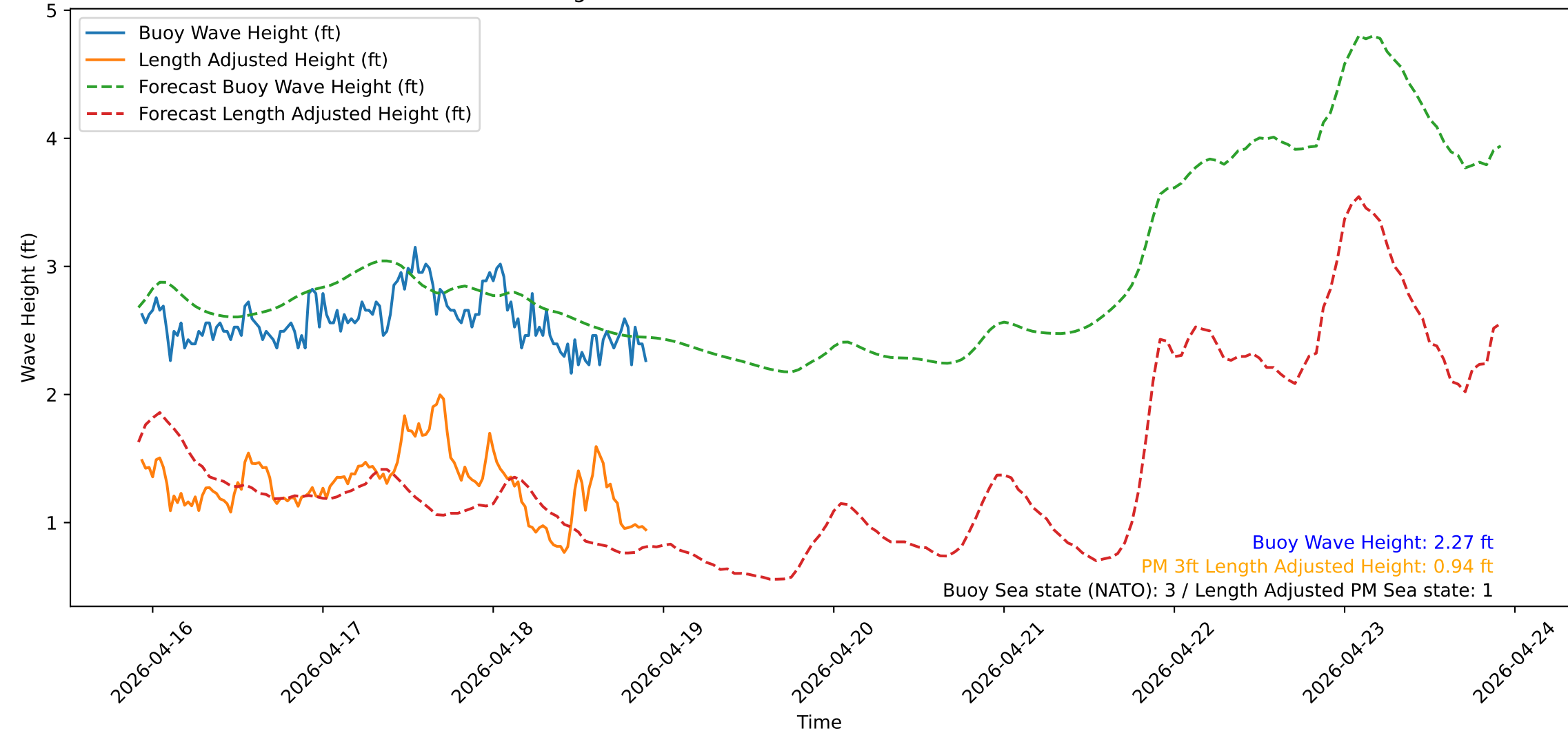
Wave Heights over Time for Red Beach at 2026-04-18 22:10:50
