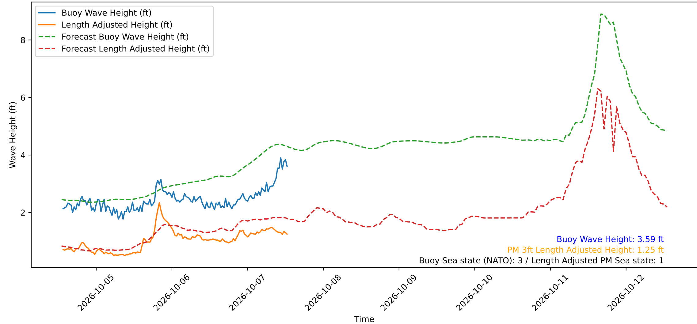
Wave Heights over Time for Green Beach at 2026-10-07 13:21:15
