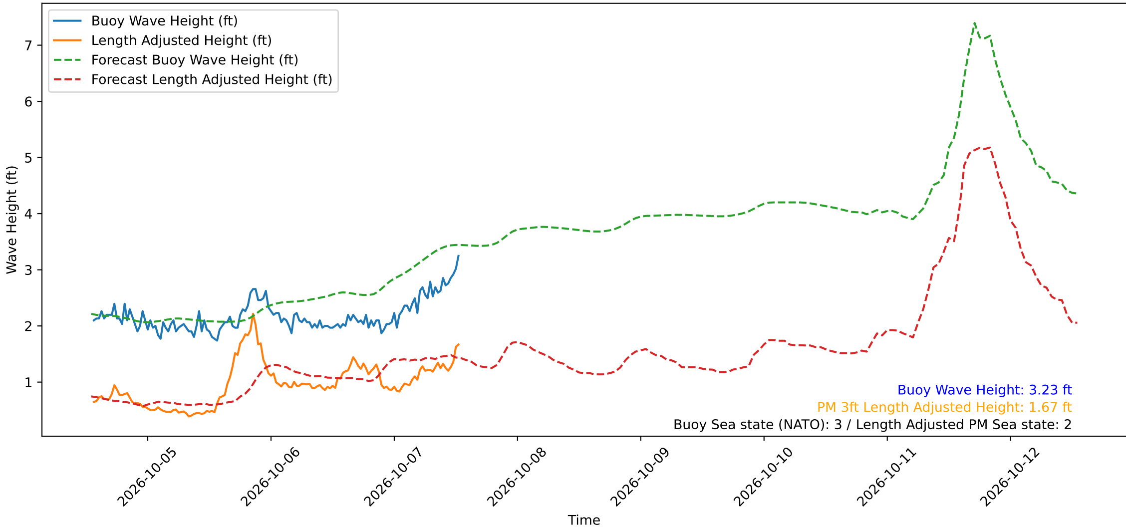
Wave Heights over Time for Red Beach at 2026-10-07 13:20:51
