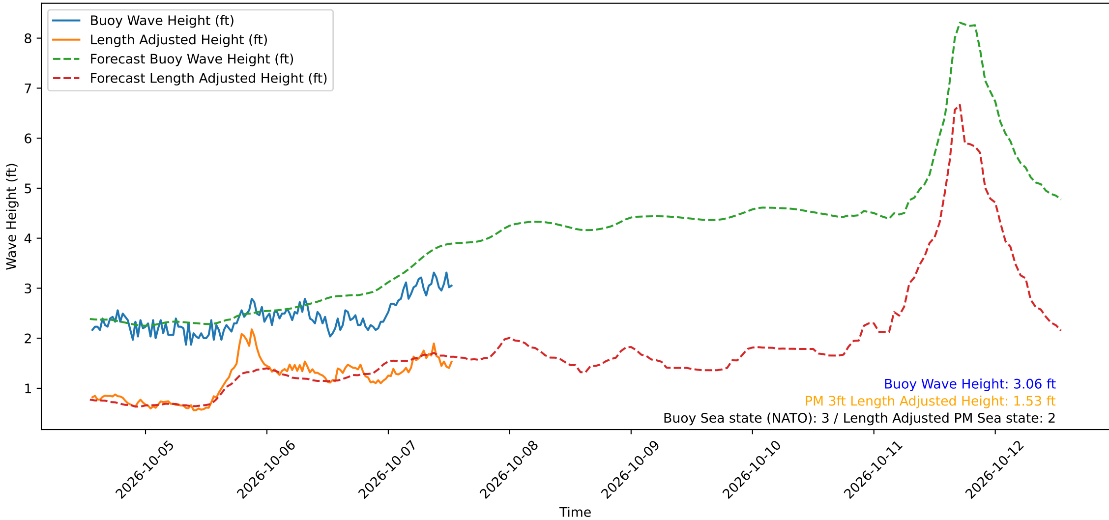
Wave Heights over Time for Oceanside Harbor at 2026-10-07 13:20:30
