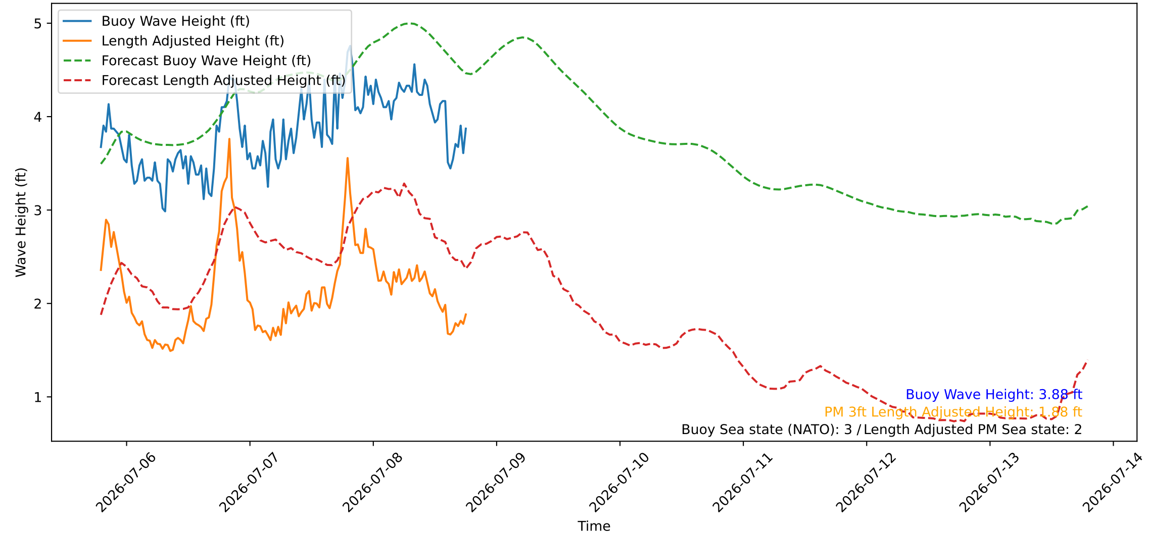
Wave Heights over Time for Green Beach at 2026-07-08 19:01:09
