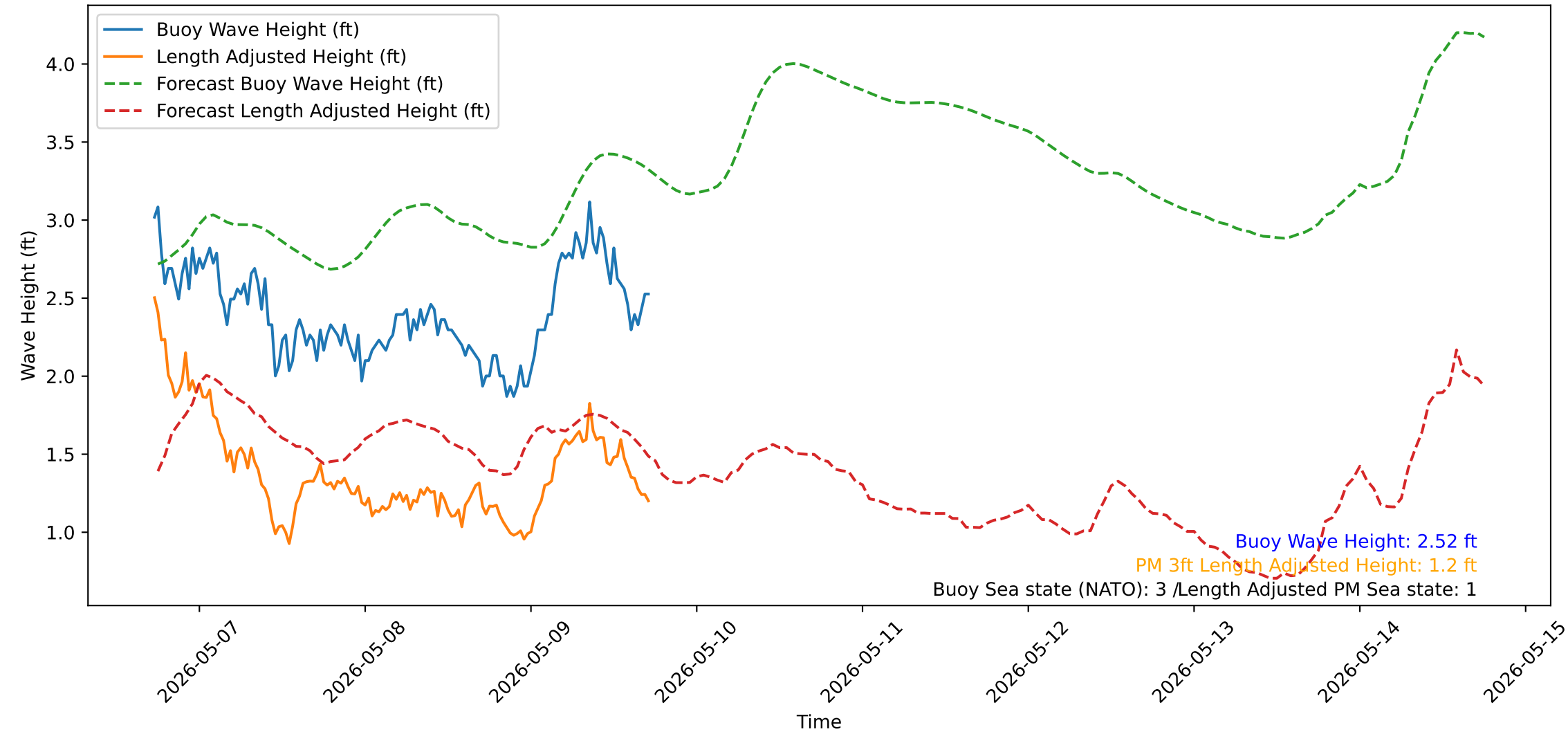
Wave Heights over Time for Oceanside Harbor at 2026-05-09 17:40:33
