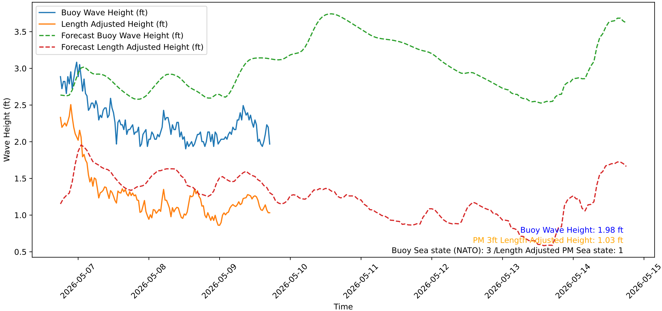
Wave Heights over Time for Red Beach at 2026-05-09 17:40:54
