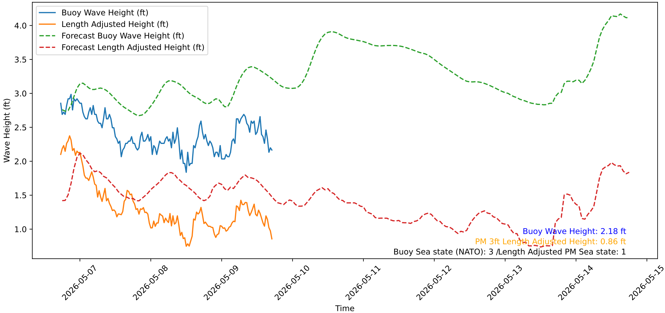
Wave Heights over Time for Green Beach at 2026-05-09 17:41:18
