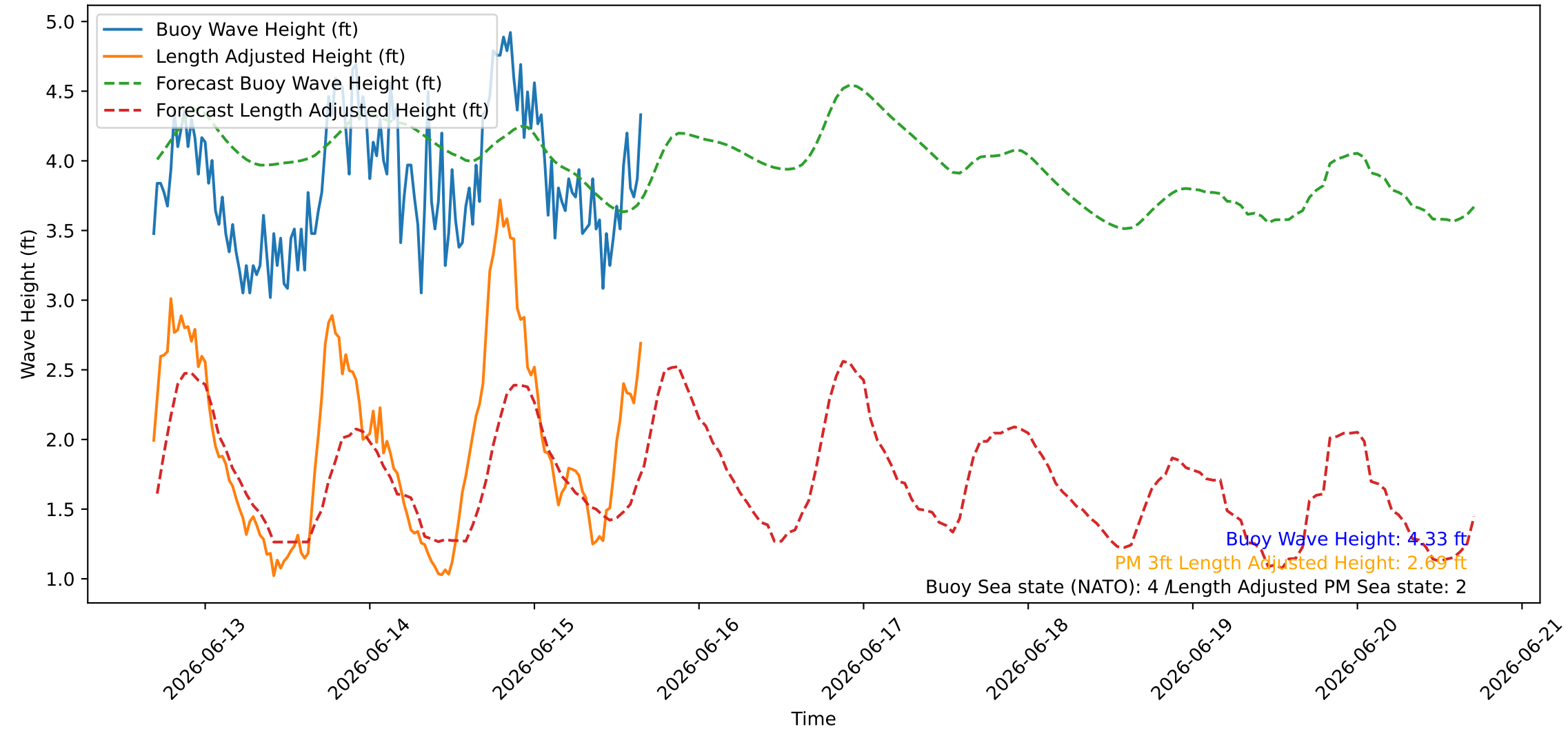
Wave Heights over Time for Green Beach at 2026-06-15 16:31:07
