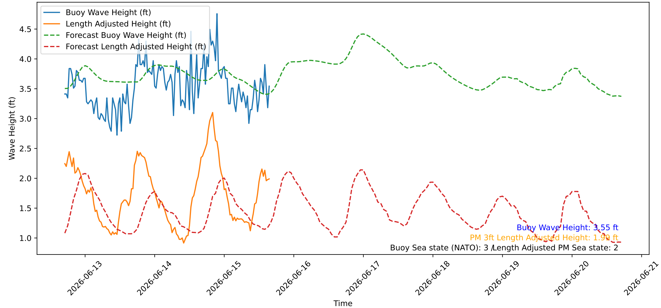
Wave Heights over Time for Red Beach at 2026-06-15 16:30:45
