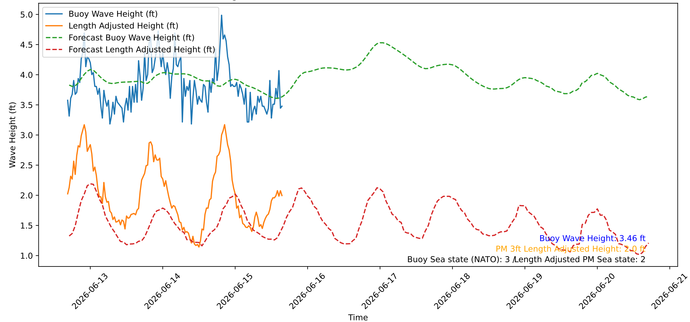
Wave Heights over Time for Oceanside Harbor at 2026-06-15 16:30:25
