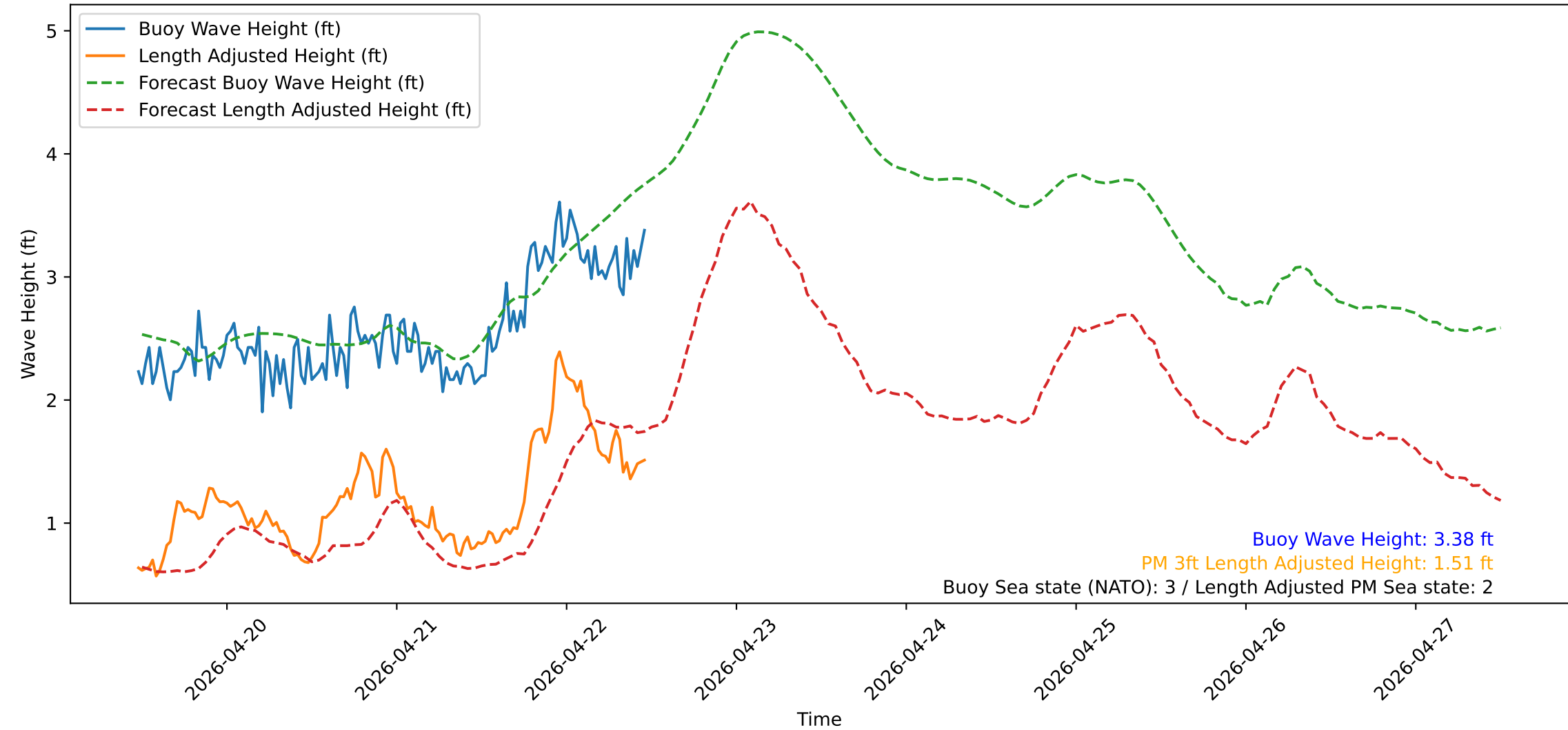
Wave Heights over Time for Oceanside Harbor at 2026-04-22 11:30:31
