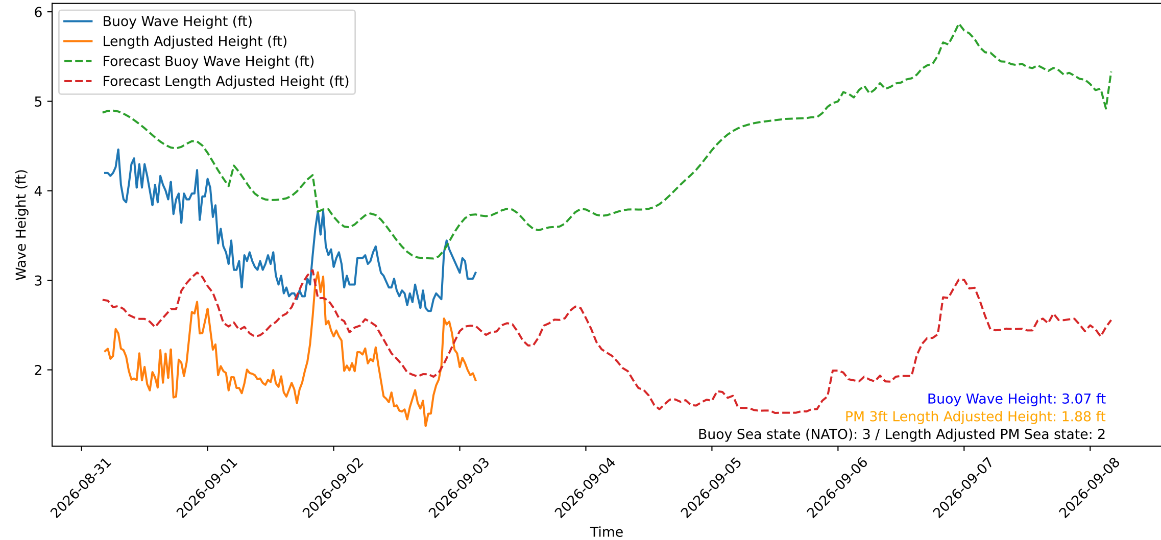
Wave Heights over Time for Green Beach at 2026-09-03 04:01:12
