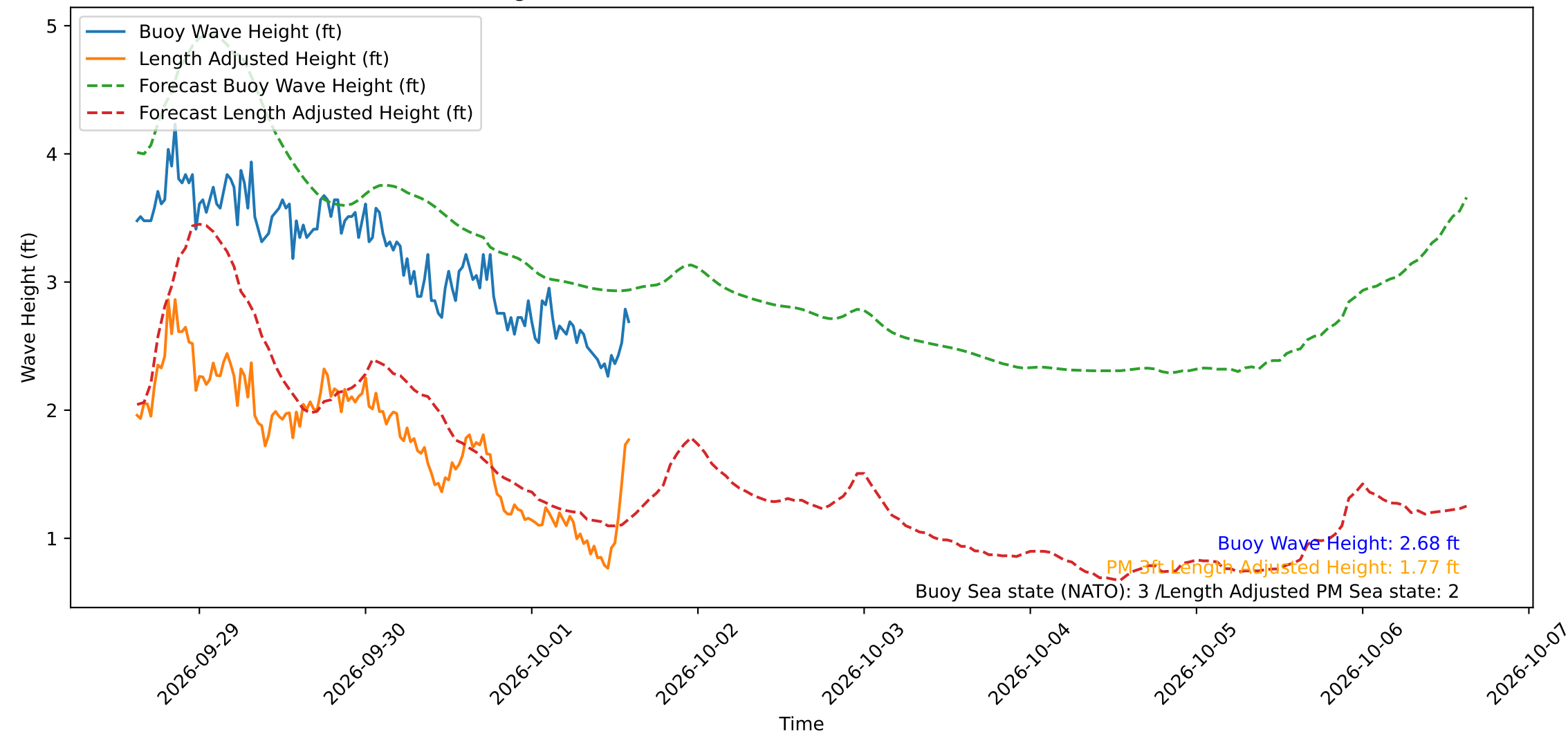
Wave Heights over Time for Oceanside Harbor at 2026-10-01 14:50:29
