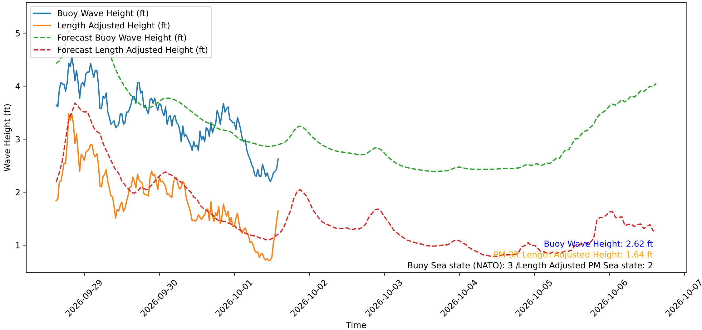
Wave Heights over Time for Green Beach at 2026-10-01 14:51:15
