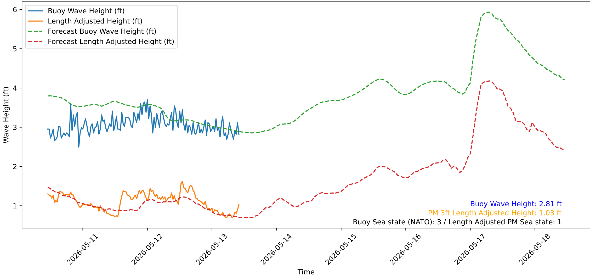
Wave Heights over Time for Oceanside Harbor at 2026-05-13 11:00:31
