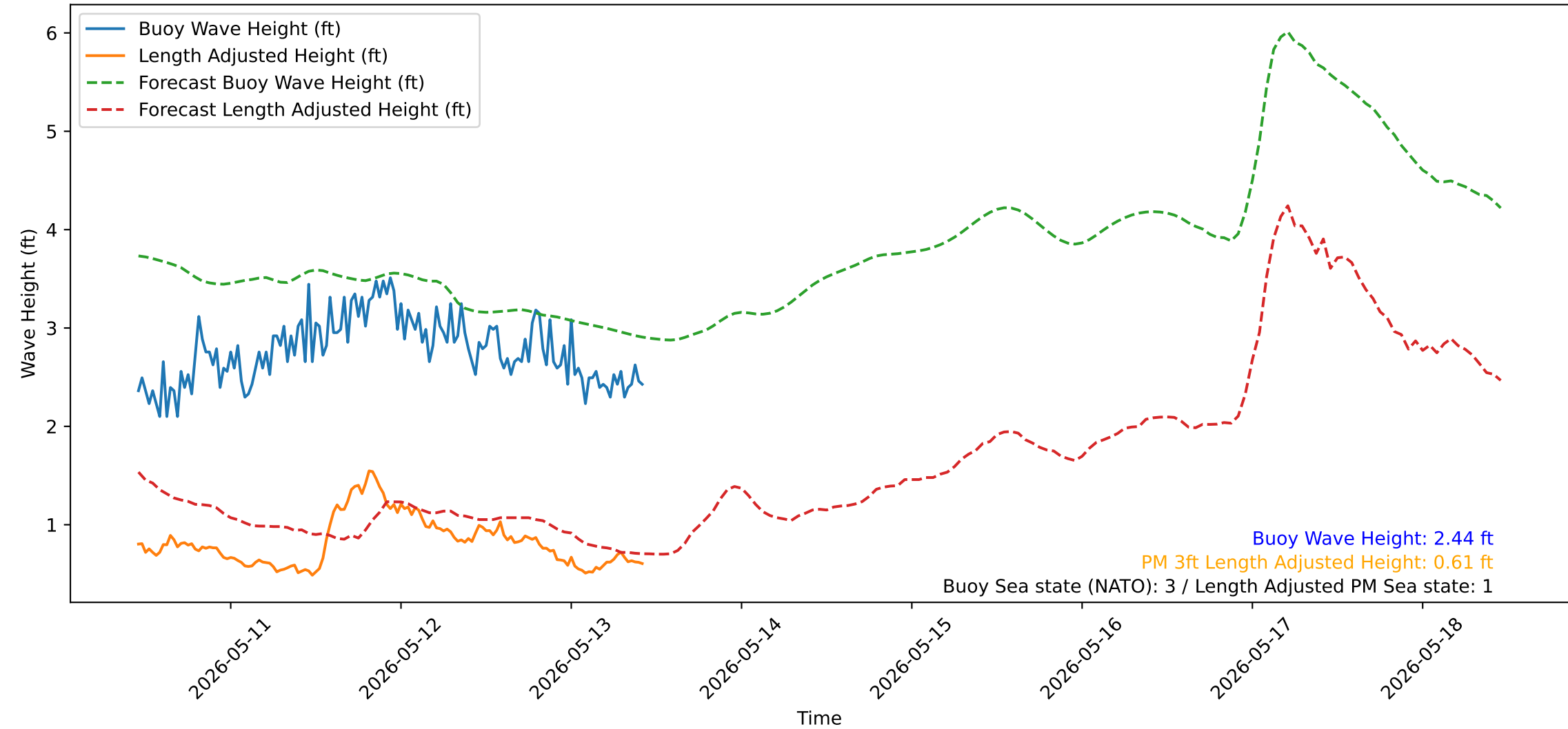
Wave Heights over Time for Green Beach at 2026-05-13 11:01:13
