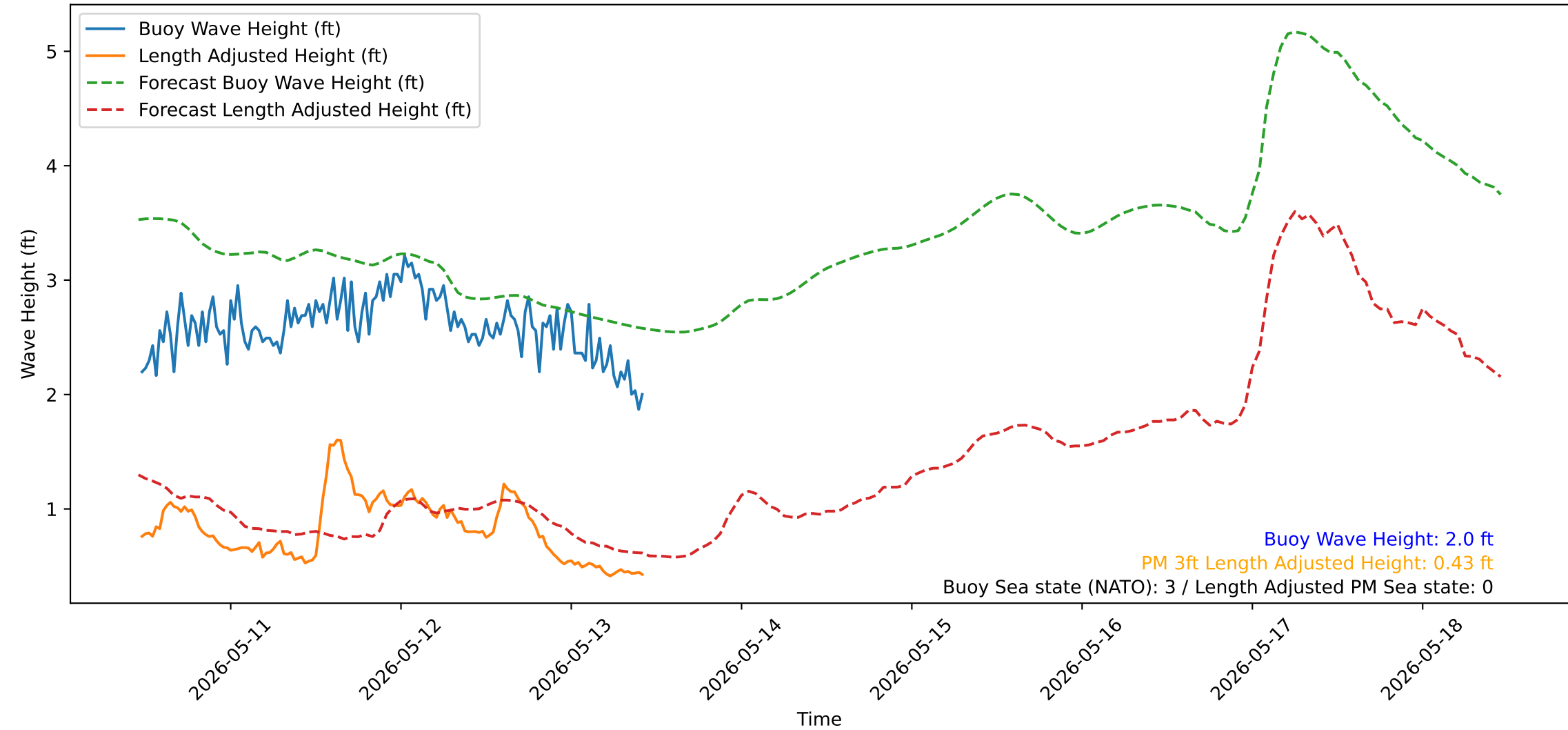
Wave Heights over Time for Red Beach at 2026-05-13 11:00:51
