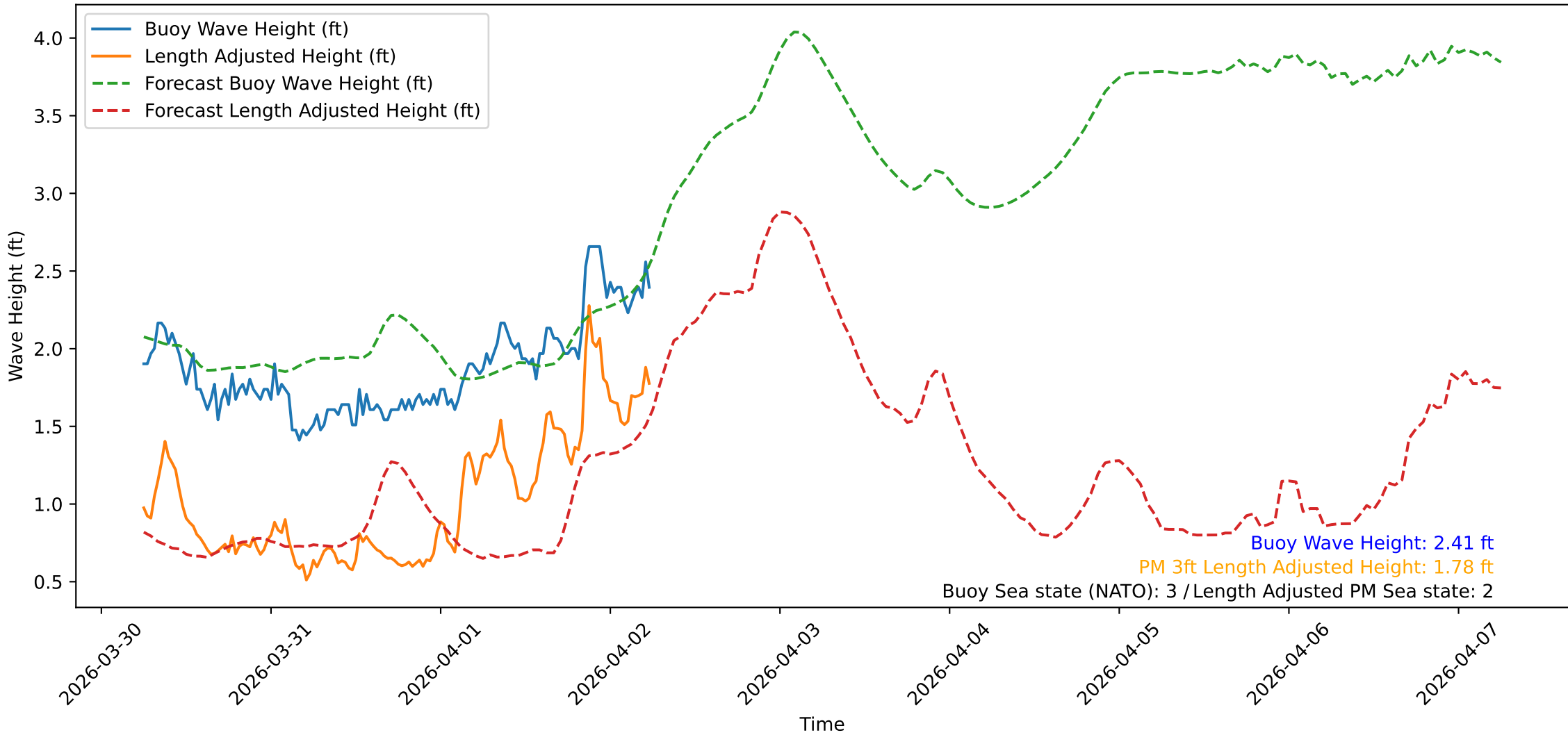
Wave Heights over Time for Green Beach at 2026-04-02 06:11:10
