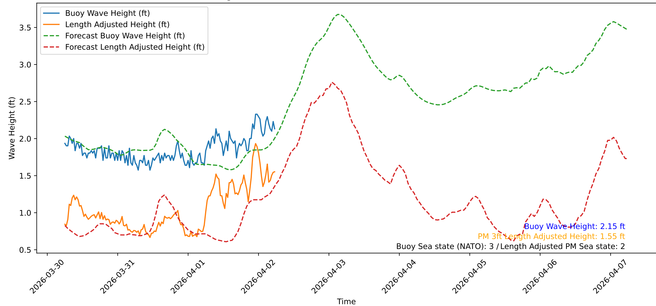
Wave Heights over Time for Oceanside Harbor at 2026-04-02 06:10:32
