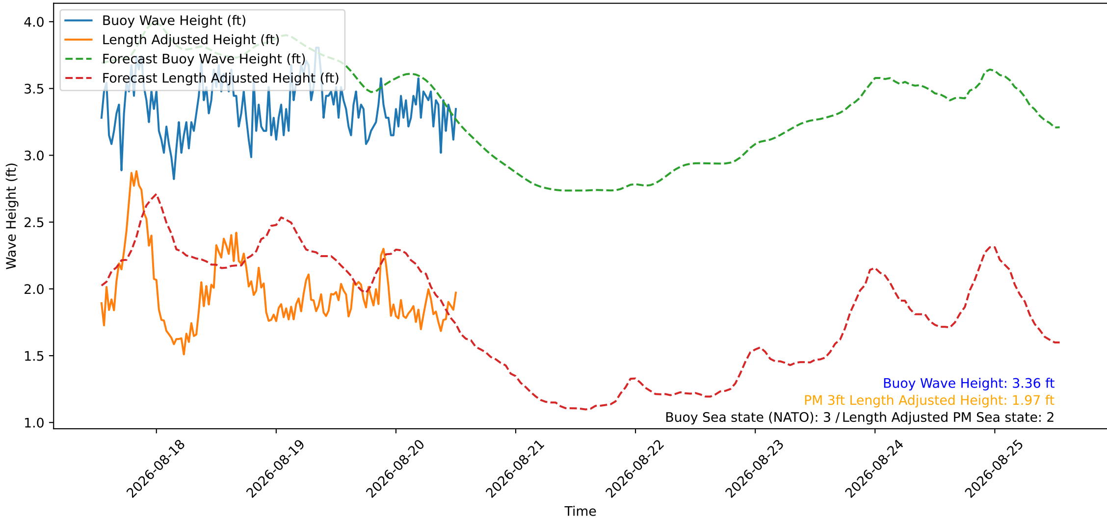
Wave Heights over Time for Oceanside Harbor at 2026-08-20 12:50:26
