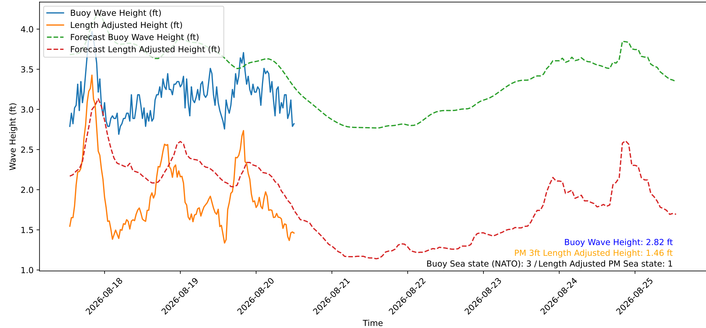
Wave Heights over Time for Green Beach at 2026-08-20 12:51:11
