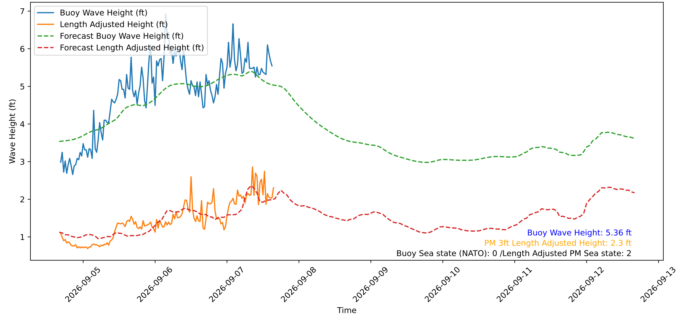
Wave Heights over Time for Red Beach at 2026-09-07 16:20:51
