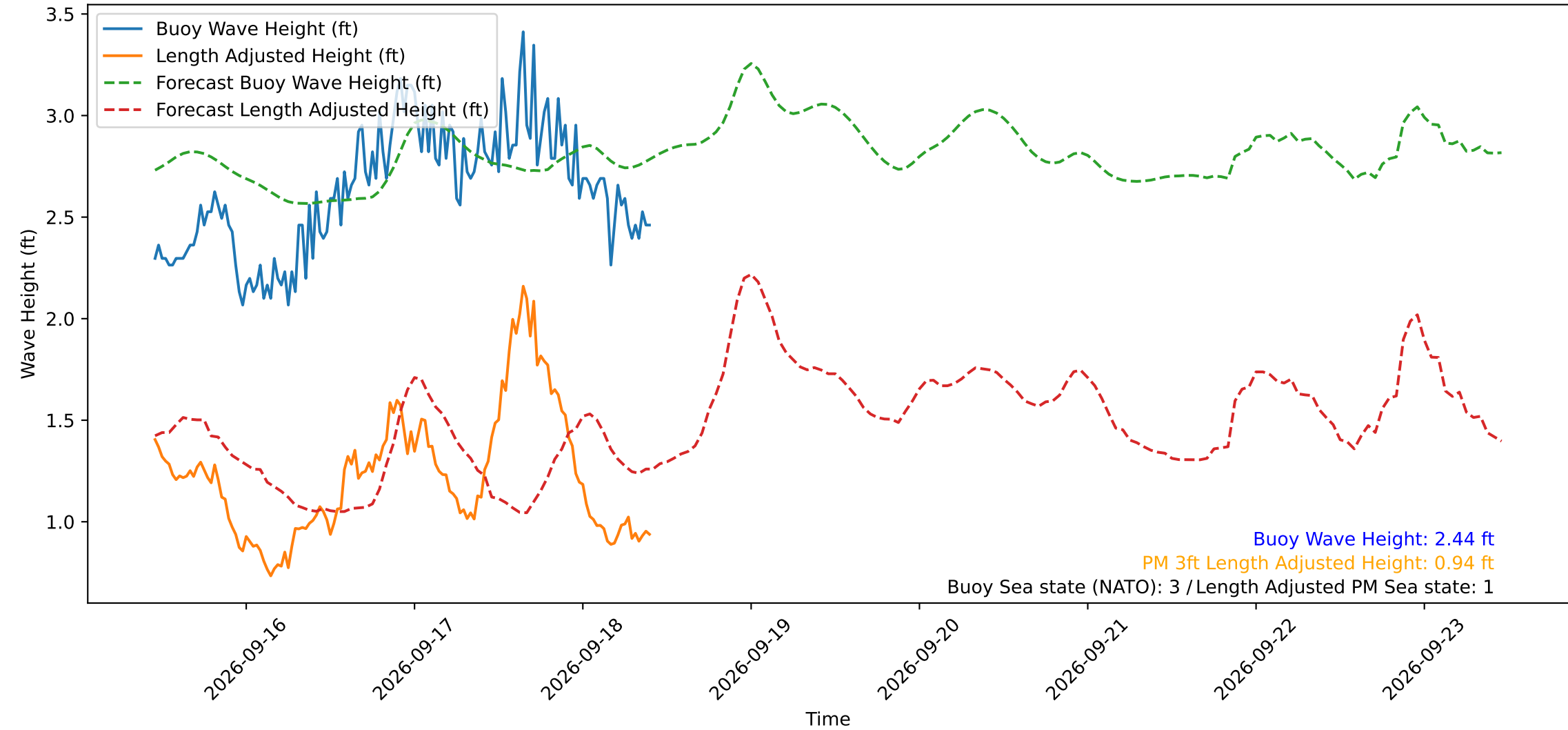
Wave Heights over Time for Red Beach at 2026-09-18 10:30:54
