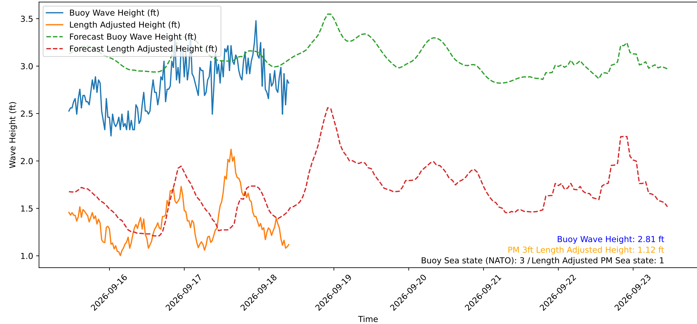
Wave Heights over Time for Green Beach at 2026-09-18 10:31:21
