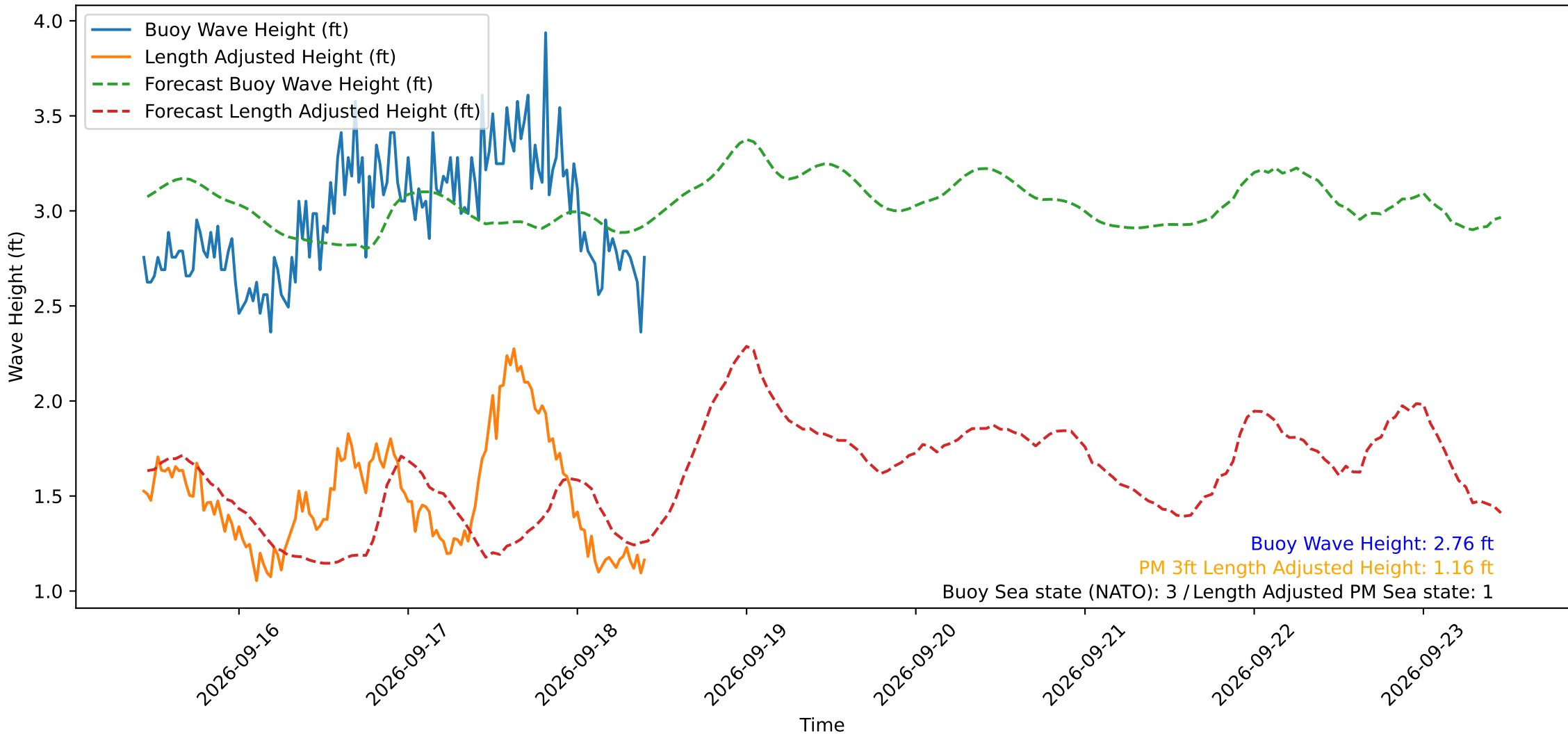
Wave Heights over Time for Oceanside Harbor at 2026-09-18 10:30:32
