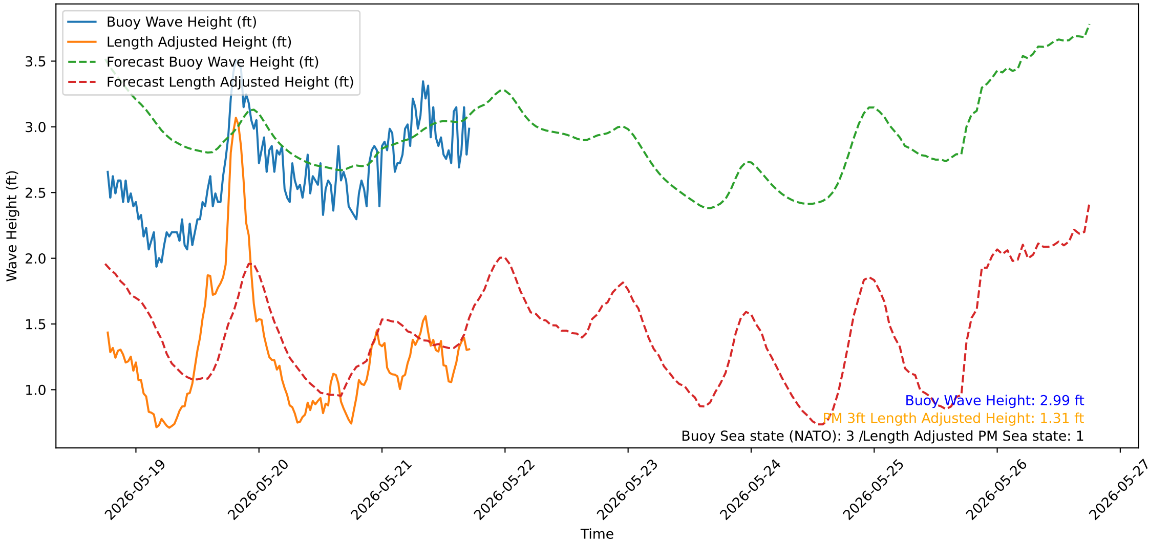
Wave Heights over Time for Red Beach at 2026-05-21 18:00:51
