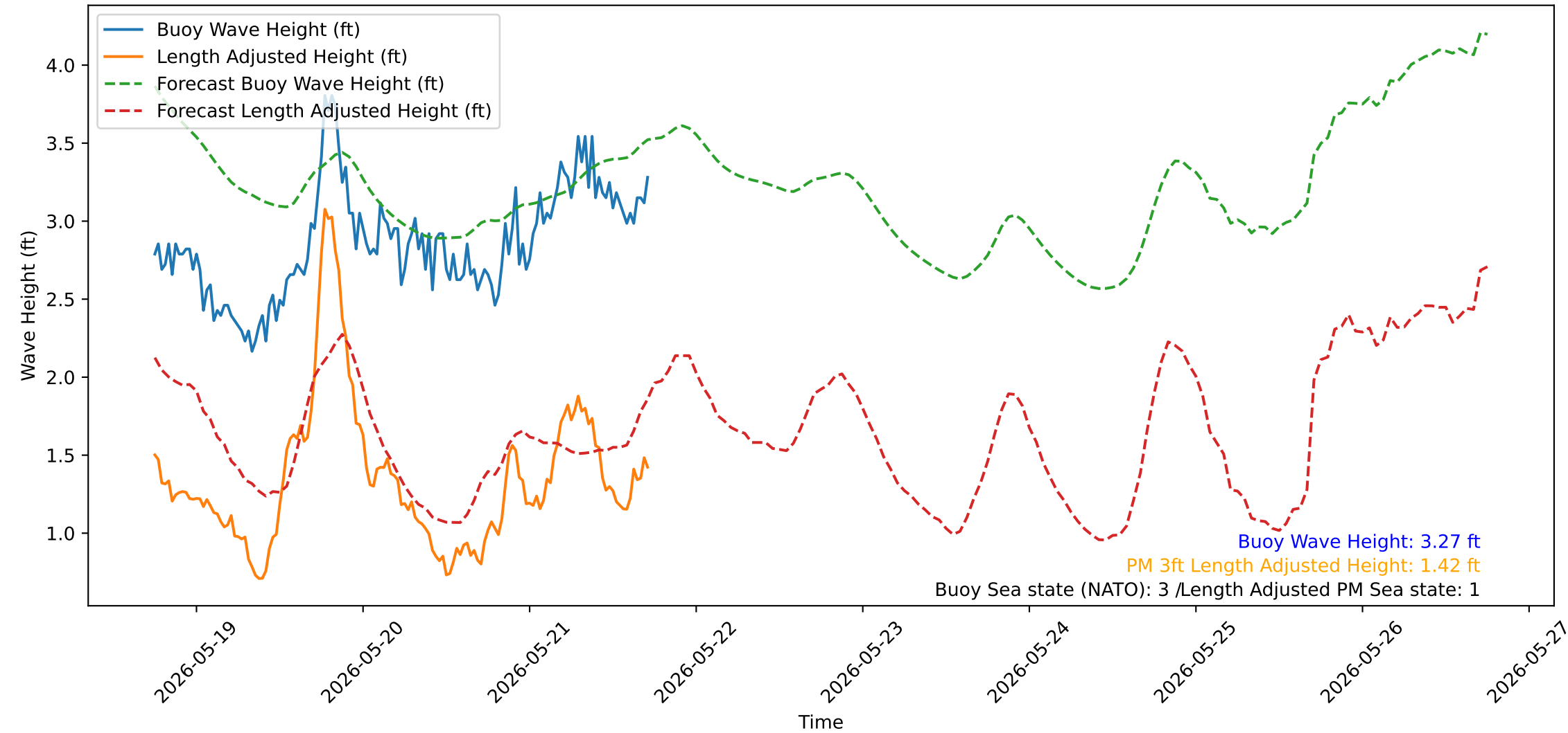
Wave Heights over Time for Green Beach at 2026-05-21 18:01:13
