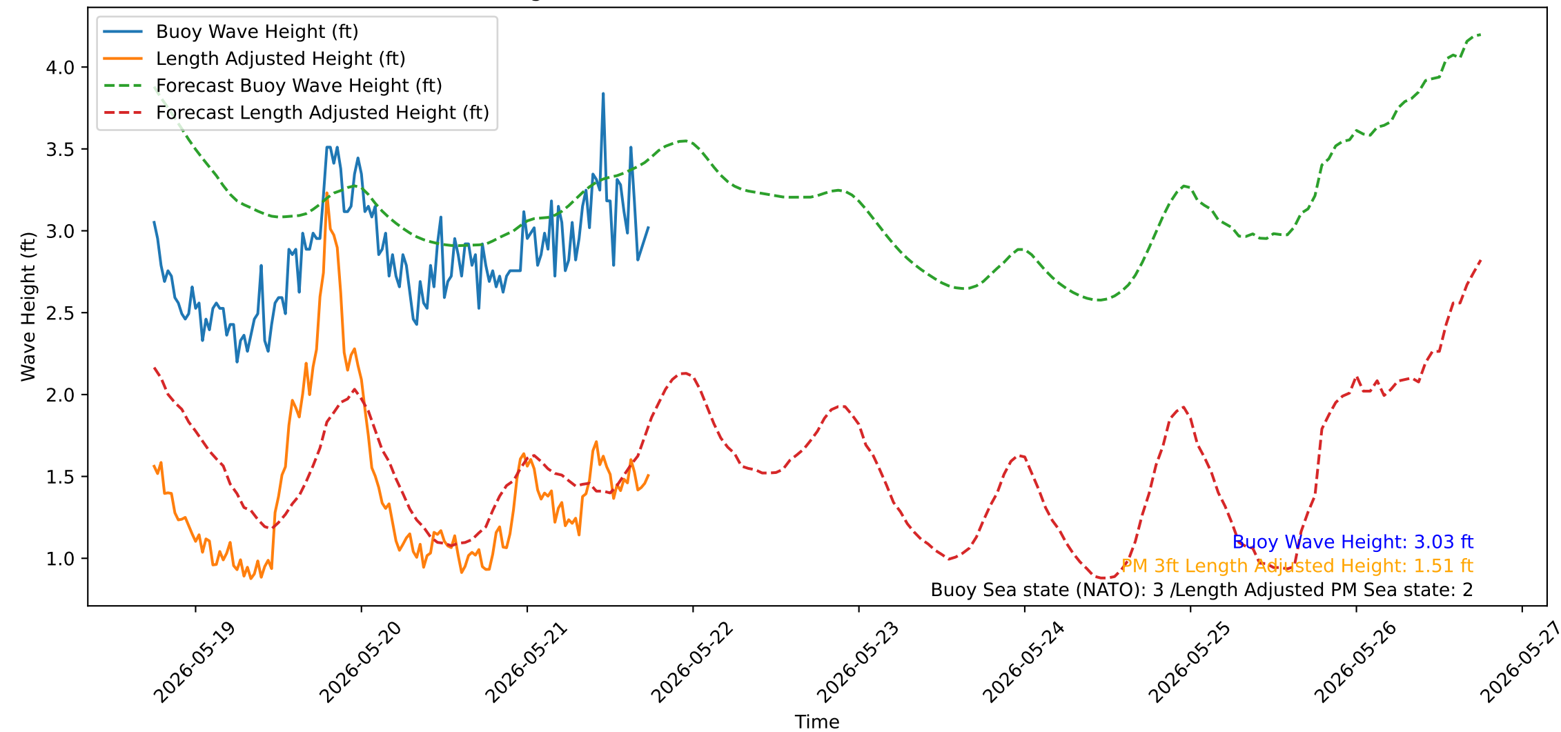
Wave Heights over Time for Oceanside Harbor at 2026-05-21 18:00:31
