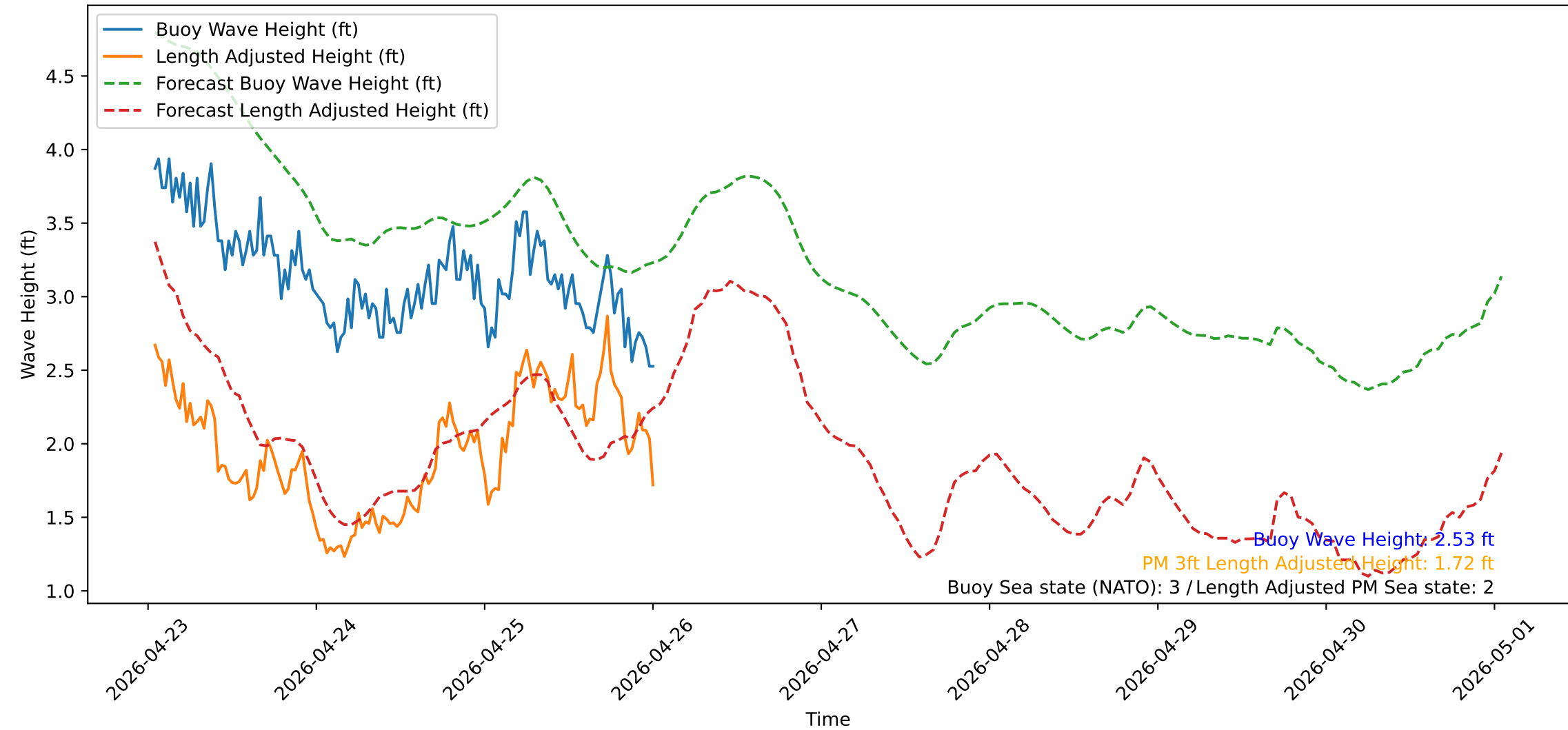
Wave Heights over Time for Green Beach at 2026-04-26 00:51:13
