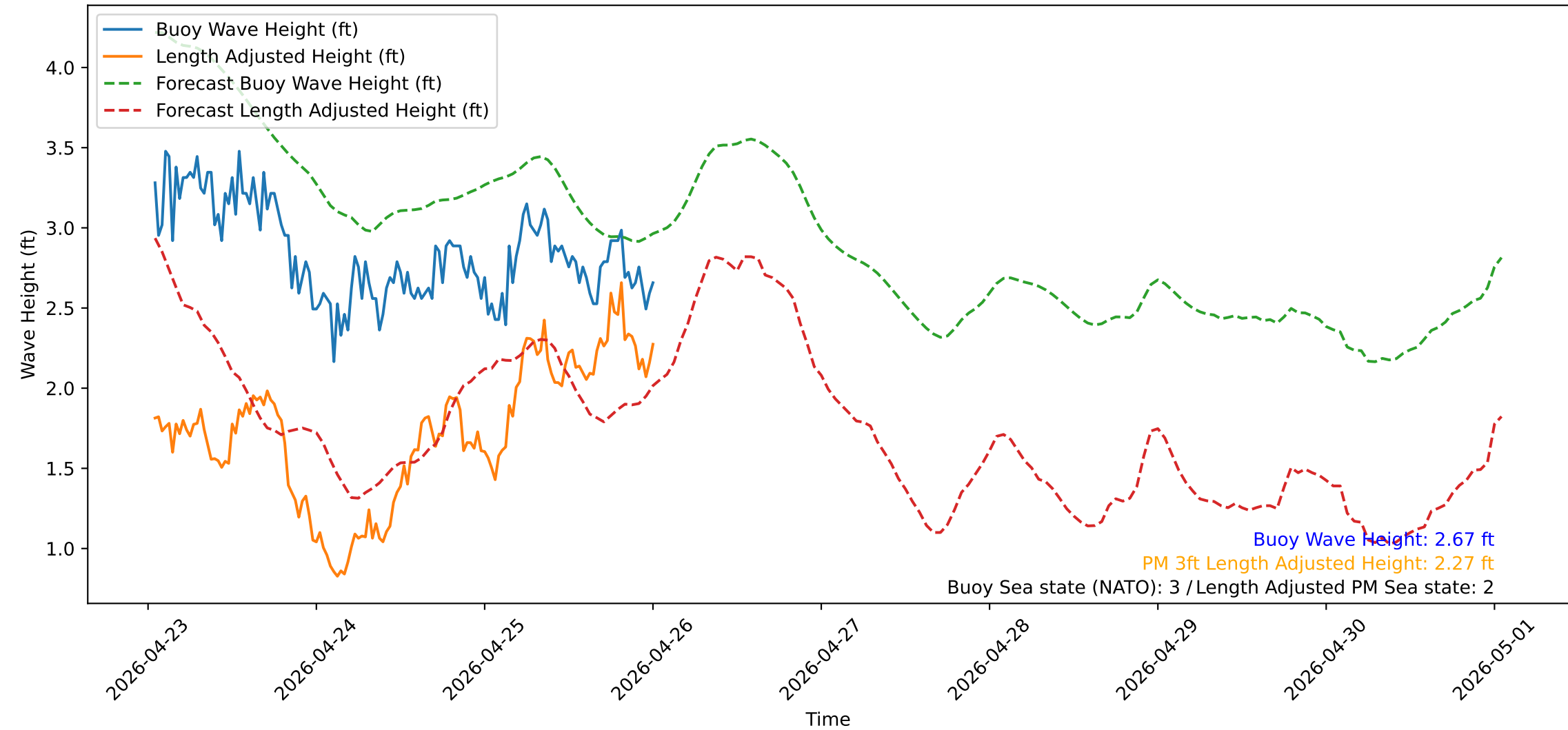
Wave Heights over Time for Red Beach at 2026-04-26 00:50:51
