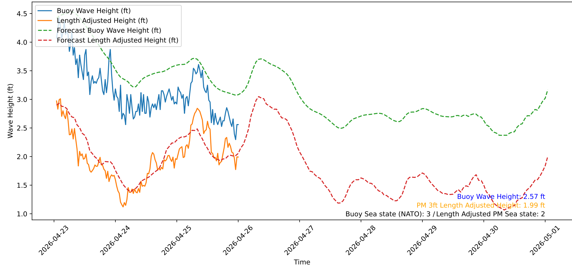
Wave Heights over Time for Oceanside Harbor at 2026-04-26 00:50:31
