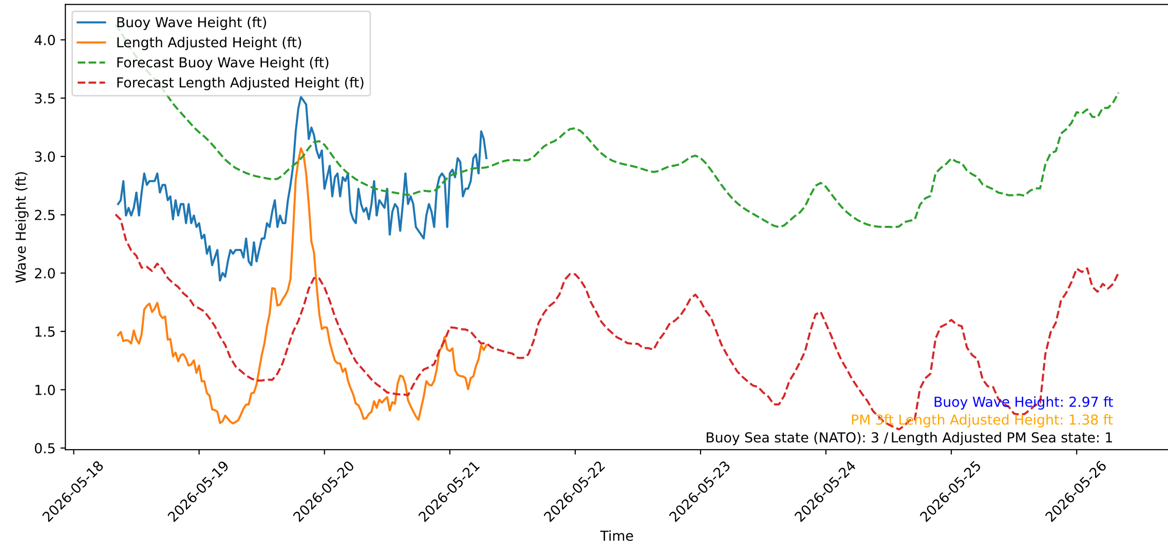
Wave Heights over Time for Red Beach at 2026-05-21 08:00:51
