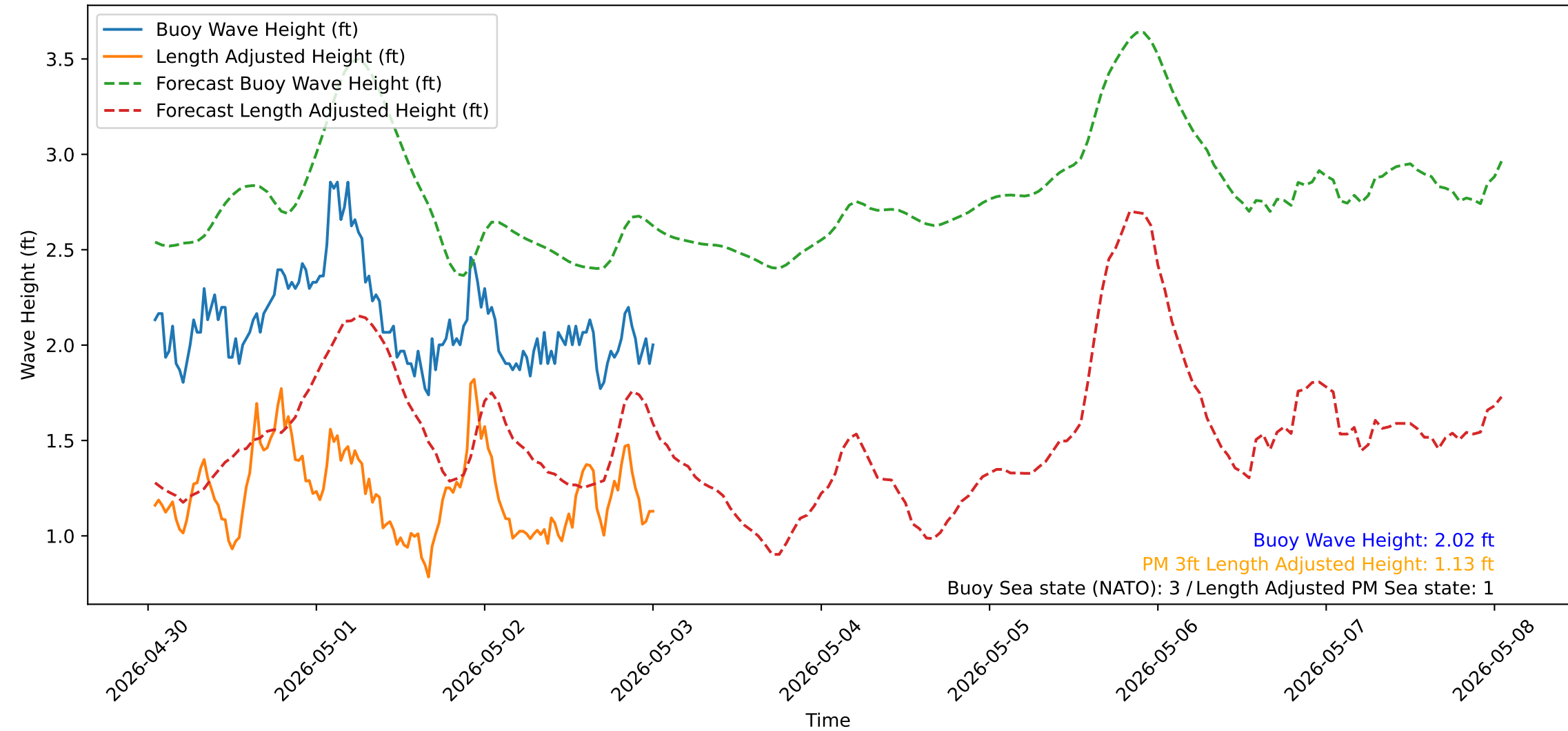
Wave Heights over Time for Green Beach at 2026-05-03 00:51:14
