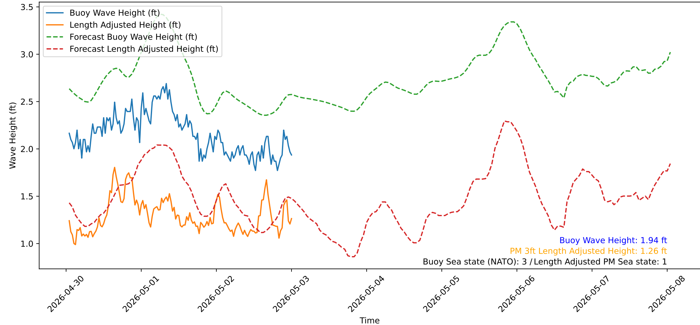
Wave Heights over Time for Oceanside Harbor at 2026-05-03 00:50:31
