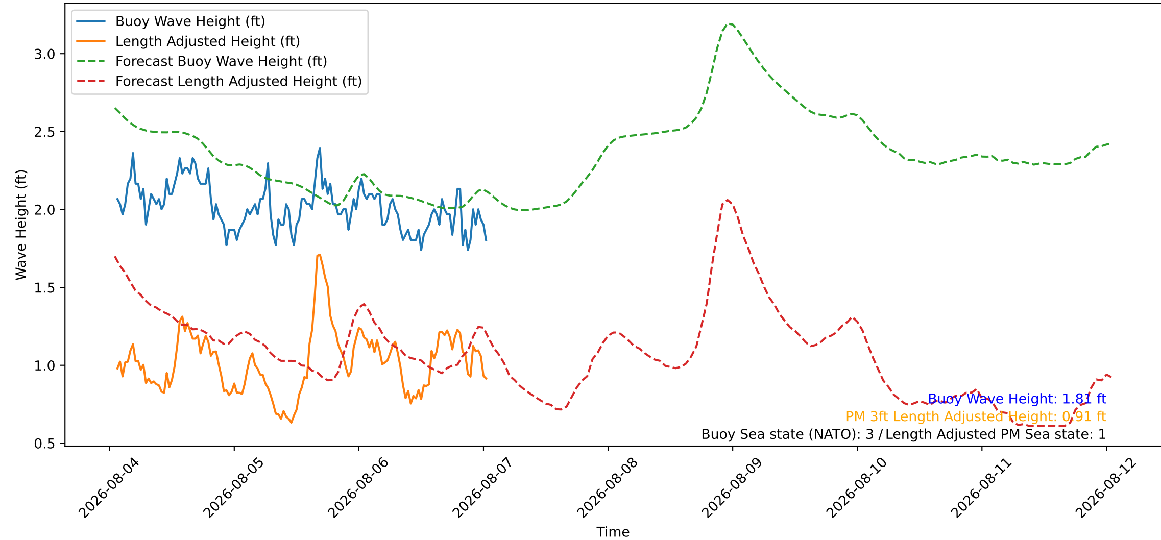
Wave Heights over Time for Red Beach at 2026-08-07 01:20:47
