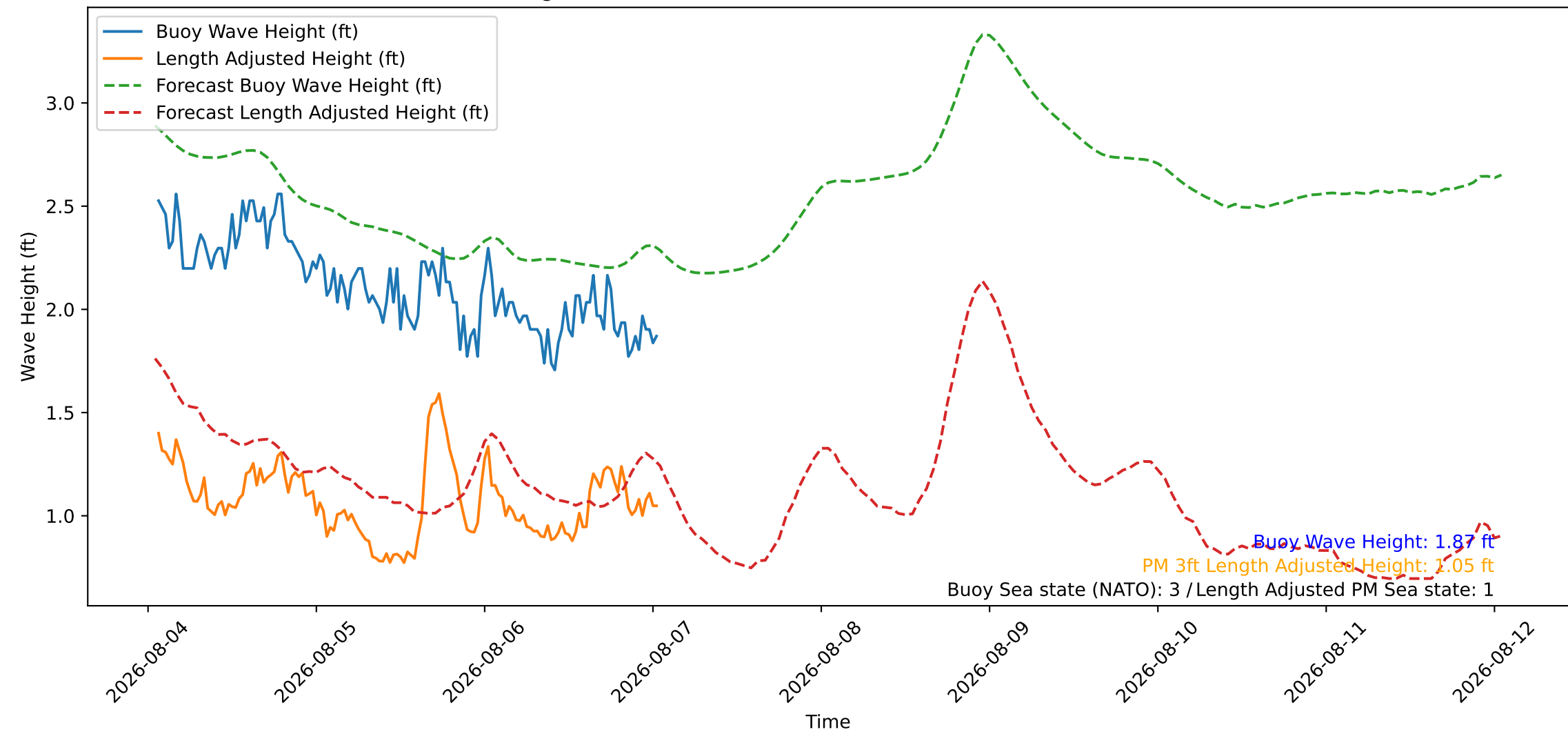
Wave Heights over Time for Oceanside Harbor at 2026-08-07 01:20:26
