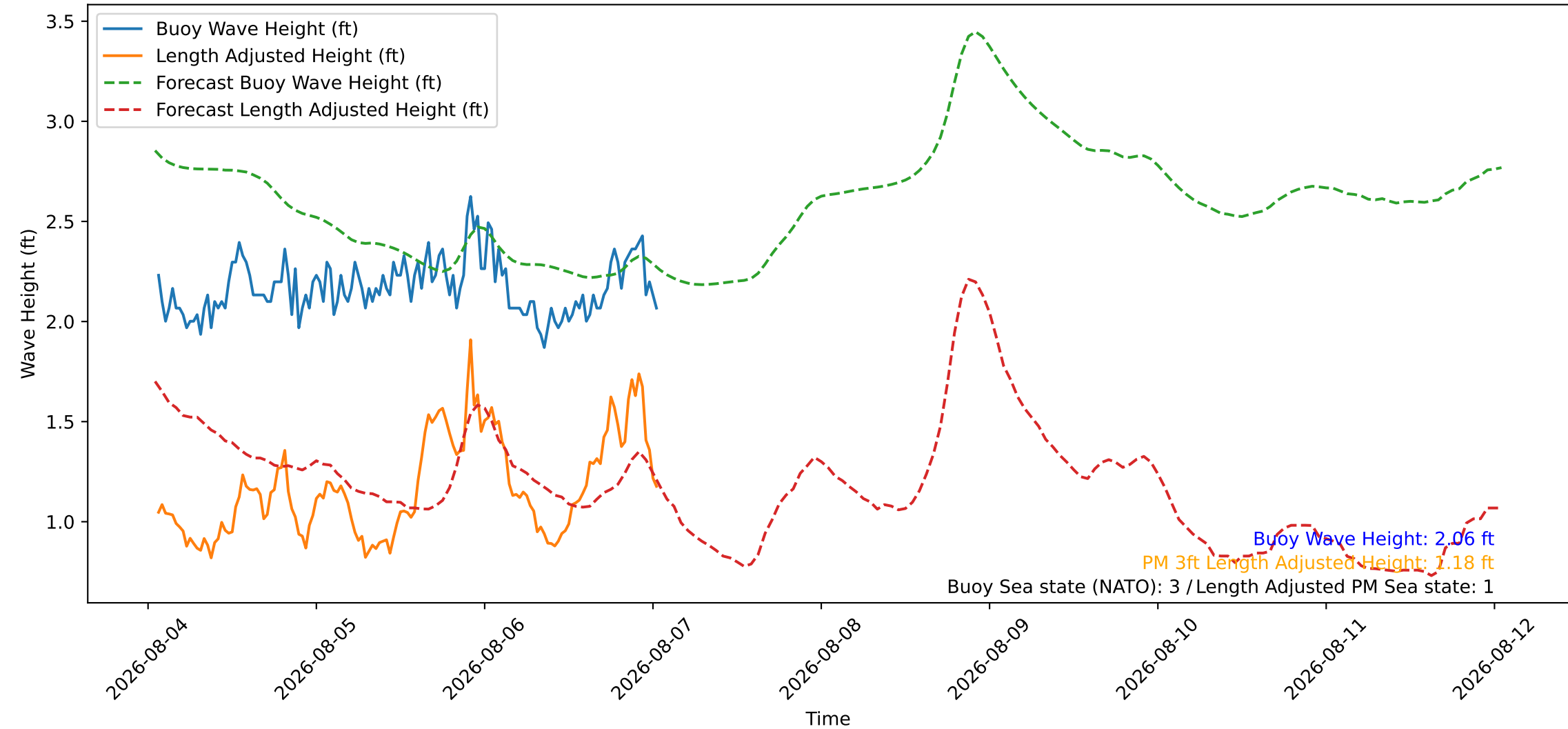
Wave Heights over Time for Green Beach at 2026-08-07 01:21:09
