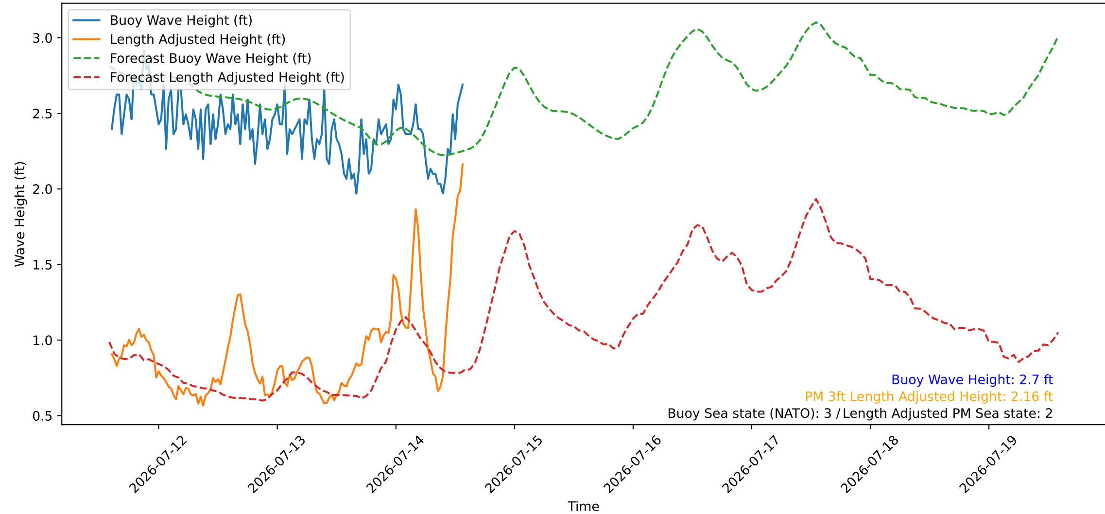
Wave Heights over Time for Red Beach at 2026-07-14 14:10:47
