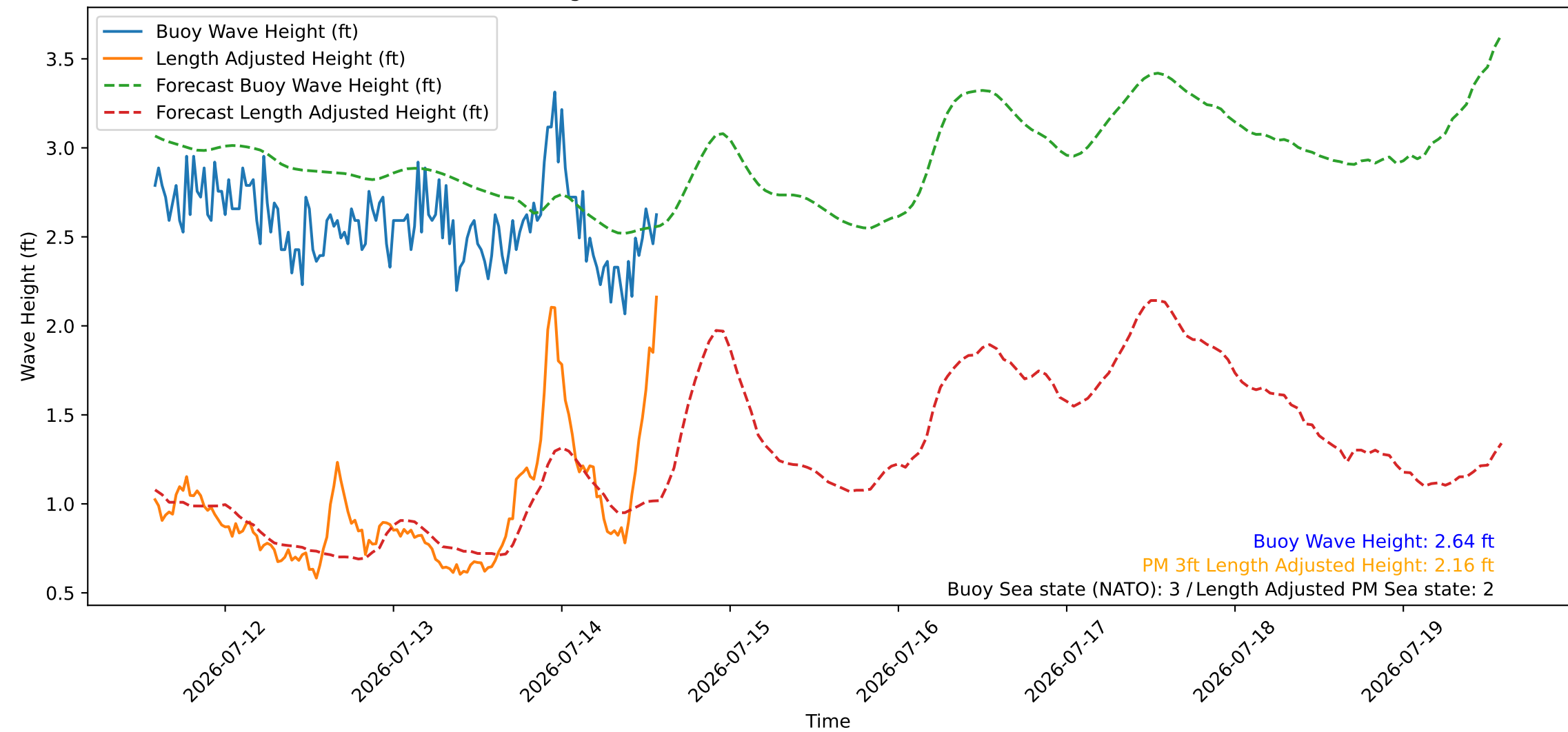
Wave Heights over Time for Green Beach at 2026-07-14 14:11:09
