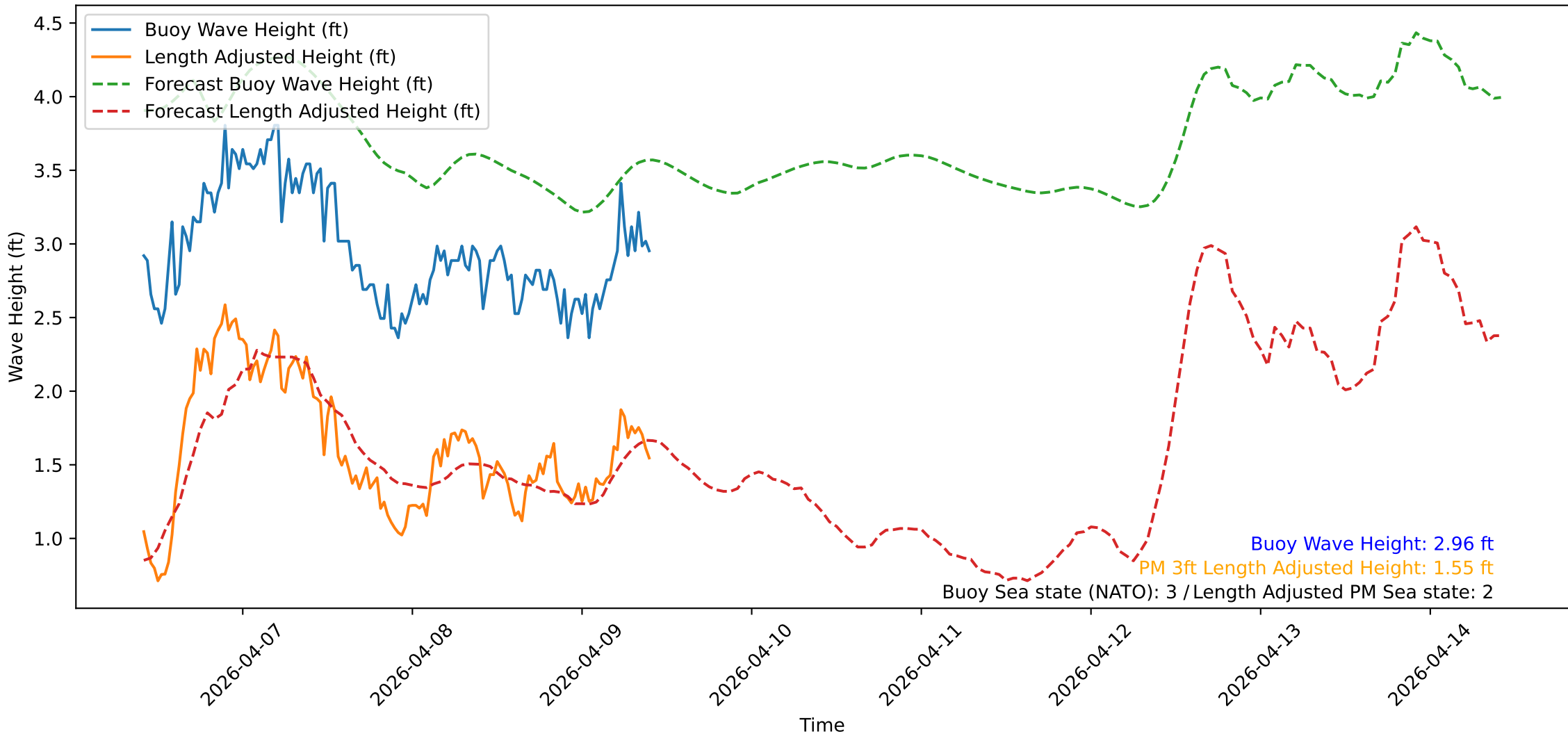
Wave Heights over Time for Green Beach at 2026-04-09 10:11:10
