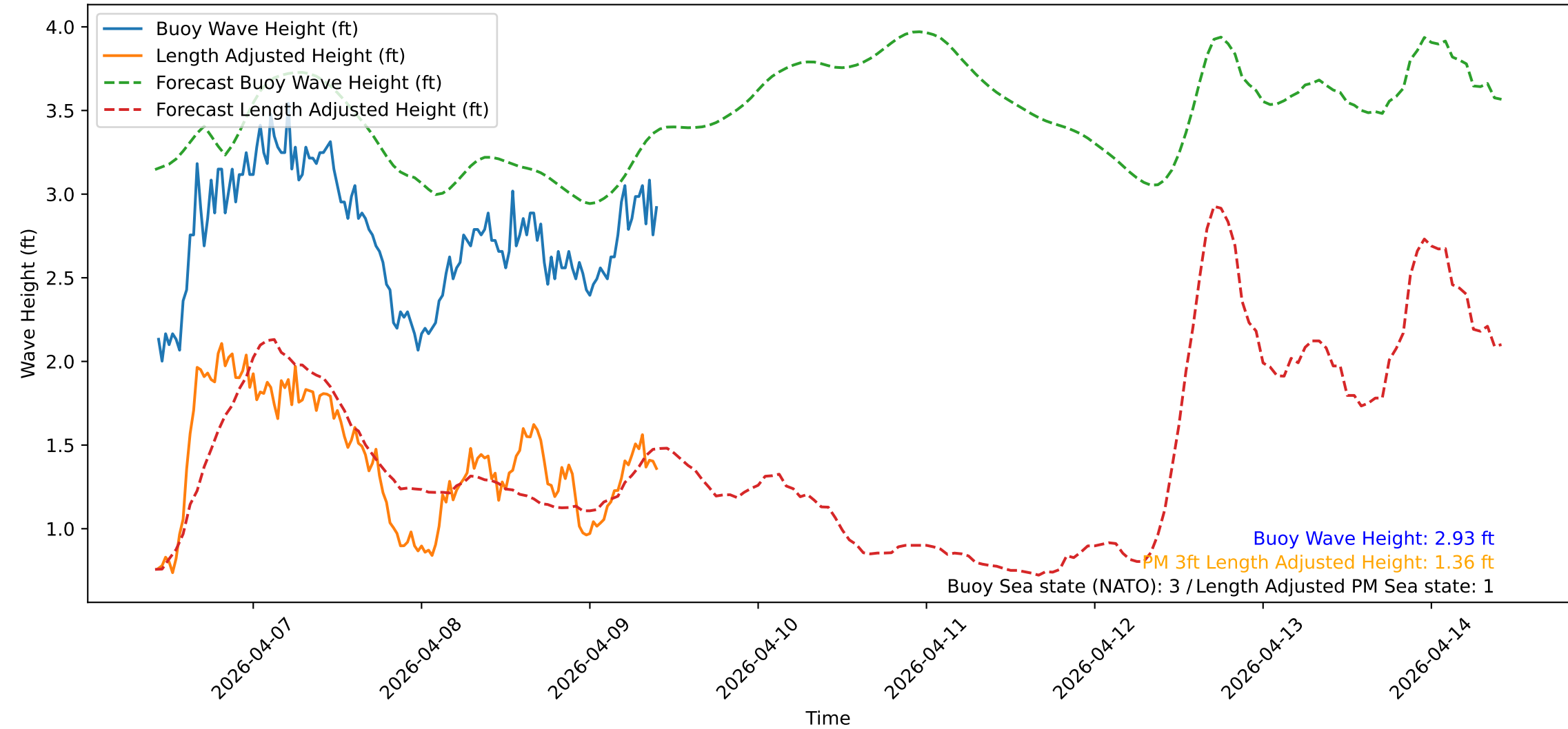
Wave Heights over Time for Red Beach at 2026-04-09 10:10:47
