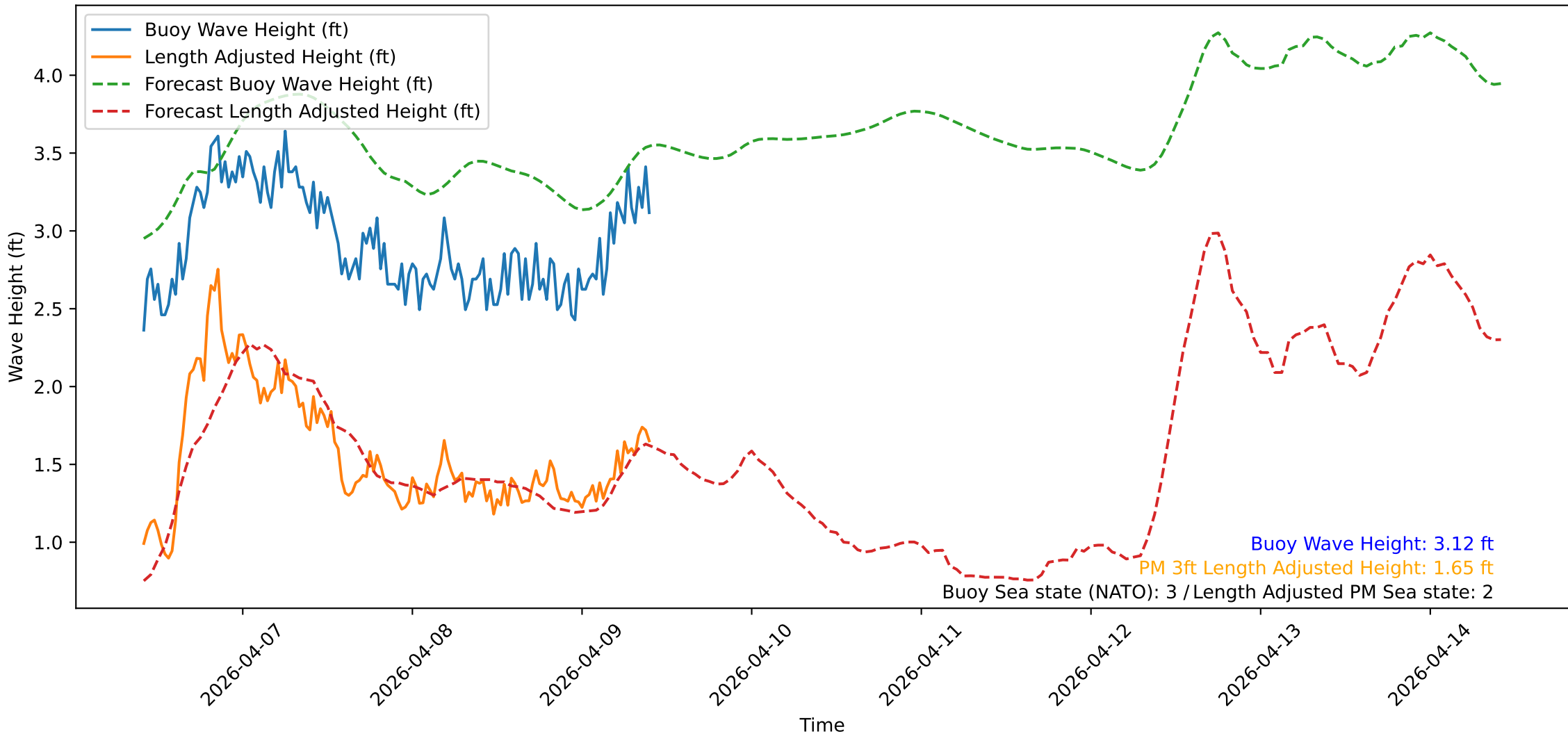
Wave Heights over Time for Oceanside Harbor at 2026-04-09 10:10:31
